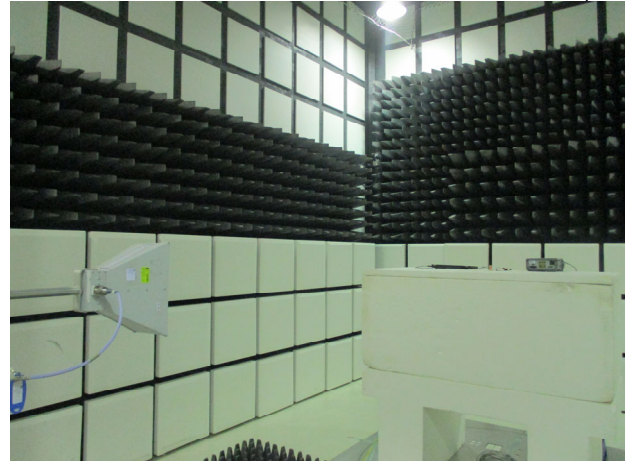
FCC_15_247_BLE_Radiated_ASC_RFANT3216120A5T_Setup
