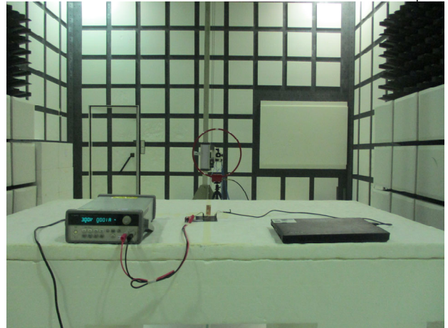
FCC_15_247_BLE_Radiated_ASC_RFANT3216120A5T_Setup
