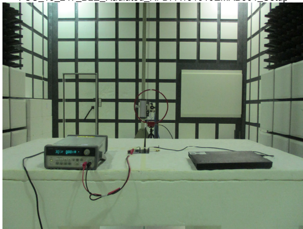
FCC_15_247_BLE_Radiated_ABR-ANT-DF01_Setup
