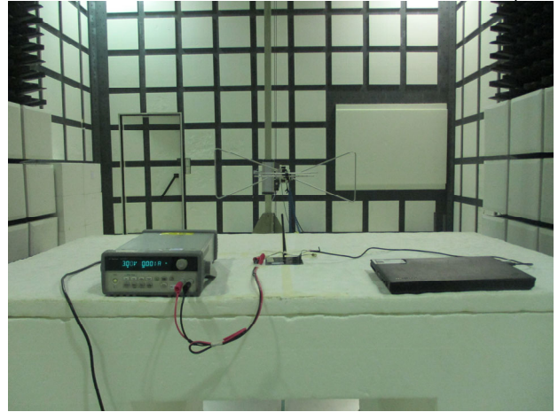
FCC_15_247_BLE_Radiated_ABR-ANT-DF01_Setup
