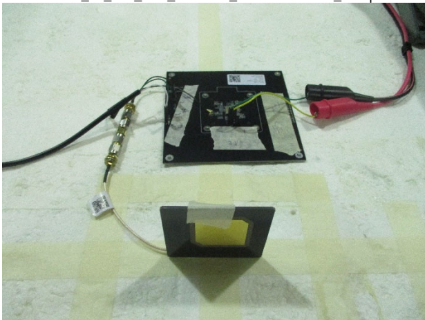
FCC_15_247_BLE_Radiated_ASC_RFANT3216120A5T_Setup
