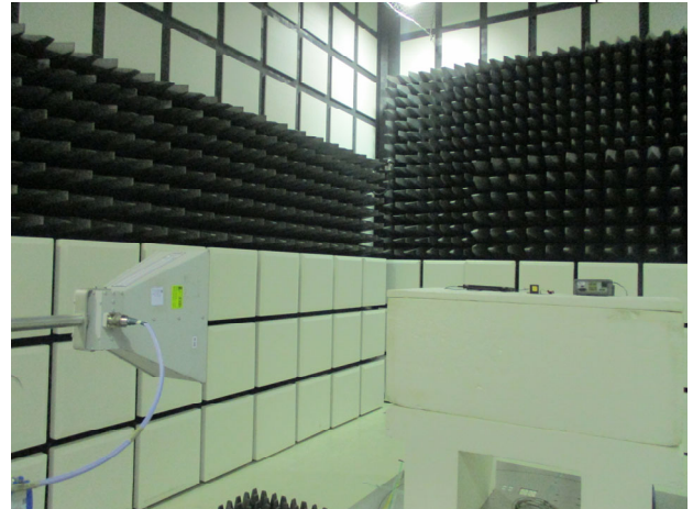
FCC_15_247_BLE_Radiated_ASC_RFANT3216120A5T_Setup
