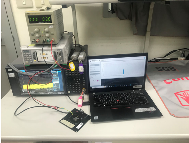
FCC_15_247_BLE_Radiated_ABR-ANT-DF01_Setup
