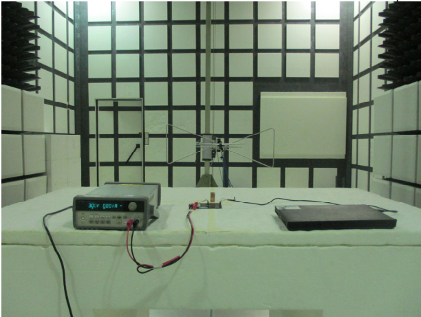
FCC_15_247_BLE_Radiated_ASC_RFANT3216120A5T_Setup
