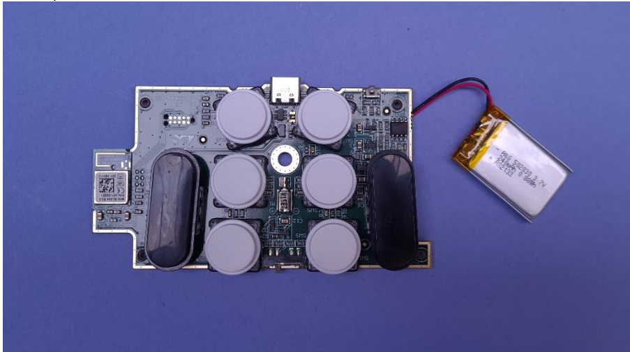
PCB bottom view
