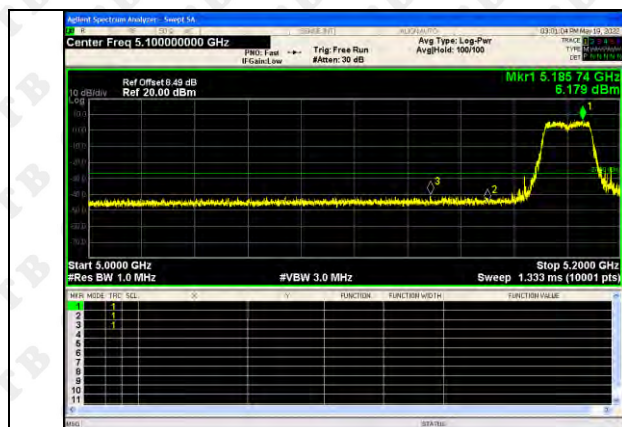
802.11n(HT40)-5190
