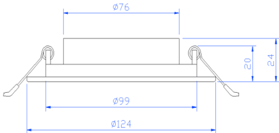
Hole cut:4"(102mm)
