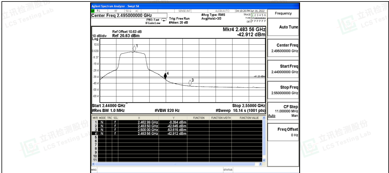
11G_Ant1_High_2462_Peak
