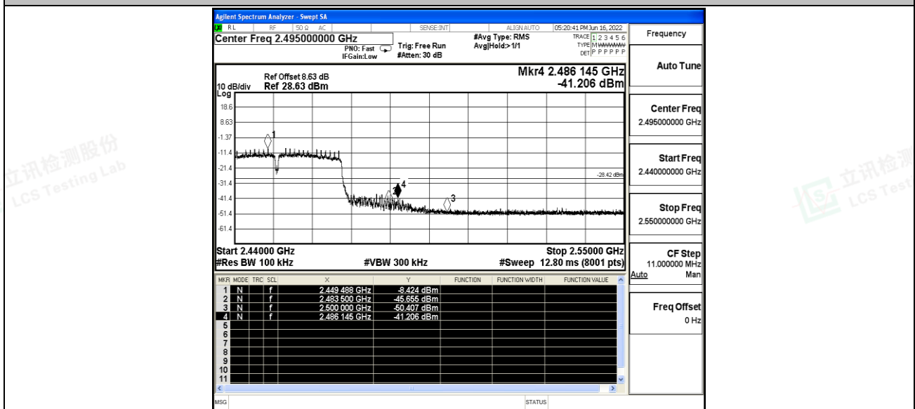
11N40SISO_Ant_High_2452
