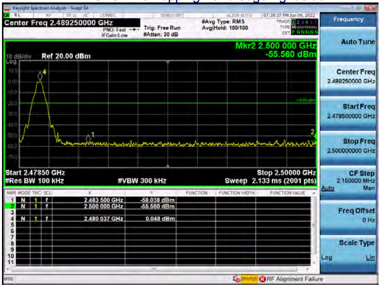
GFSK No-hopping Band edge-right side
