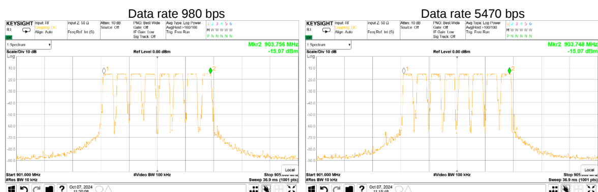
Plot 7.3.1 Number of hopping frequencies
