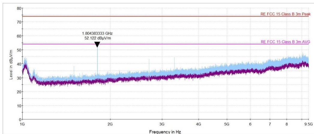
Plot 7.7.8 Radiated emission measurements from 1000 to 9500 MHz at the mid carrier frequency
