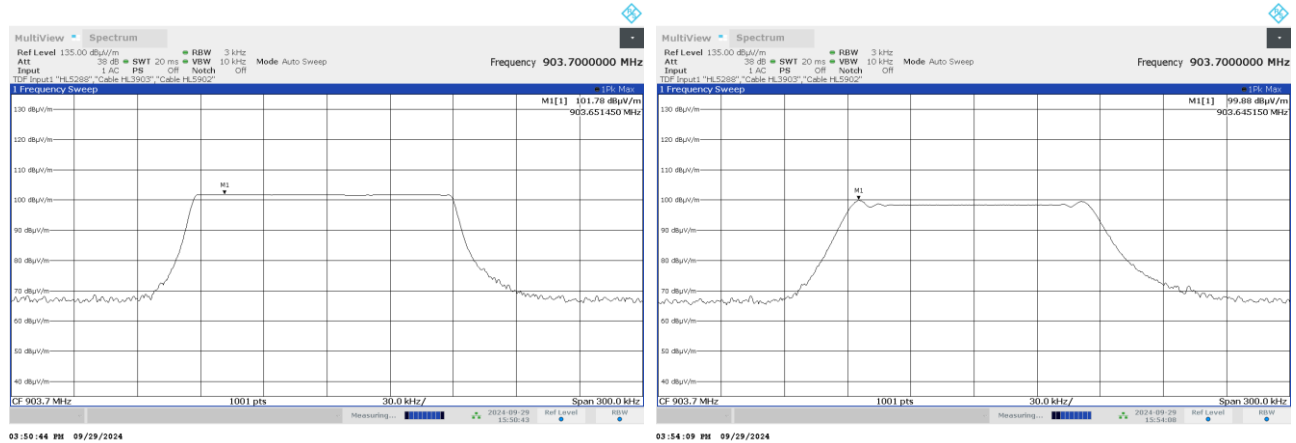
Plot 7.6.4 Peak spectral power density at low frequency (POLYMER)
