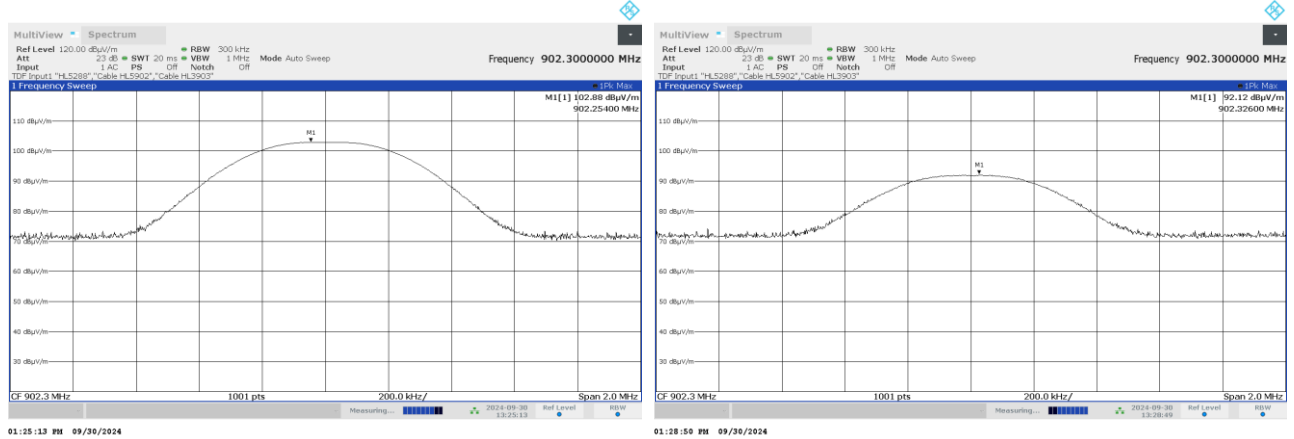
Plot 7.5.1 Field strength of carrier at low frequency (BRASS)
