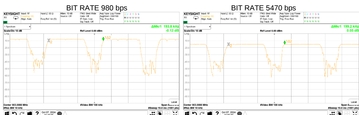
Plot 7.2.1 Carrier frequency separation
