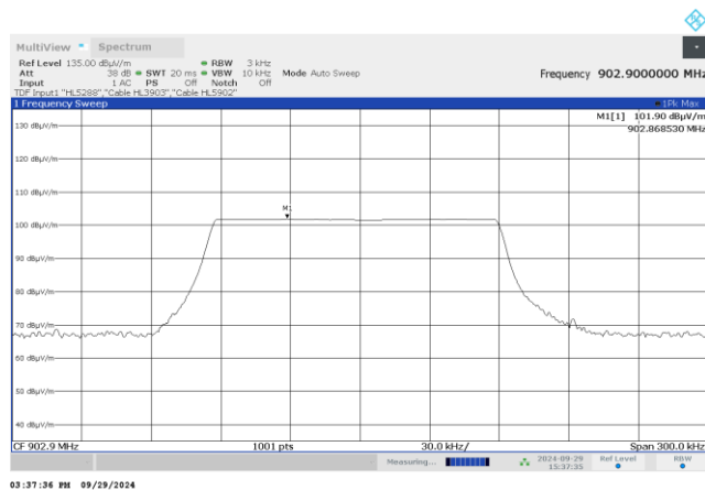
Plot 7.6.2 Peak spectral power density at mid frequency ( BRASS)
