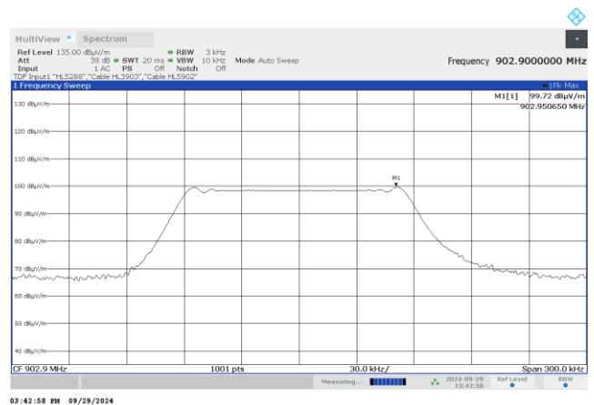
Plot 7.6.2 Peak spectral power density at mid frequency ( BRASS)
