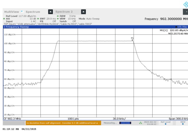
Plot 7.6.2 Peak spectral power density at mid frequency
