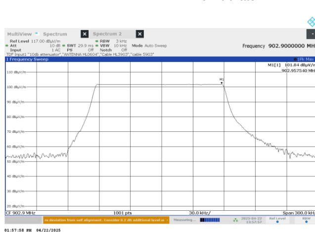
Plot 7.6.2 Peak spectral power density at mid frequency
