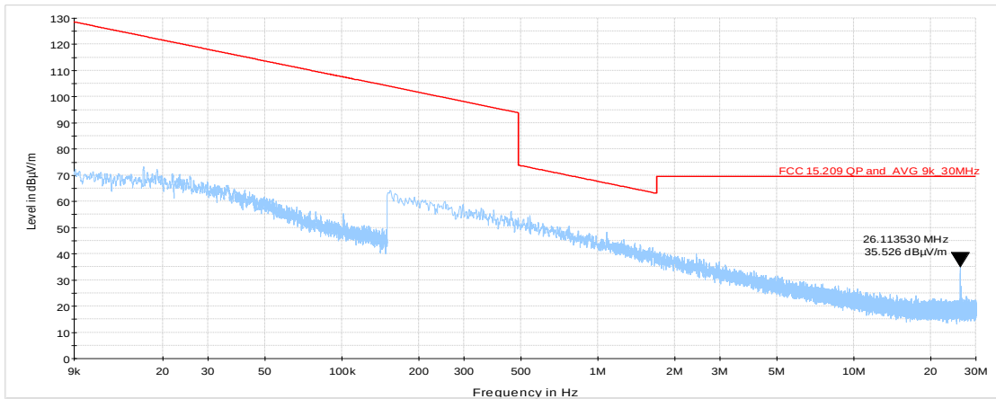
Plot 7.7.5 Radiated emission measurements from 0.009 to 30 MHz at the mid carrier frequency
