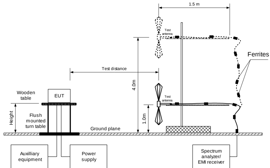
Figure 7.7.2 Setup for spurious emission field strength measurements from 30 to 1000 MHz
