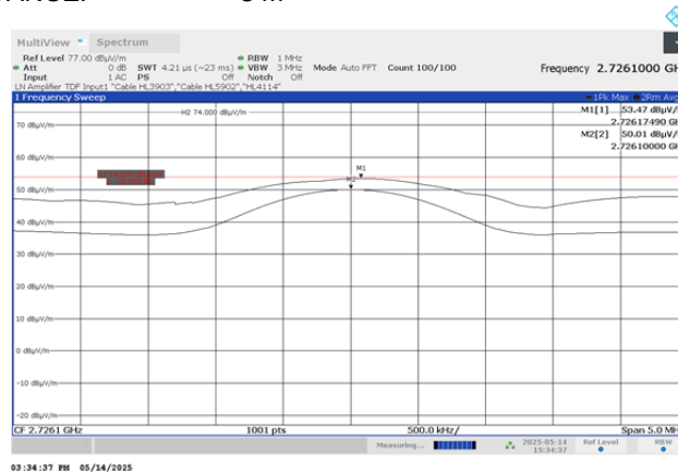
Plot 7.7.15 Radiated emission measurements at the third harmonic of high carrier frequency
