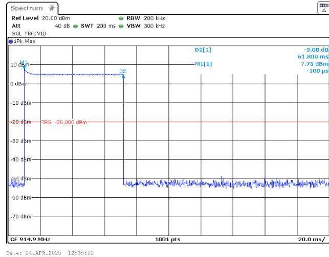
Plot 7.7.16 Transmission pulse duration
