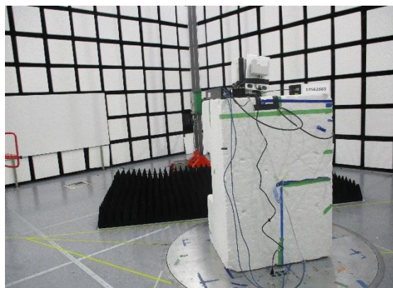
BACK PHOTO(Directional antenna with Tripod)
