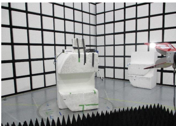
FRONT PHOTO (Directional antenna with Tripod)
