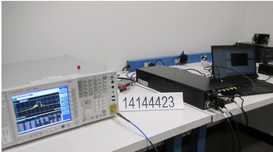
FREQUENCY TOLERANCE OVER EXTREME CONDITIONS
