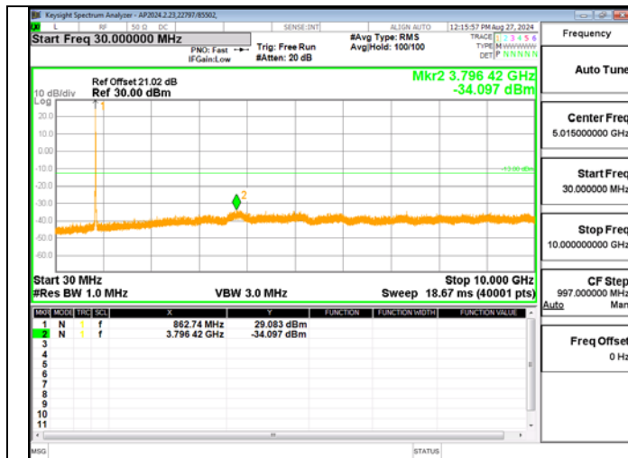
LTE BAND 26(90S) QPSK 5M RB25-0 Mid Ch – BTS 2
