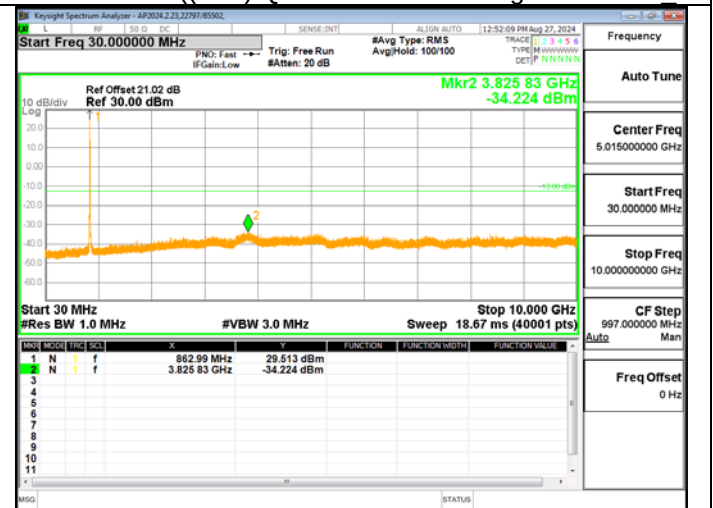
LTE BAND 26(90S) QPSK 5M RB25-0 Mid Ch – BTS 3
