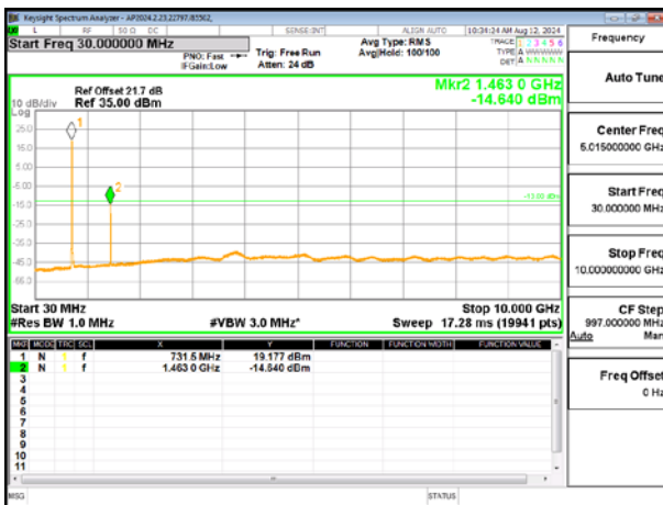
LTE BAND 12 QPSK 5M RB25-0 Low Ch – BTS_3
