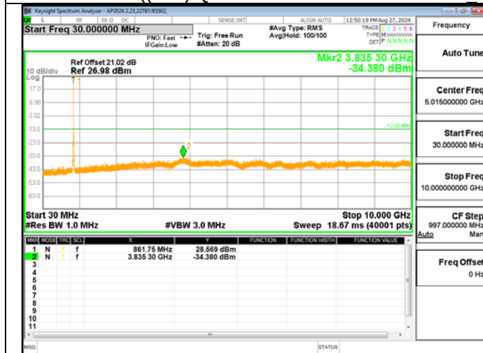
LTE BAND 26(90S) QPSK 5M RB25-0 Low Ch – BTS 3
