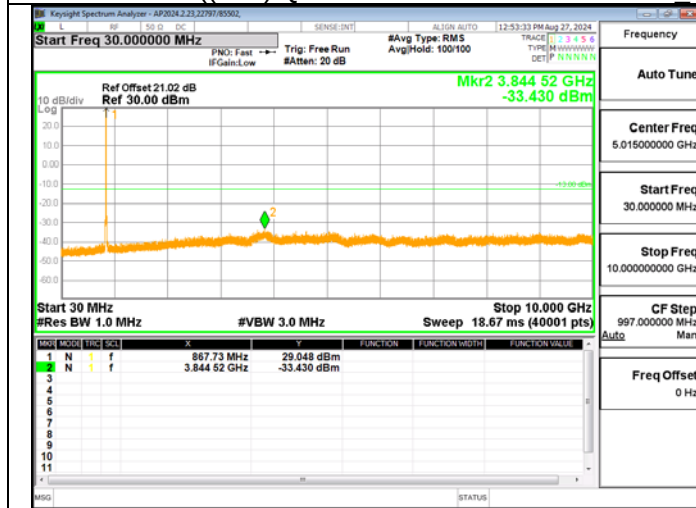
LTE BAND 26(90S) QPSK 5M RB25-0 High Ch – BTS 3
