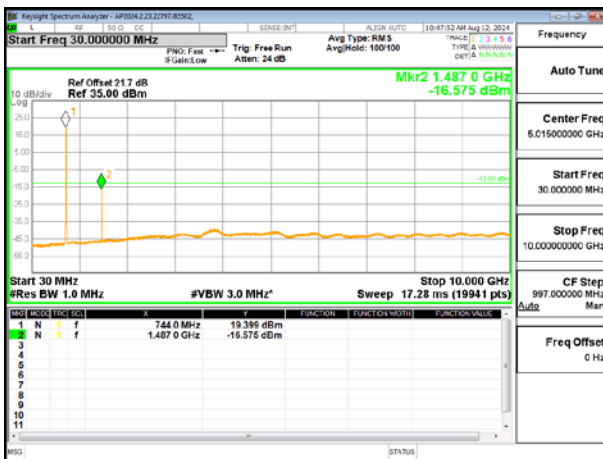
LTE BAND 12 QPSK 5M RB25-0 High Ch – BTS_3
