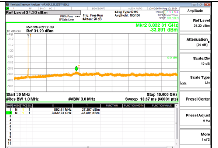
LTE BAND 26(22H) QPSK 5M RB25-0 High Ch – BTS_2
