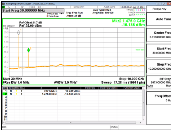
LTE BAND 12 QPSK 5M RB25-0 Mid Ch – BTS_2
