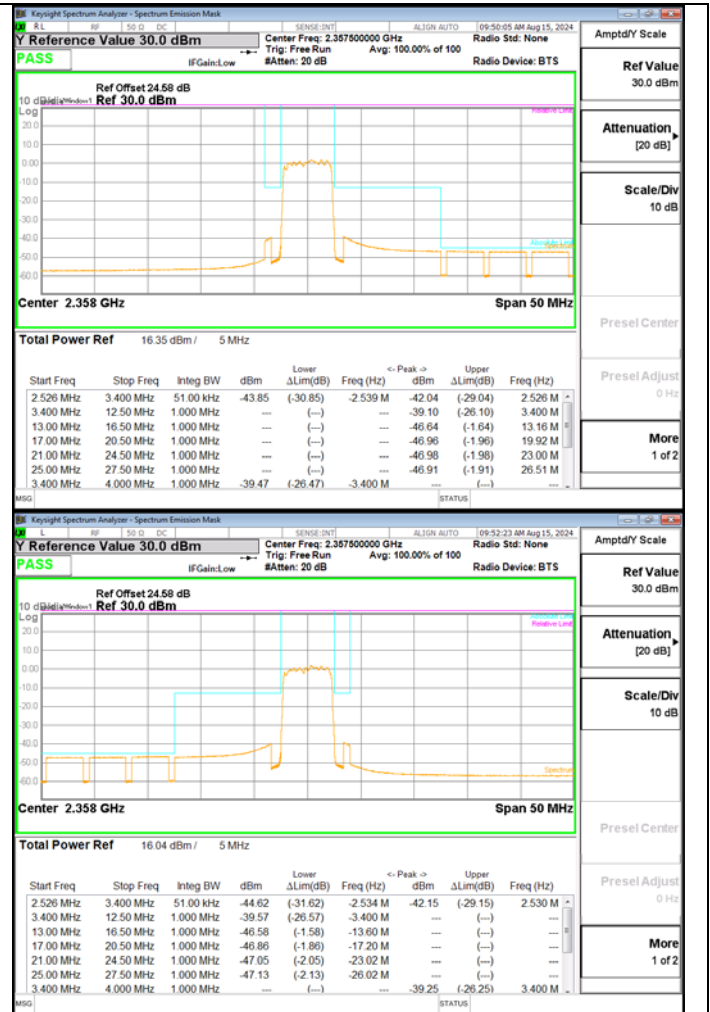
LTE BAND 30 QPSK 5M RB25-0 High Ch – BTS_1
