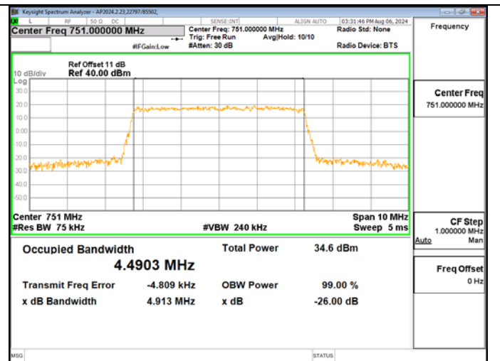
LTE Band 13 QPSK Mid Channel
