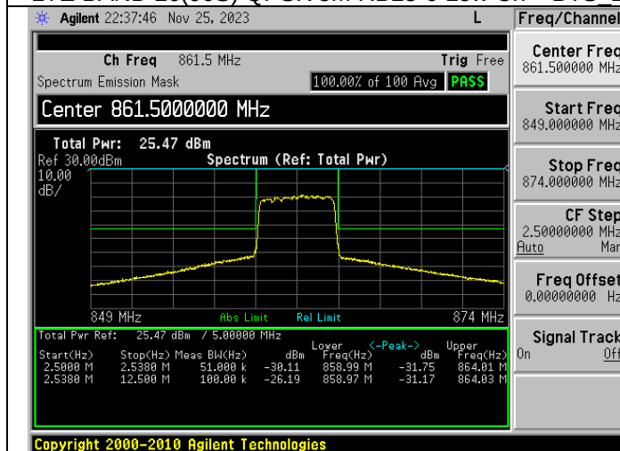
LTE BAND 26(90S) QPSK 5M RB25-0 Low Ch – BTS 2
