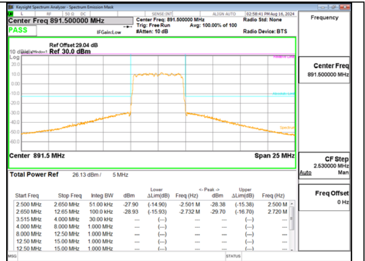
LTE BAND 26(22H) QPSK 5M RB25-0 High Ch – BTS 1
