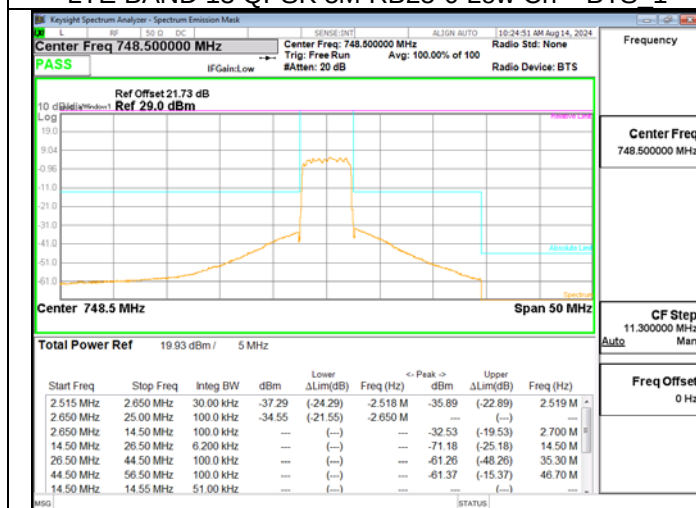
LTE BAND 13 QPSK 5M RB25-0 Low Ch – BTS 2
