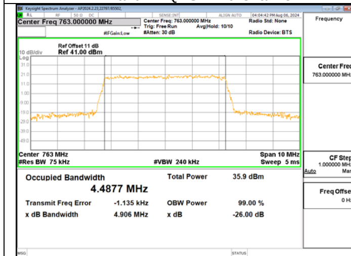
LTE Band 14 QPSK Mid Channel
