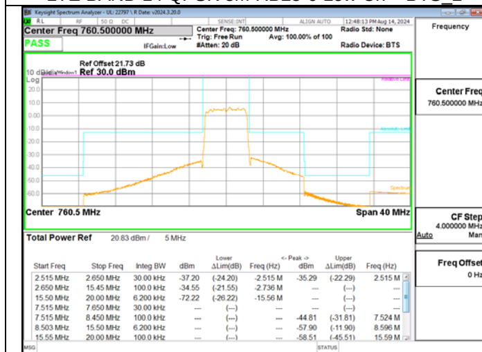
LTE BAND 14 QPSK 5M RB25-0 Low Ch – BTS 3
