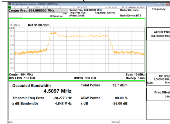
5G NR n26 (90S) QPSK Mid Channel
