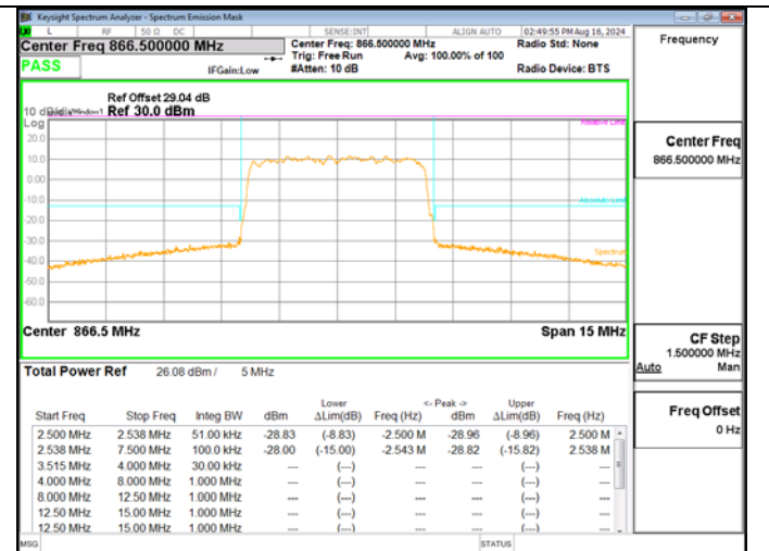
LTE BAND 26(90S) QPSK 5M RB25-0 High Ch – BTS 1
