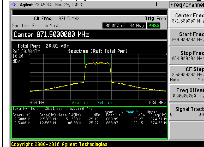
LTE BAND 26(22H) QPSK 5M RB25-0 Low Ch – BTS 3
