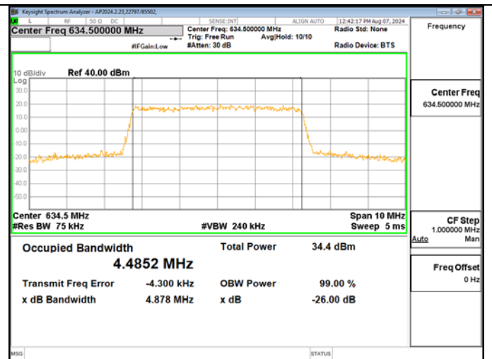
LTE Band 71 QPSK Mid Channel
