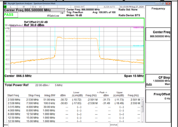
5G NR N26(90S) QPSK 5M RB25-0 High Ch – BTS_3
