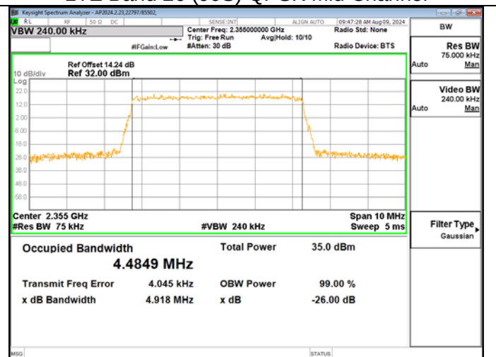
LTE Band 30 QPSK Mid Channel
