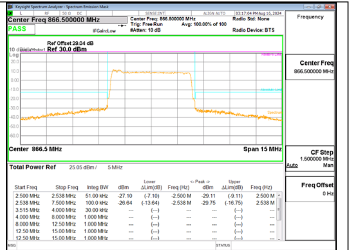
5G NR N26(90S) QPSK 5M RB25-0 High Ch – BTS_1
