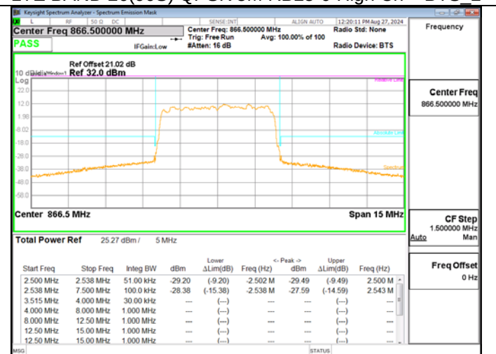
LTE BAND 26(90S) QPSK 5M RB25-0 High Ch – BTS 3
