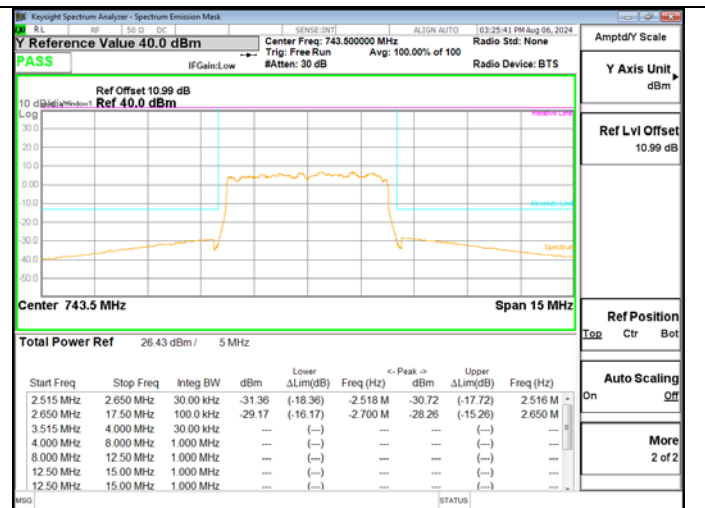
LTE BAND 12 QPSK 5M RB25-0 High Ch – BTS 1
