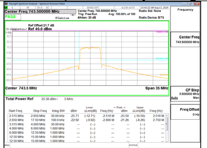
LTE BAND 12 QPSK 5M RB25-0 High Ch – BTS 2
