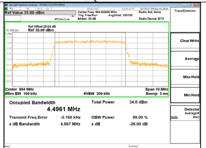
LTE Band 26 (90S) QPSK Mid Channel
