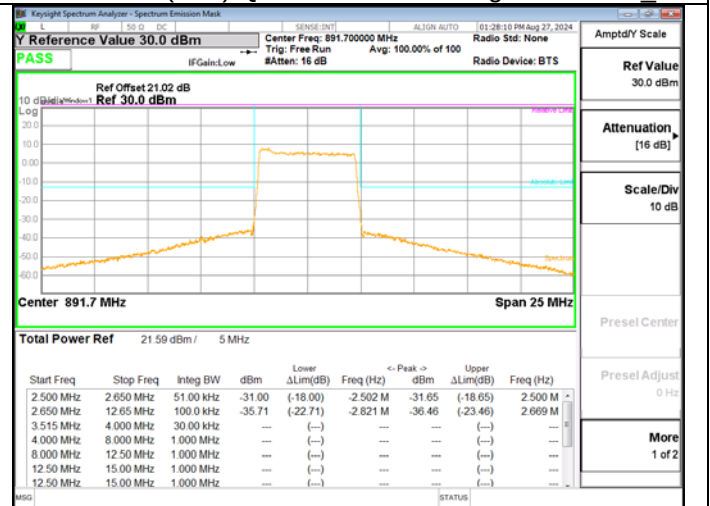
5G NR BAND n26 QPSK 5M RB25-0 High Ch – BTS 3
