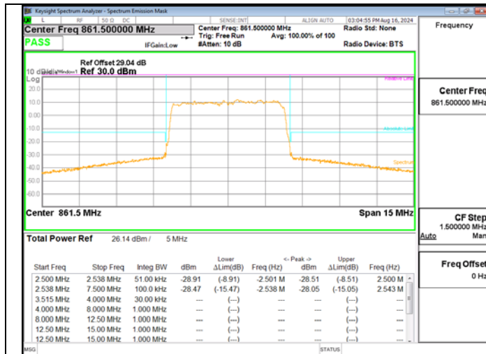
LTE BAND 26(90S) QPSK 5M RB25-0 Low Ch – BTS 1
