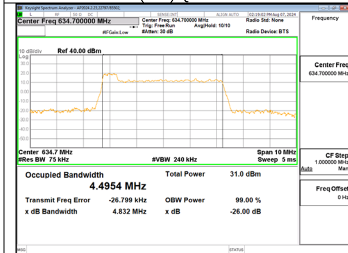
5G NR n71 QPSK Mid Channel
