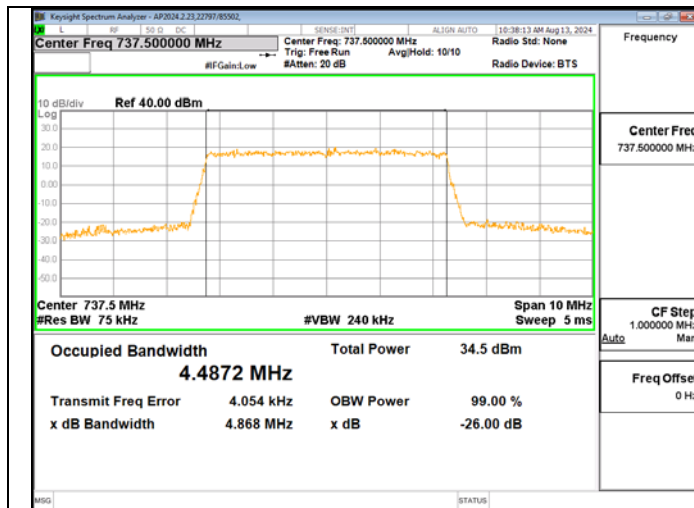
LTE Band 12 QPSK Mid Channel
