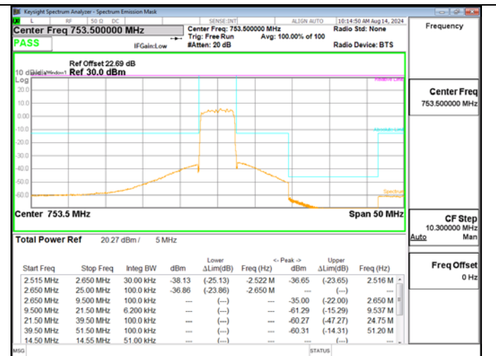
LTE BAND 13 QPSK 5M RB25-0 High Ch – BTS 1
