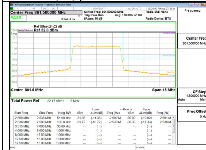
5G NR N26(90S) QPSK 5M RB25-0 Low Ch – BTS_2
