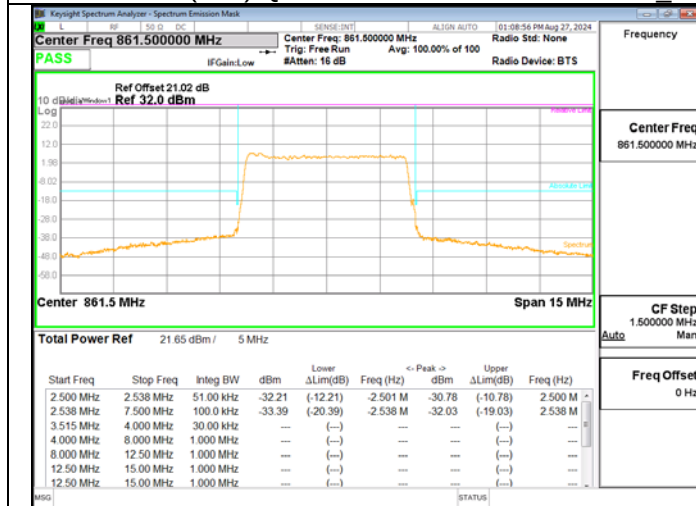
5G NR N26(90S) QPSK 5M RB25-0 Low Ch – BTS_3
