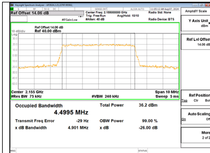
LTE Band 66 QPSK Mid Channel
