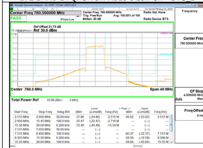
LTE BAND 14 QPSK 5M RB25-0 Low Ch – BTS 2
