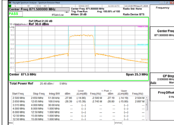
LTE BAND 26(22H) QPSK 5M RB25-0 Low Ch – BTS 2
