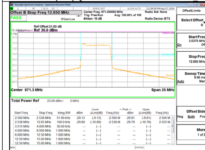
5G NR BAND n26 QPSK 5M RB25-0 Low Ch – BTS 2
