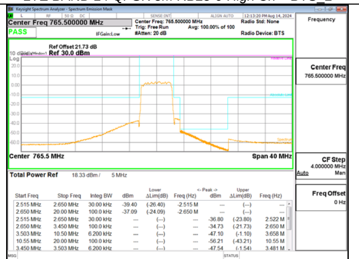
LTE BAND 14 QPSK 5M RB25-0 High Ch – BTS 3
