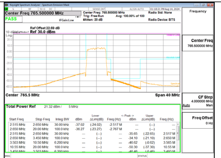
LTE BAND 14 QPSK 5M RB25-0 High Ch – BTS 1
