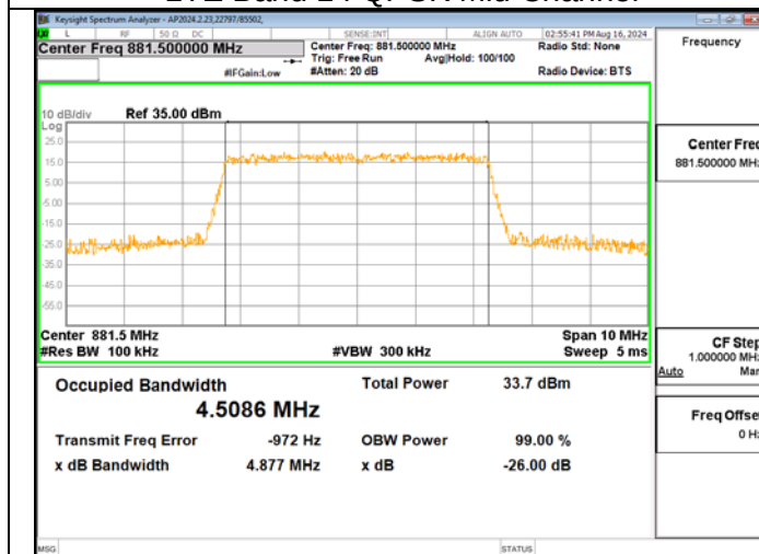
LTE Band 26 (22H) QPSK Mid Channel
