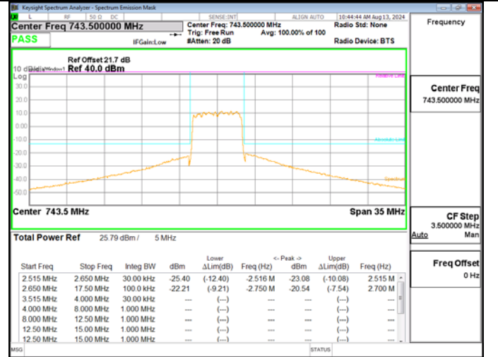
LTE BAND 12 QPSK 5M RB25-0 High Ch – BTS 3
