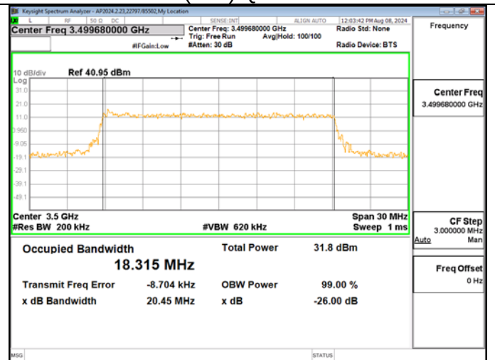
5G NR n77 (3450 - 3550) QPSK Mid Channel
