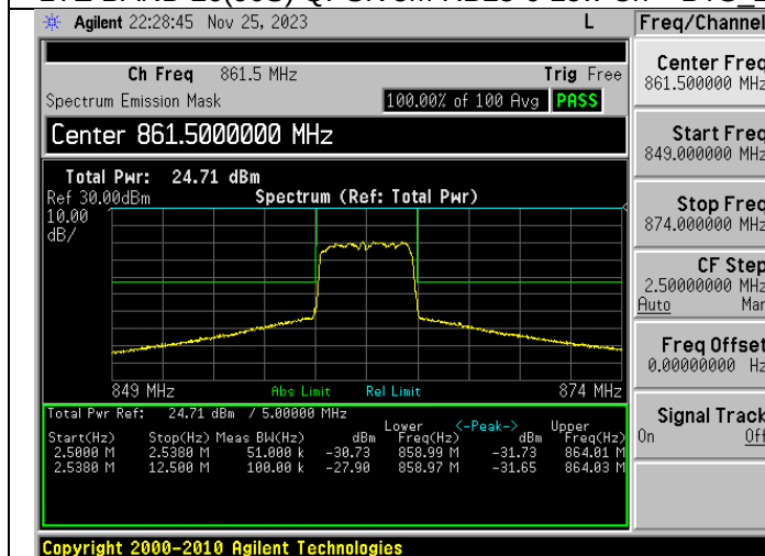
LTE BAND 26 (90S) QPSK 5M RB25 Low Ch – BTS 3
