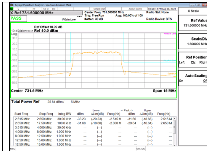
LTE BAND 12 QPSK 5M RB25-0 Low Ch – BTS 1
