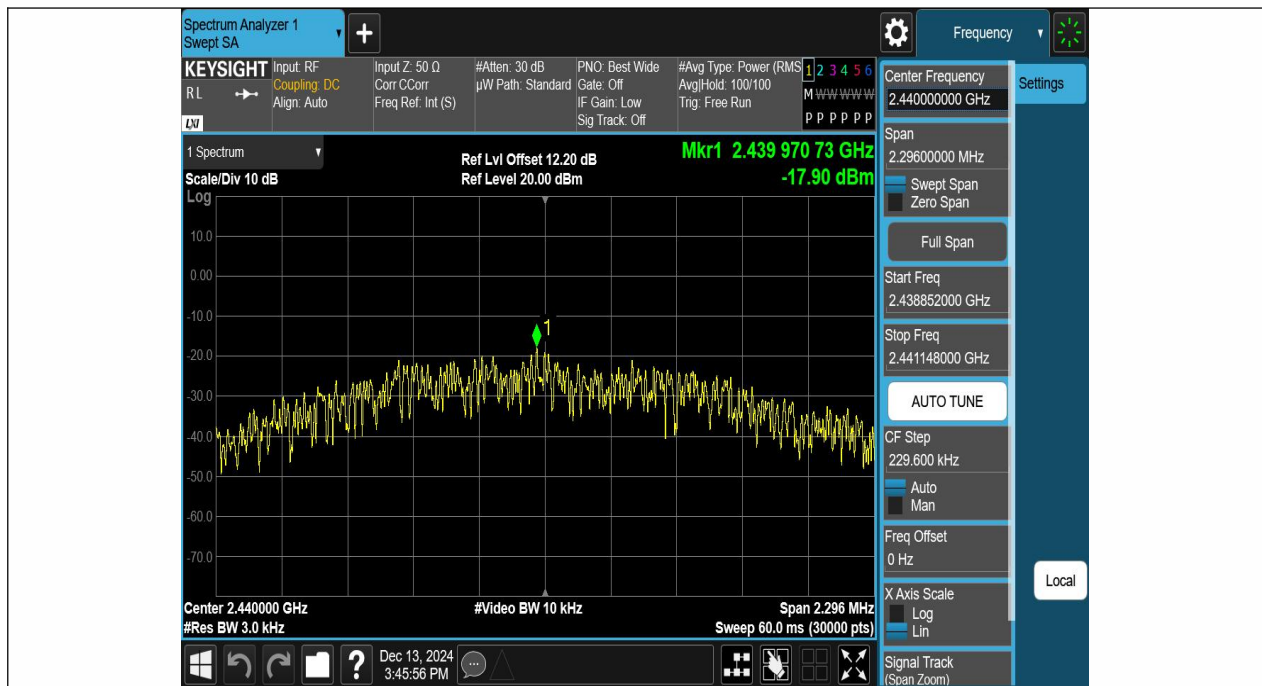
BLE_2M-Ant1-2440-PASS
