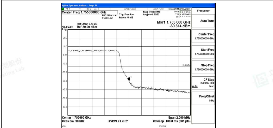
Band4-3MHz-QPSK-19965-15RB#0
