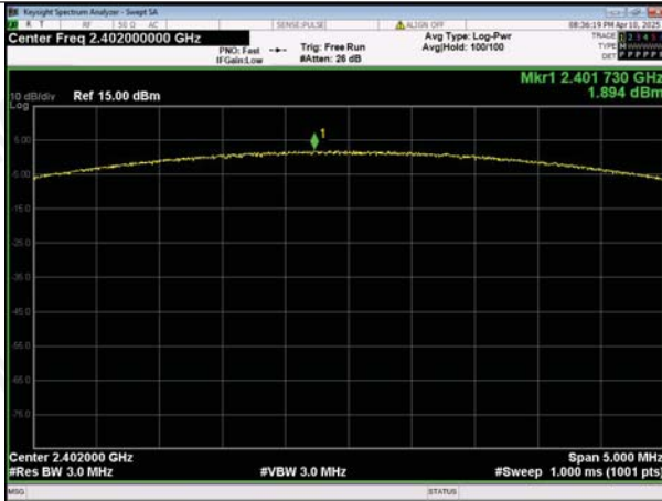
Peak Output Power 8DPSK_Channel 0
