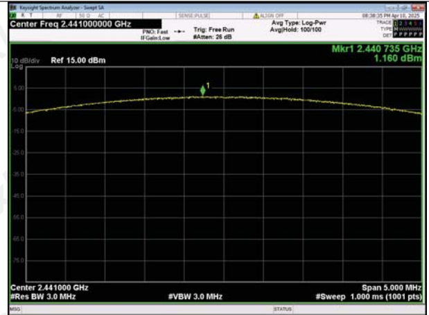
Peak Output Power 8DPSK_Channel 39
