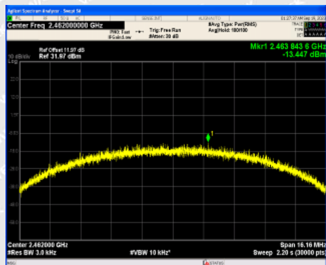
802.11b_High Channel
