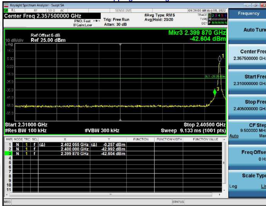
GFSK No-hopping Band edge-left side
