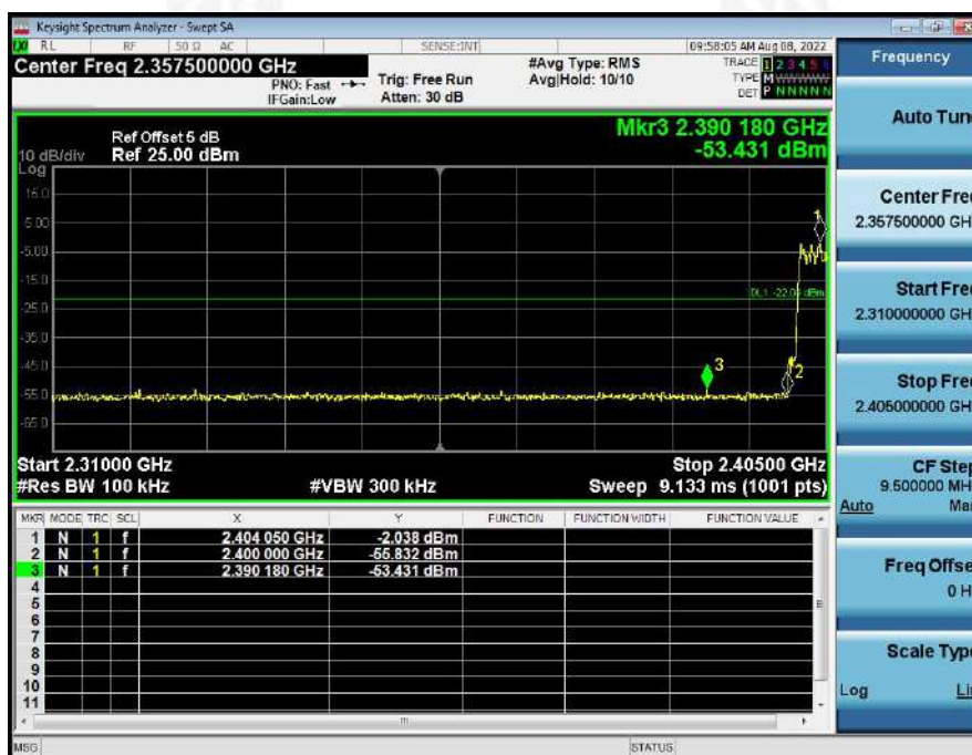
\pi/4 -DQPSK Hopping Band edge-left side
