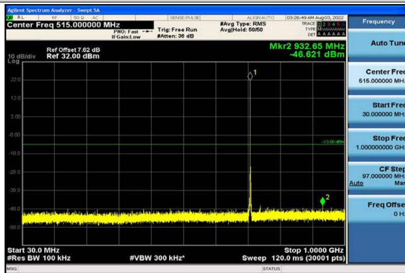
Band12-1.4MHz-16QAM-23173-1RB#0-30~1000MHz
