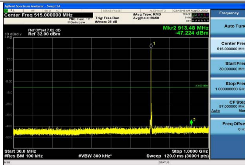
Band12-3MHz-16QAM-23165-1RB#0-30~1000MHz
