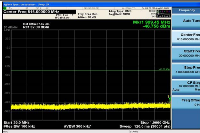
Band2-5MHz-QPSK-18900-1RB#0-30~1000MHz
