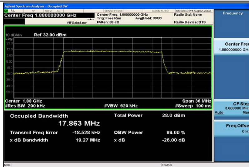
Band2-20MHz-QPSK-18900-100RB#0-17.863
