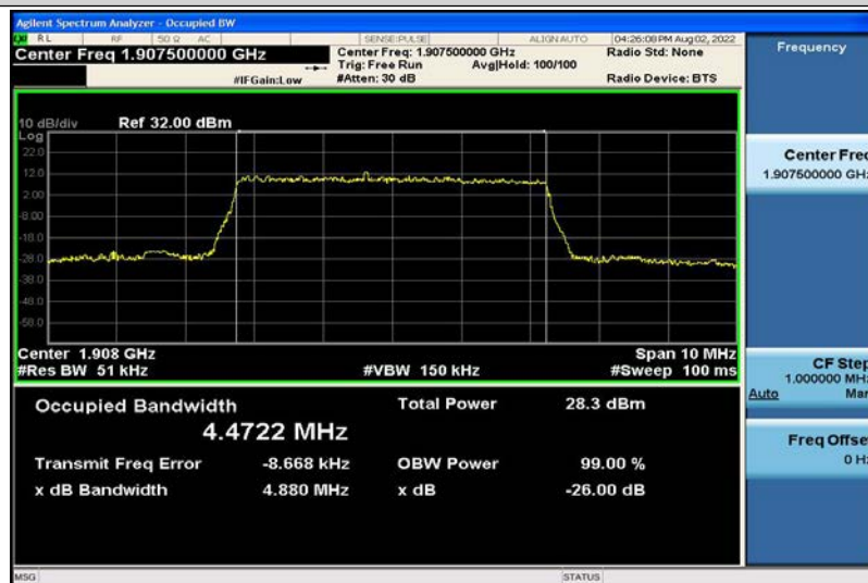
Band2-5MHz-16QAM-19175-25RB#0-4.4722
