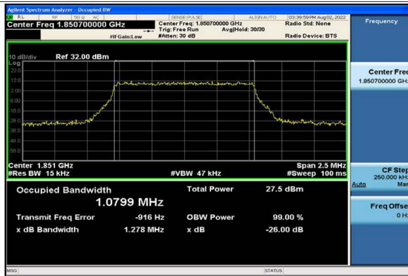
Band2-1.4MHz-QPSK-18607-6RB#0-1.0799
