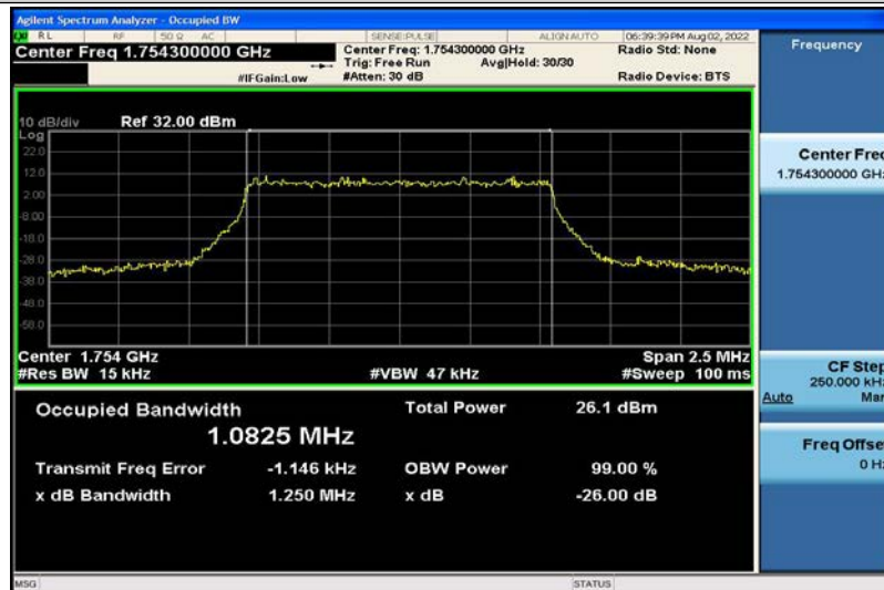
Band4-1.4MHz-16QAM-20393-6RB#0-1.0825
