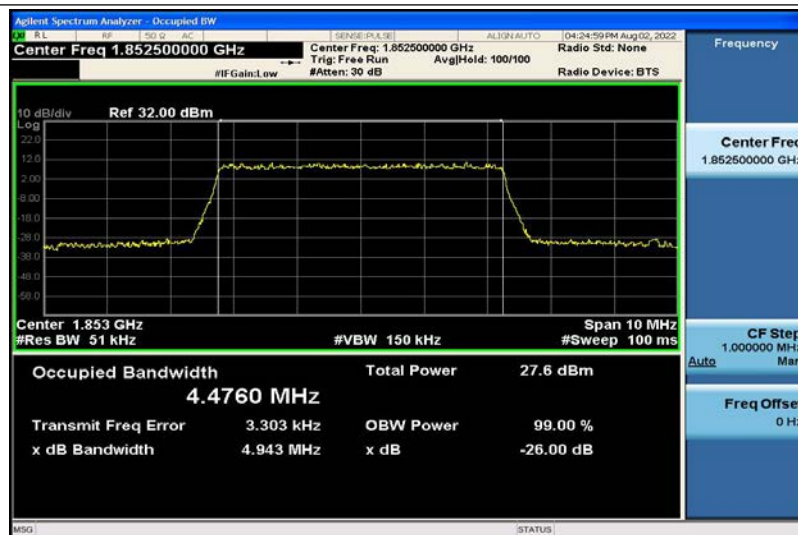
Band2-5MHz-16QAM-18625-25RB#0-4.4760
