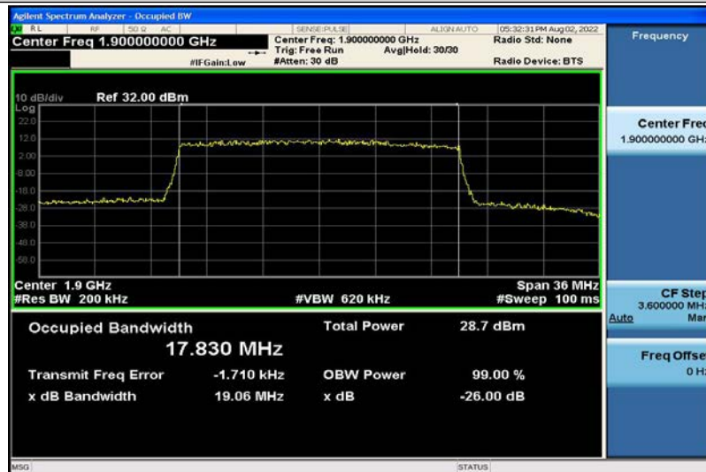
Band2-20MHz-QPSK-19100-100RB#0-17.830
