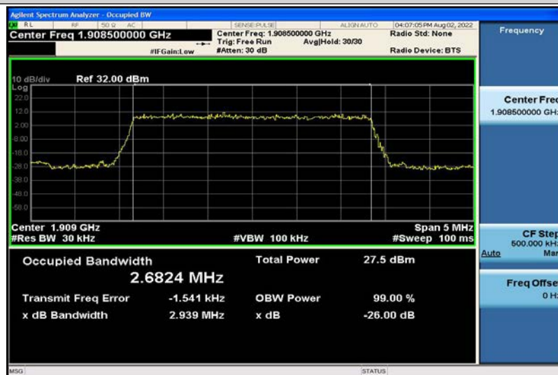
Band2-3MHz-16QAM-19185-15RB#0-2.6824
