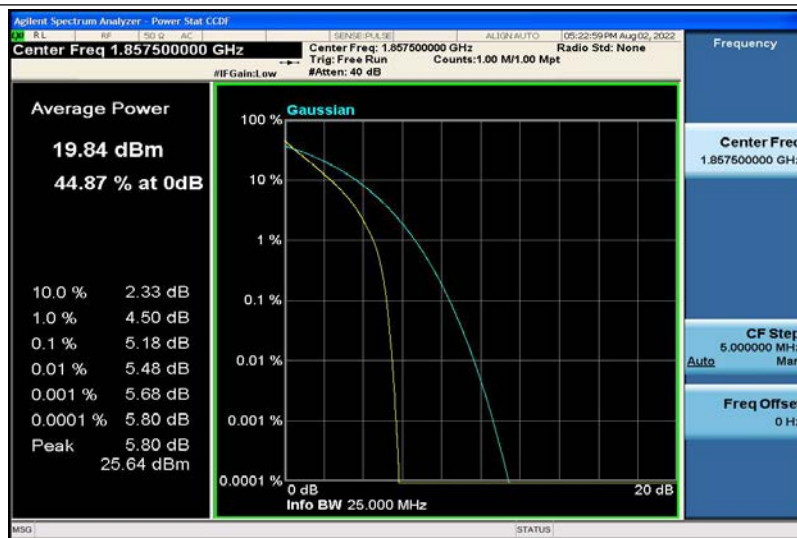
Band2-15MHz-QPSK-18675-1RB#0
