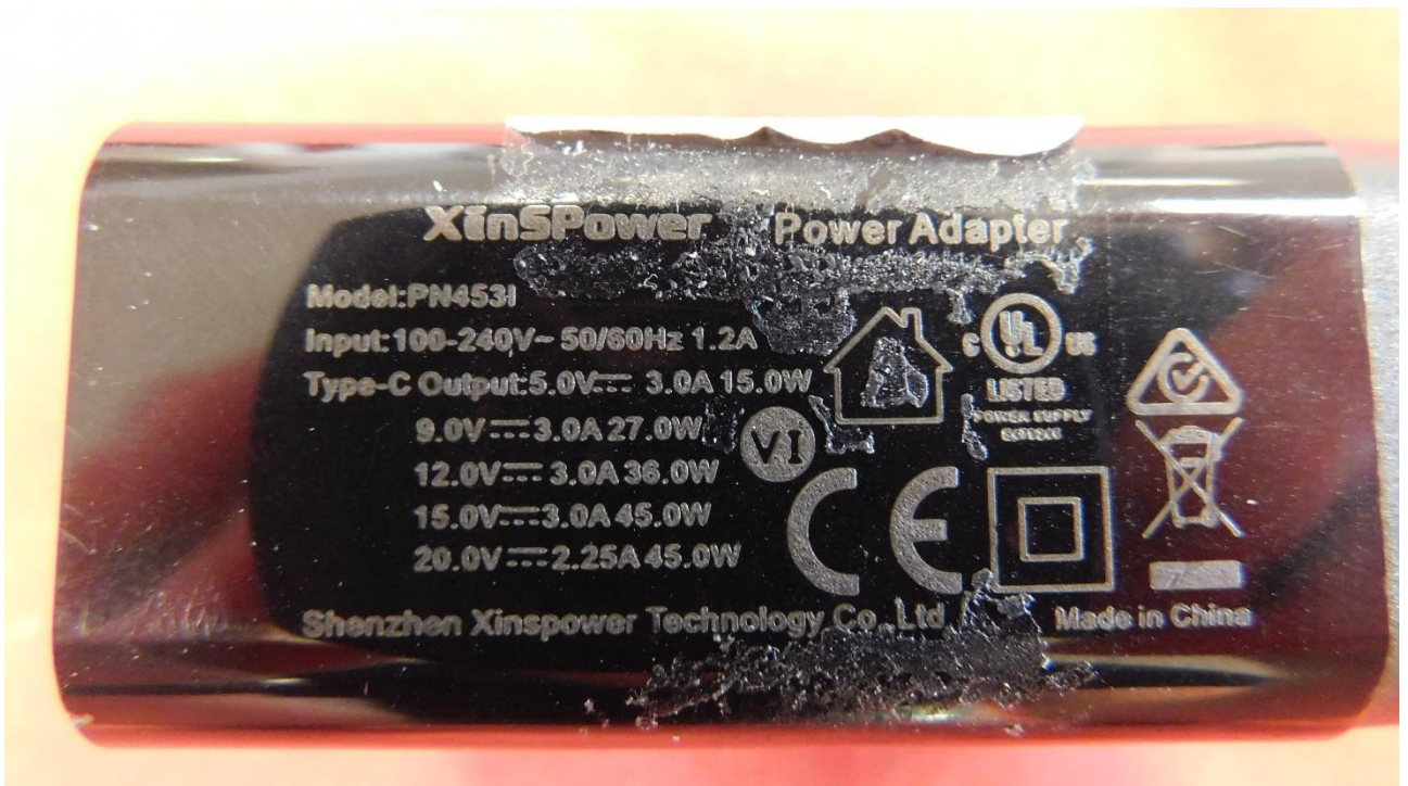
Picture 16: Name plate of power supply
