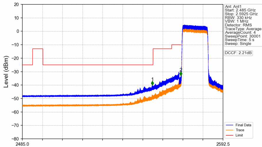
Band38_15MHz_16QAM_LCH_2577.5MHz_RB_75_0_NTNV
