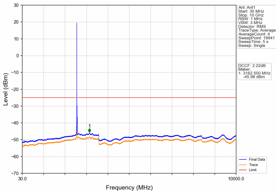
Band38_15MHz_16QAM_LCH_2577.5MHz_RB_1_0_NTNV
