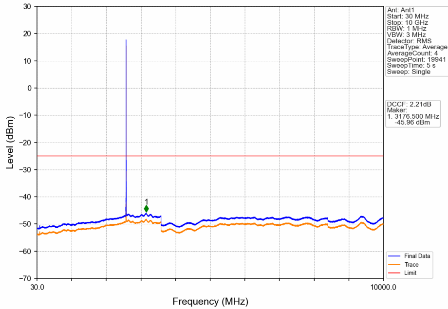
Band38_5MHz_16QAM_MCH_2595MHz_RB_1_0_NTNV
