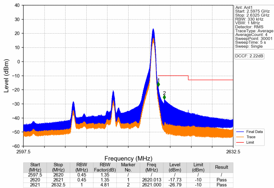
Band38_15MHz_QPSK_HCH_2612.5MHz_RB_1_74_NTNV
