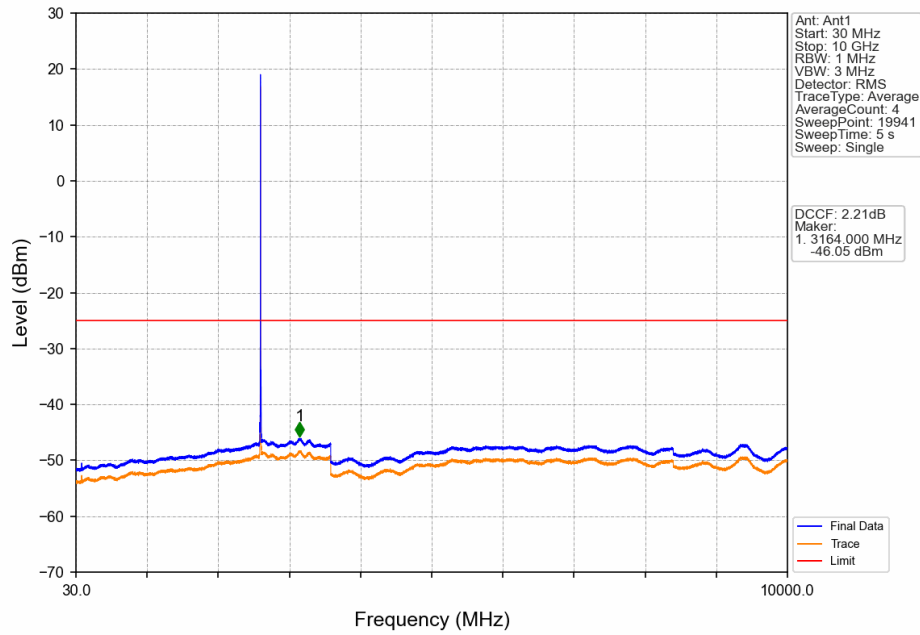
Band38_5MHz_QPSK_HCH_2617.5MHz_RB_1_0_NTNV
