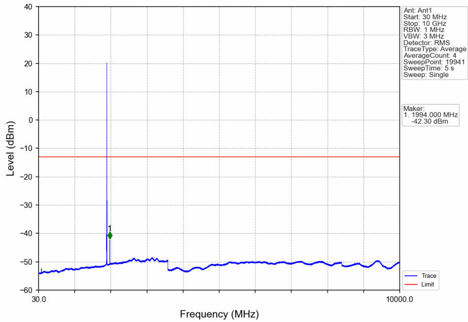
Band25_3MHz_QPSK_HCH_1913.5MHz_RB_1_0_NTNV
