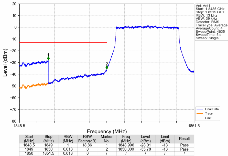
Band25_1.4MHz_16QAM_LCH_1850.7MHz_RB_6_0_NTNV
