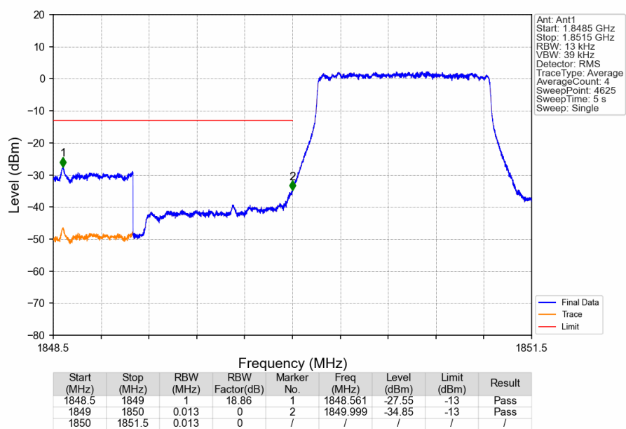
Band25_1.4MHz_QPSK_LCH_1850.7MHz_RB_6_0_NTNV
