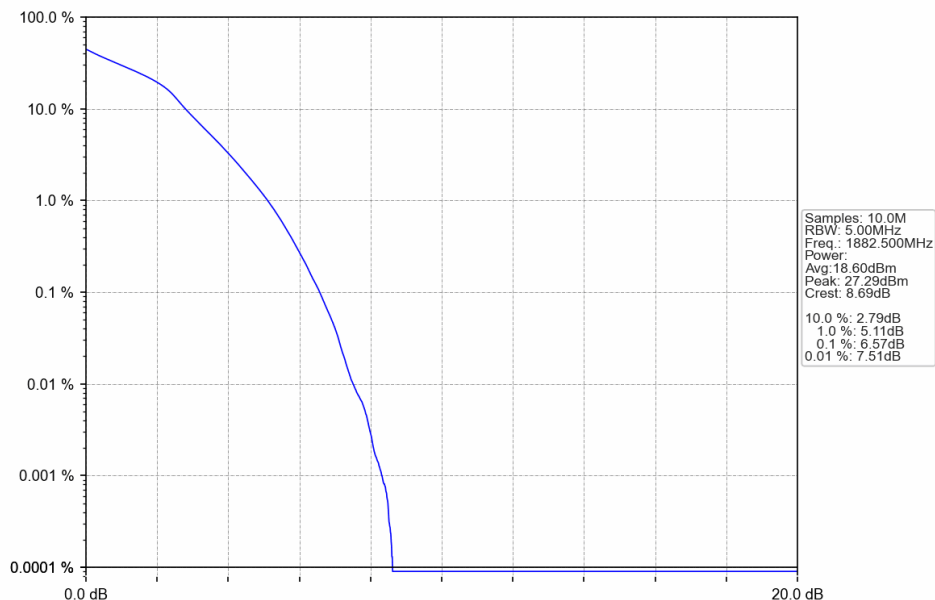
Band25_5MHz_16QAM_MCH_1882.5MHz_RB_25_0_NTNV
