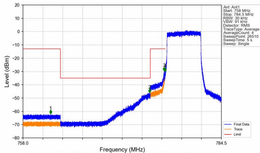
Band13_5MHz_16QAM_LCH_779.5MHz_RB_25_0_NTNV
