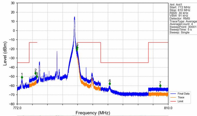
Band13_10MHz_16QAM_HCH_782MHz_RB_1_49_NTNV
