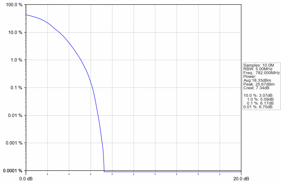
Band13_10MHz_16QAM_LCH_782MHz_RB_50_0_NTNV
