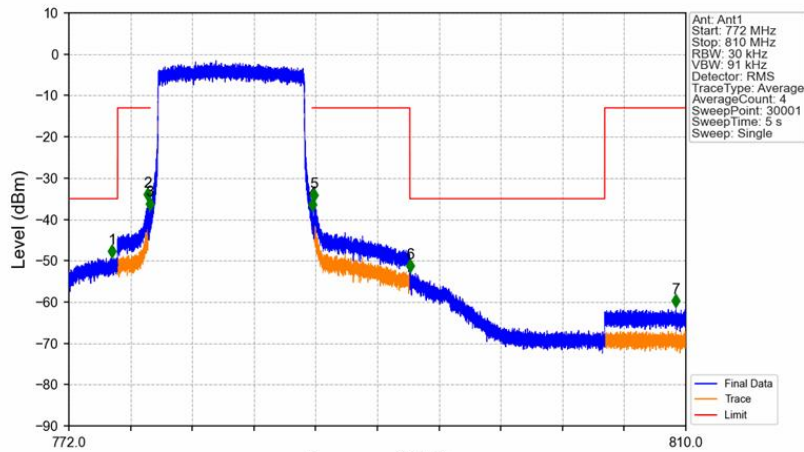
Band13_10MHz_16QAM_HCH_782MHz_RB_50_0_NTNV
