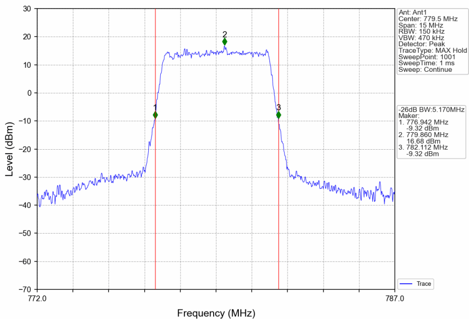
Band13_5MHz_16QAM_LCH_779.5MHz_RB_25_0_NTNV
