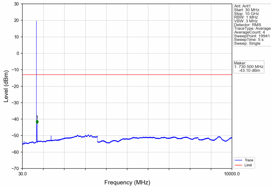
Band12_3MHz_16QAM_LCH_700.5MHz_RB_15_0_NTNV
