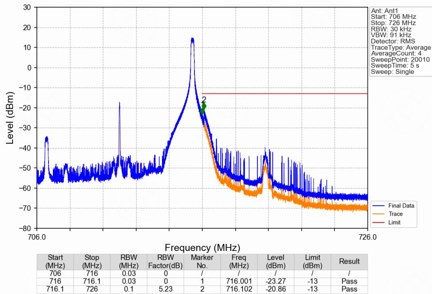
Band12_10MHz_QPSK_HCH_711MHz_RB_1_49_NTNV
