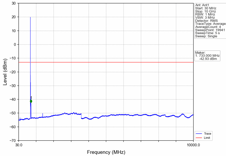
Band12_10MHz_16QAM_LCH_704MHz_RB_50_0_NTNV
