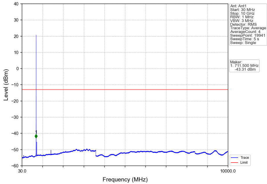
Band12_1.4MHz_QPSK_HCH_715.3MHz_RB_1_5_NTNV
