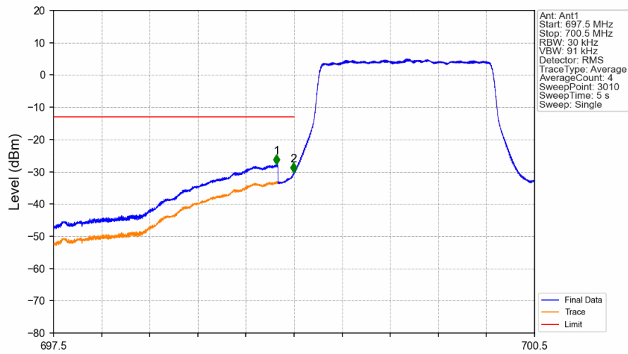
Band12_1.4MHz_16QAM_LCH_699.7MHz_RB_6_0_NTNV
