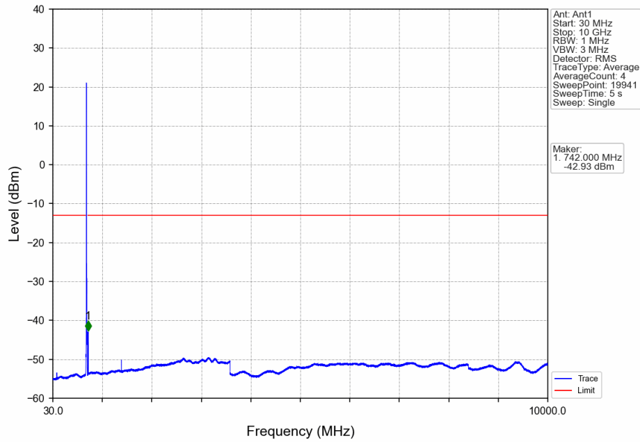
Band12_10MHz_QPSK_HCH_711MHz_RB_1_49_NTNV
