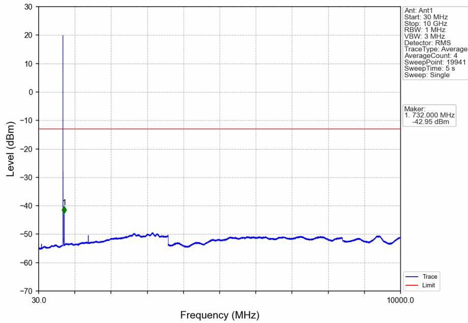
Band12_5MHz_16QAM_LCH_701.5MHz_RB_25_0_NTNV
