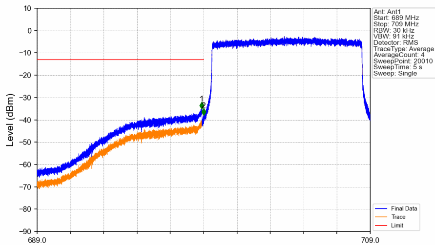
Band12_10MHz_16QAM_LCH_704MHz_RB_50_0_NTNV
