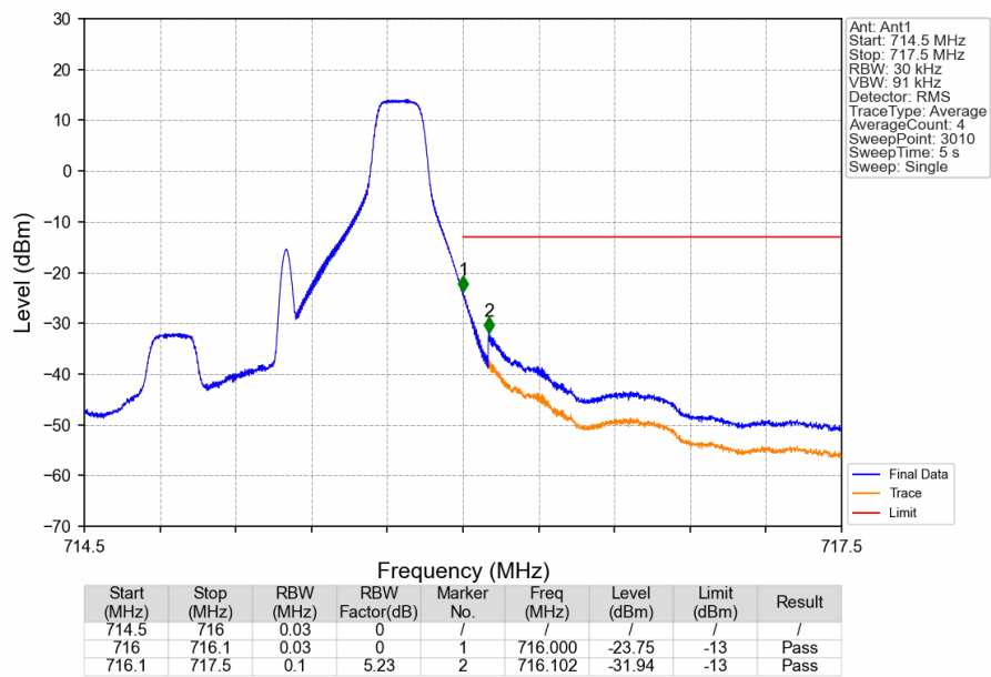
Band12_1.4MHz_QPSK_HCH_715.3MHz_RB_1_5_NTNV
