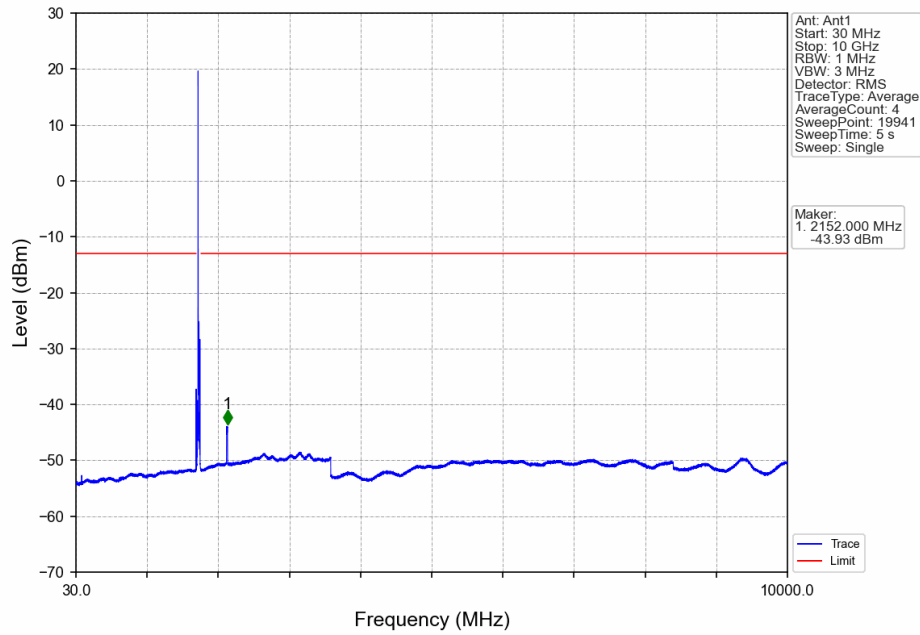
Band4_15MHz_16QAM_HCH_1747.5MHz_RB_1_0_NTNV
