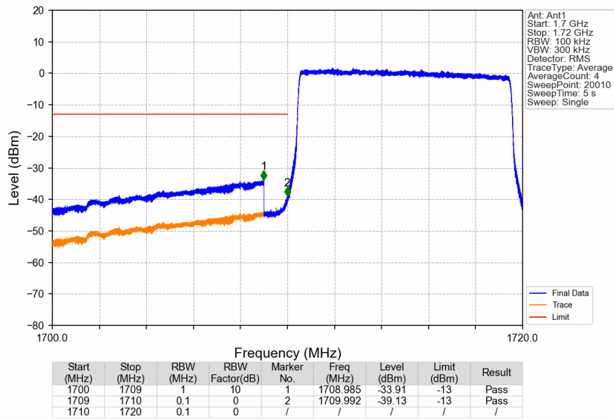
Band4_10MHz_16QAM_LCH_1715MHz_RB_50_0_NTNV
