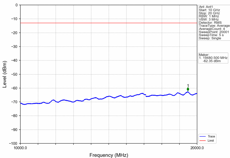
Band2_1.4MHz_16QAM_MCH_1880MHz_RB_1_0_NTNV
