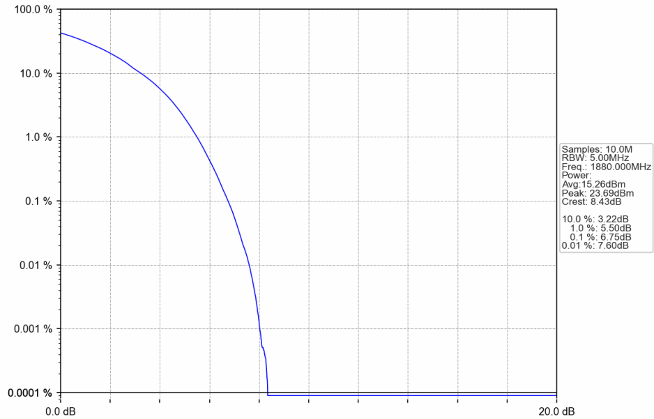
Band2_15MHz_16QAM_MCH_1880MHz_RB_75_0_NTNV
