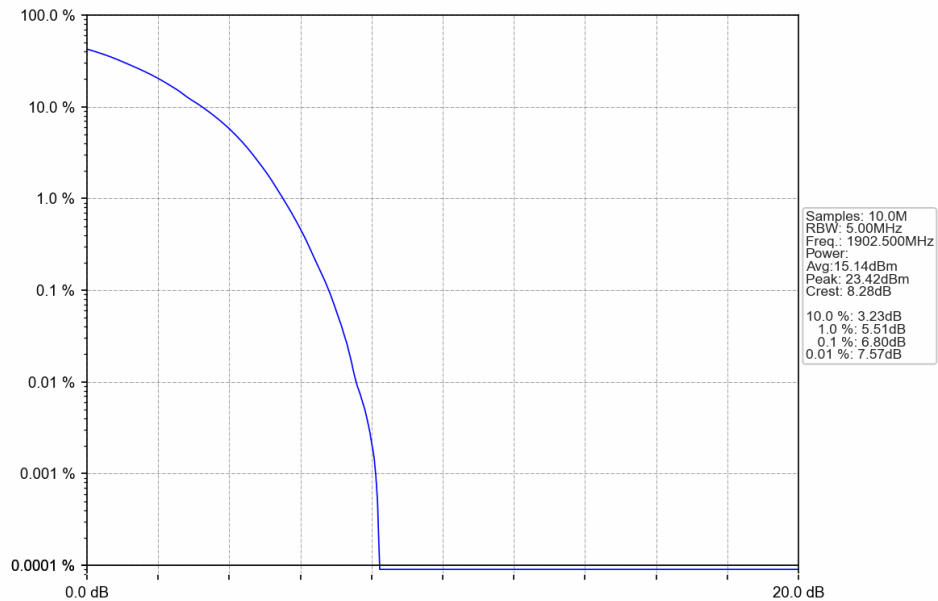
Band2_15MHz_16QAM_HCH_1902.5MHz_RB_75_0_NTNV
