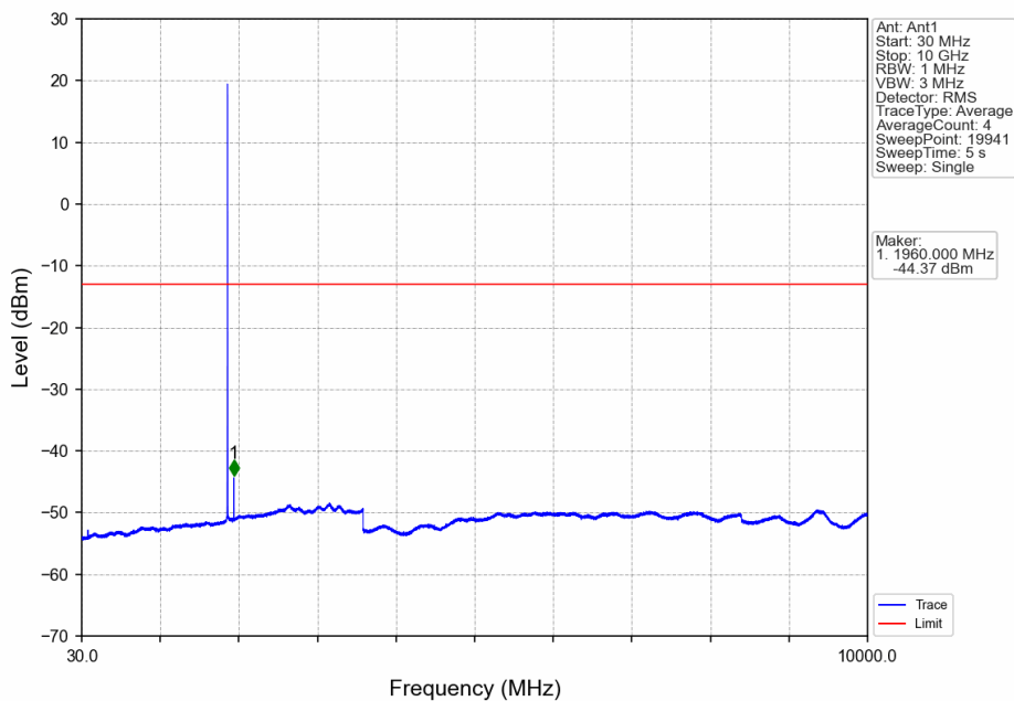
Band2_1.4MHz_16QAM_MCH_1880MHz_RB_1_0_NTNV
