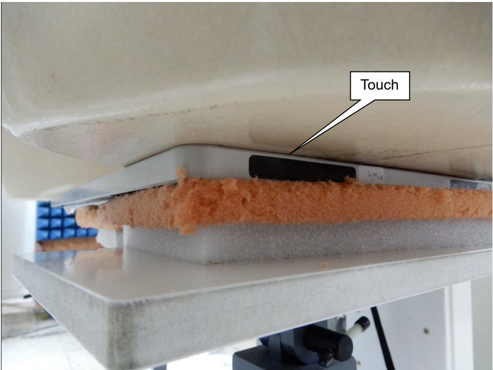
EUT Back – Limb SAR (Main Antenna)
