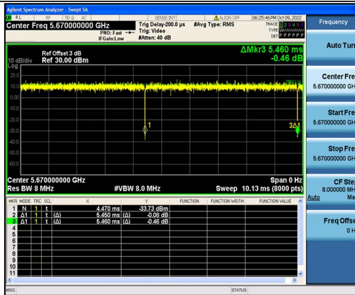
802.11ax(HE40)_Ant2_5670
