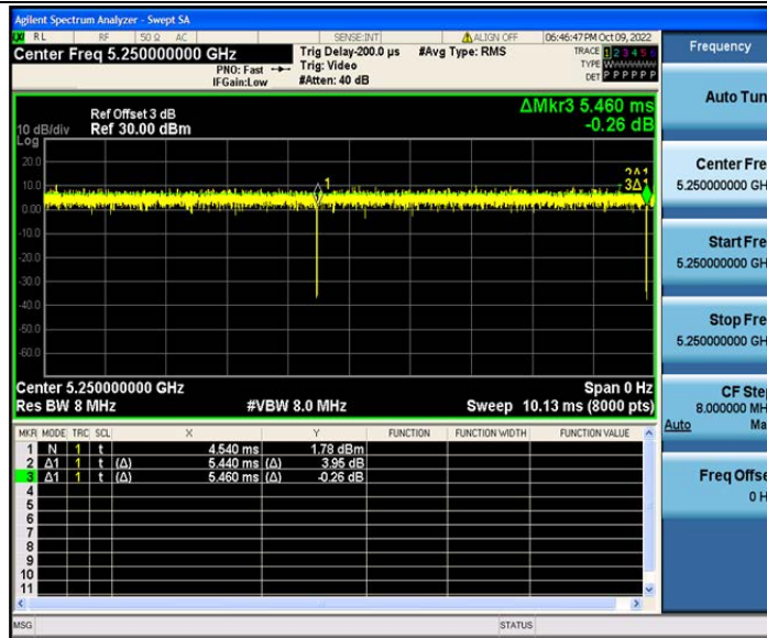
802.11ax(HE160)_Ant2_5250
