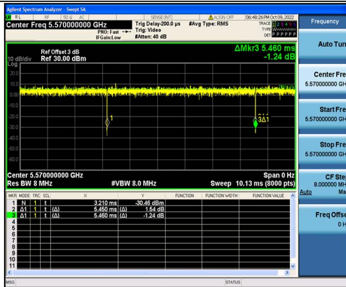
802.11ax(HE160)_Ant2_5570
