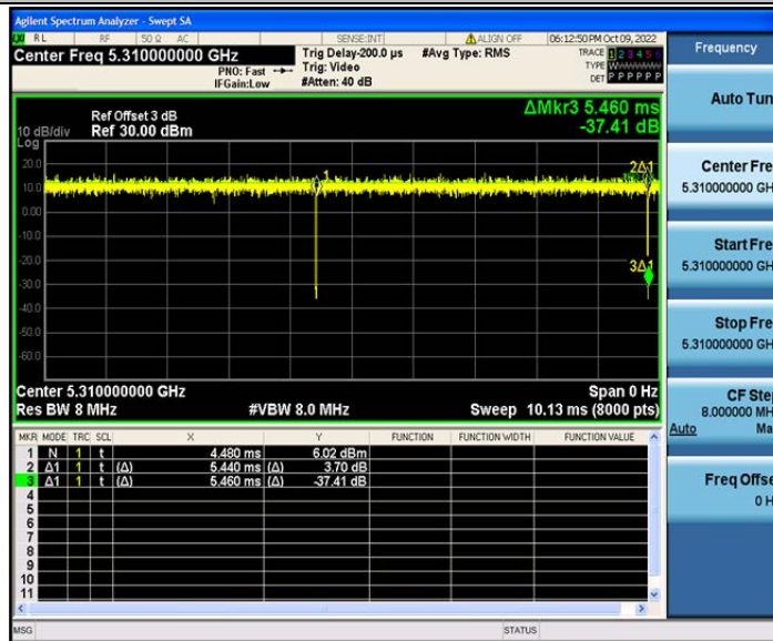
802.11ax(HE40)_Ant2_5310
