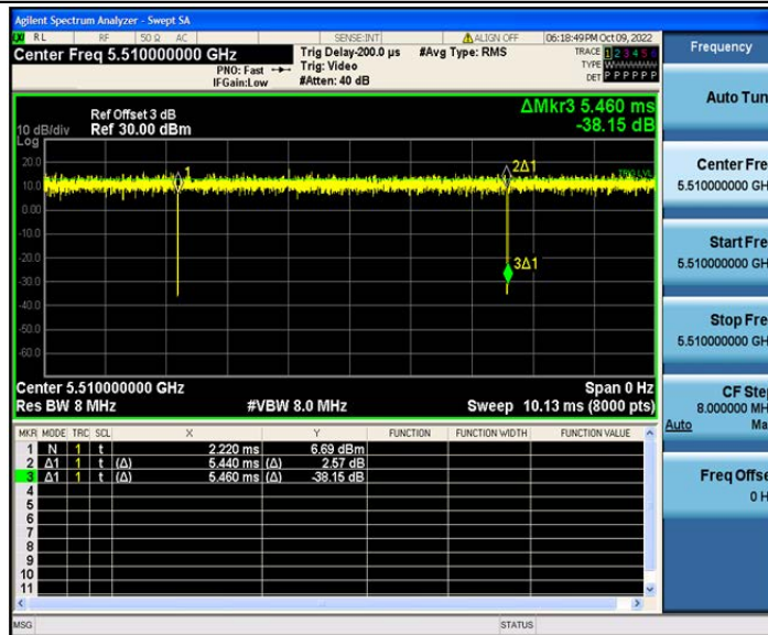
802.11ax(HE40)_Ant2_5510
