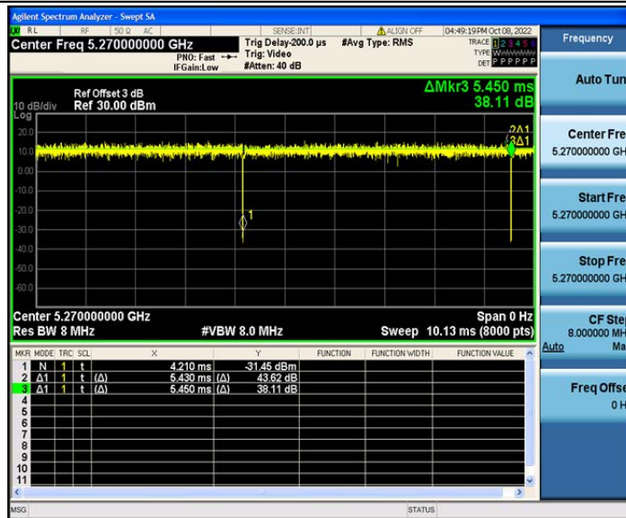
802.11ac(VHT40)_Ant2_5270
