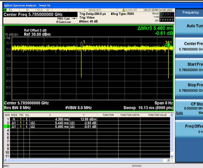
802.11ax(HE20)_Ant2_5785
