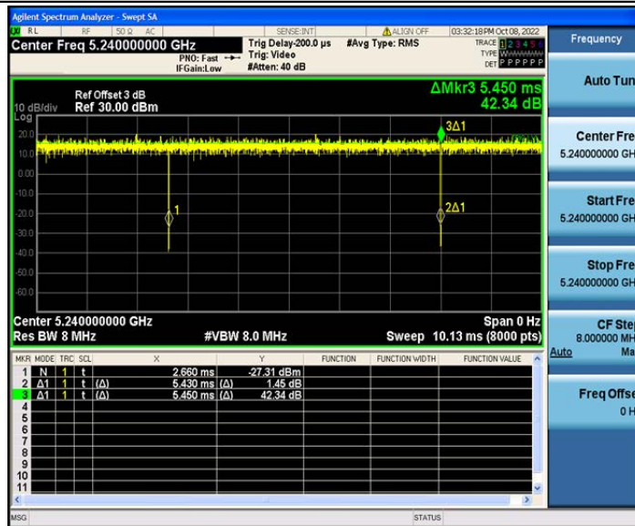
802.11ac(VHT20)_Ant2_5240
