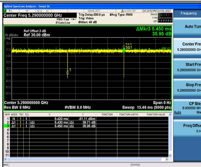
802.11ac(VHT80)_Ant2_5290
