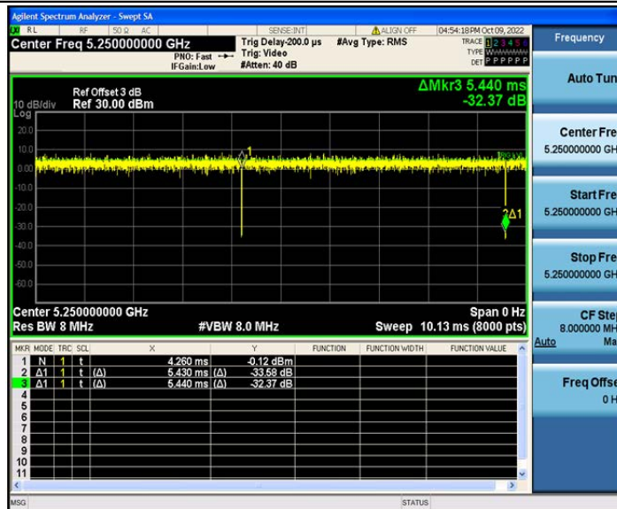
802.11ac(VHT160)_Ant2_5250
