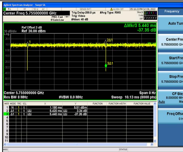
802.11ac(VHT40)_Ant2_5755
