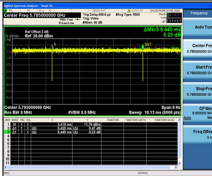
802.11ac(VHT20)_Ant2_5785
