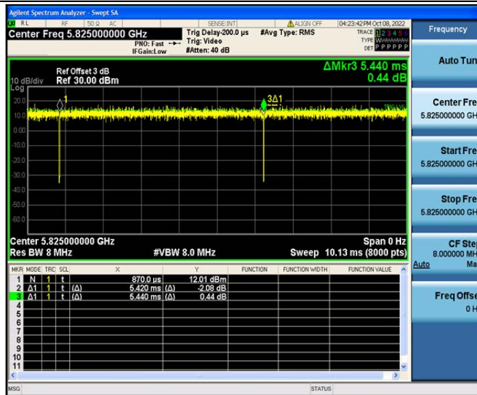
802.11ac(VHT20)_Ant2_5825
