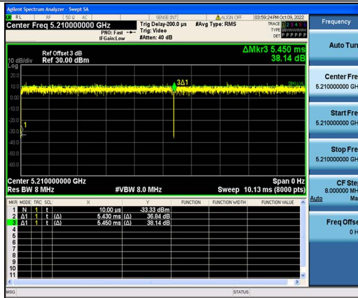
802.11ac(VHT80)_Ant2_5210
