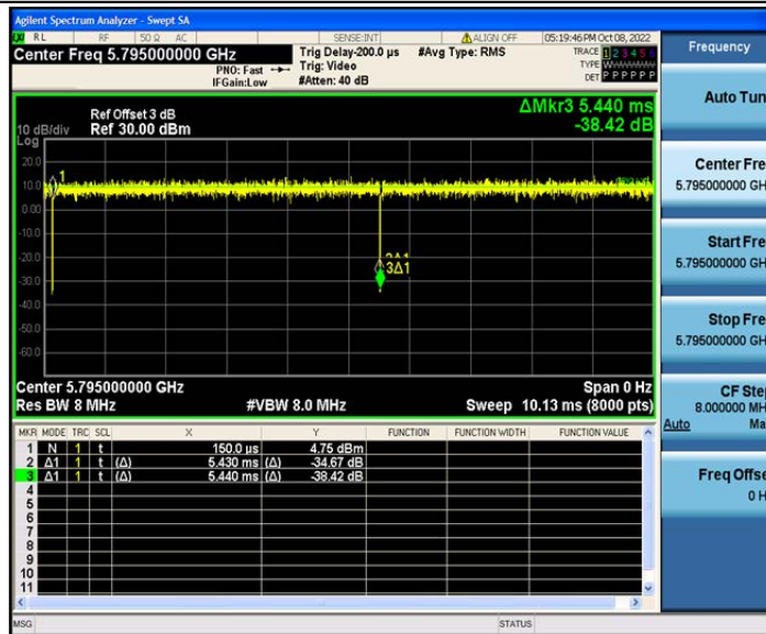
802.11ac(VHT40)_Ant2_5795
