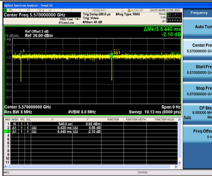
802.11ac(VHT160)_Ant2_5570
