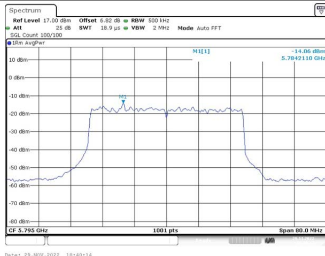
802.11ax(HE40)_Ant2_5795 106/54
