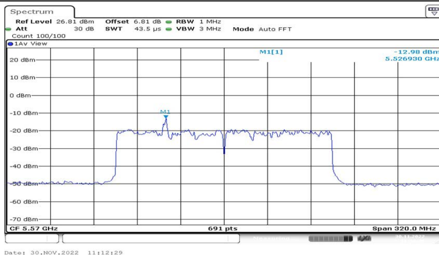
802.11ax(HE160)_Ant2_5570 52/44
