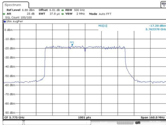
802.11ax(HE80)_Ant2_5775 106/56
