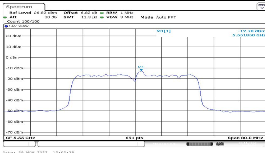
802.11ax(HE40)_Ant2_5550 26/8
