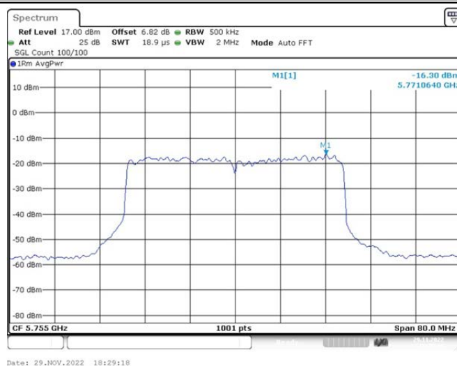
802.11ax(HE40)_Ant2_5755 106/54
