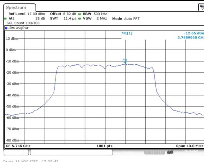
802.11ax(HE20)_Ant2_5745 52/38
