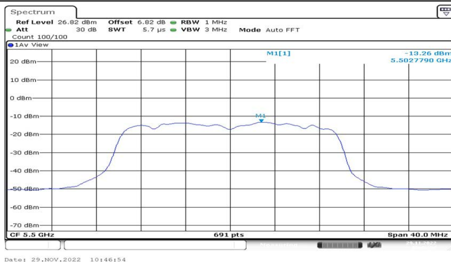
802.11ax(HE20)_Ant2_5500 106/53
