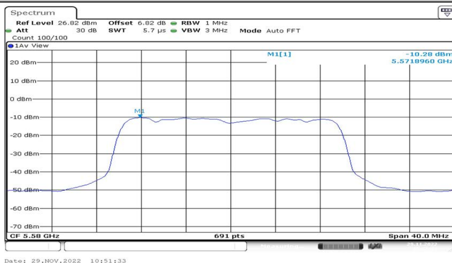
802.11ax(HE20)_Ant2_5580 52/38
