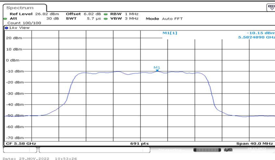
802.11ax(HE20)_Ant2_5580 106/53
