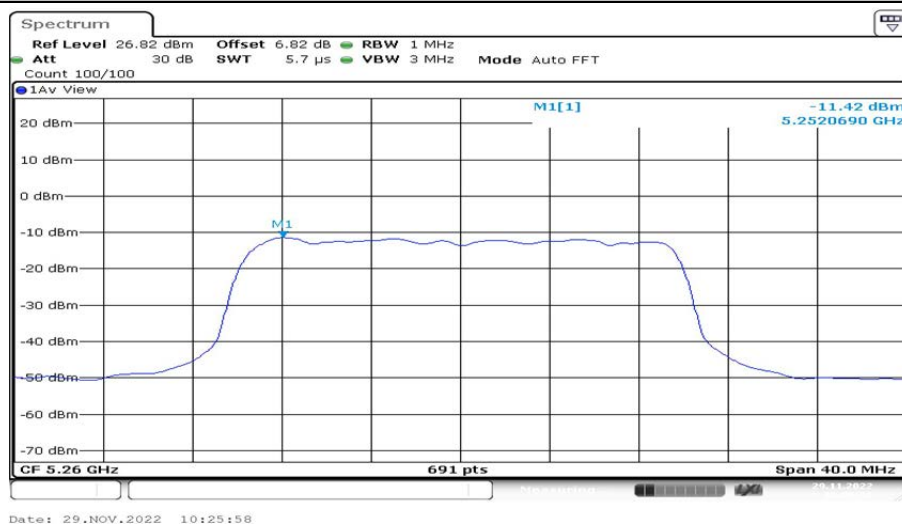
802.11ax(HE20)_Ant2_5260 106/53
