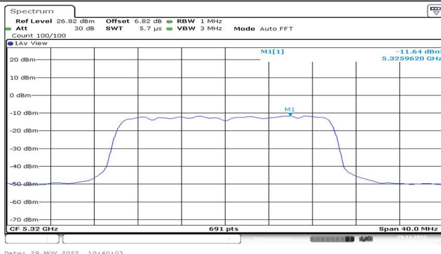
802.11ax(HE20)_Ant2_5320 106/53
