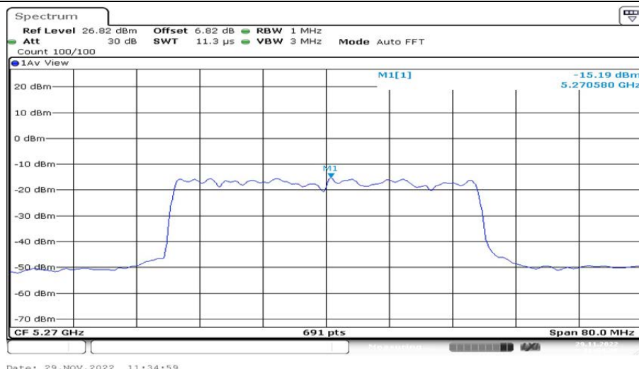
802.11ax(HE40)_Ant2_5270 26/8
