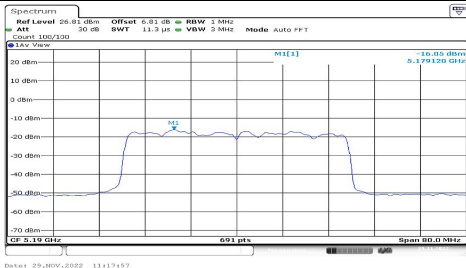
802.11ax(HE40)_Ant2_5190 26/8
