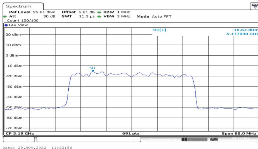
802.11ax(HE40)_Ant2_5190 106/54
