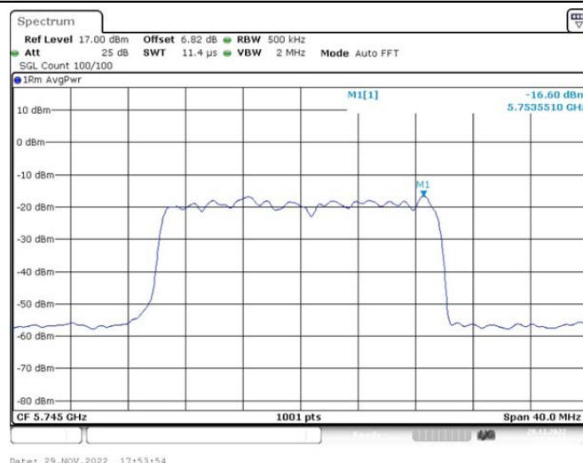
802.11ax(HE20)_Ant2_5745 106/53
