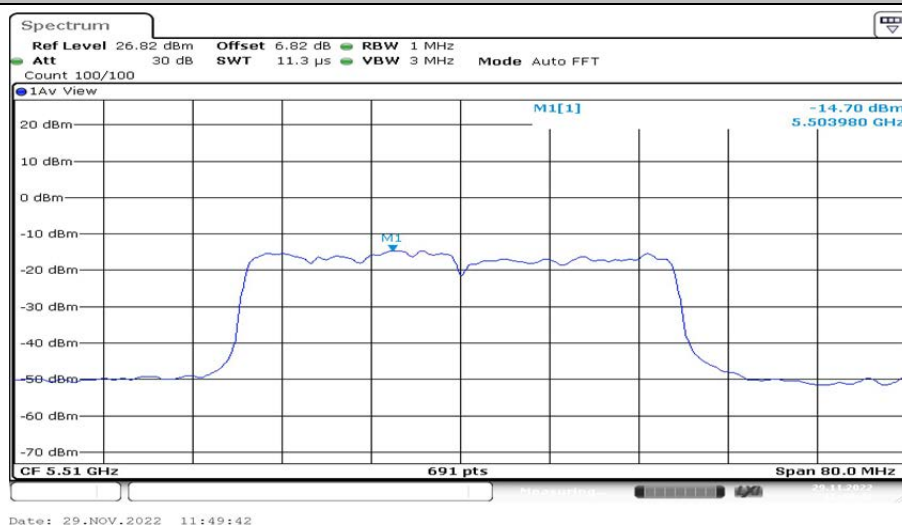
802.11ax(HE40)_Ant2_5510 106/54
