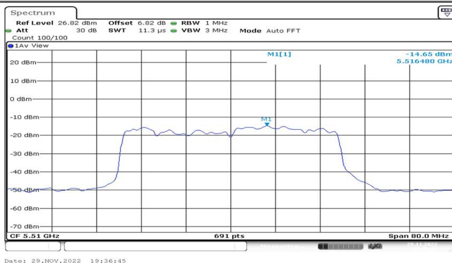
802.11ax(HE40)_Ant2_5510 52/40
