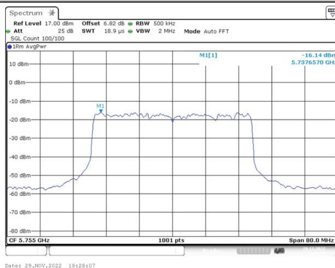
802.11ax(HE40)_Ant2_5755 26/8
