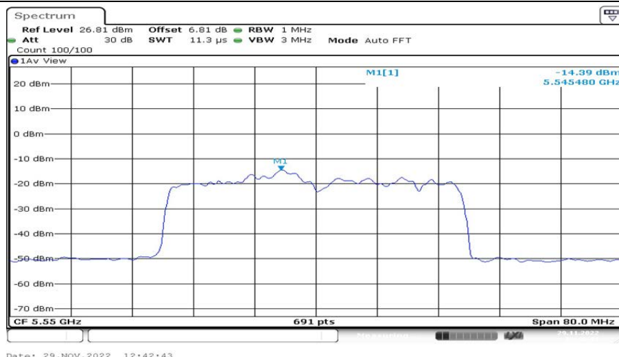
802.11ax(HE40)_Ant2_5550 106/54
