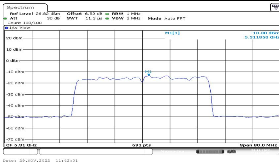
802.11ax(HE40)_Ant2_5310 26/8
