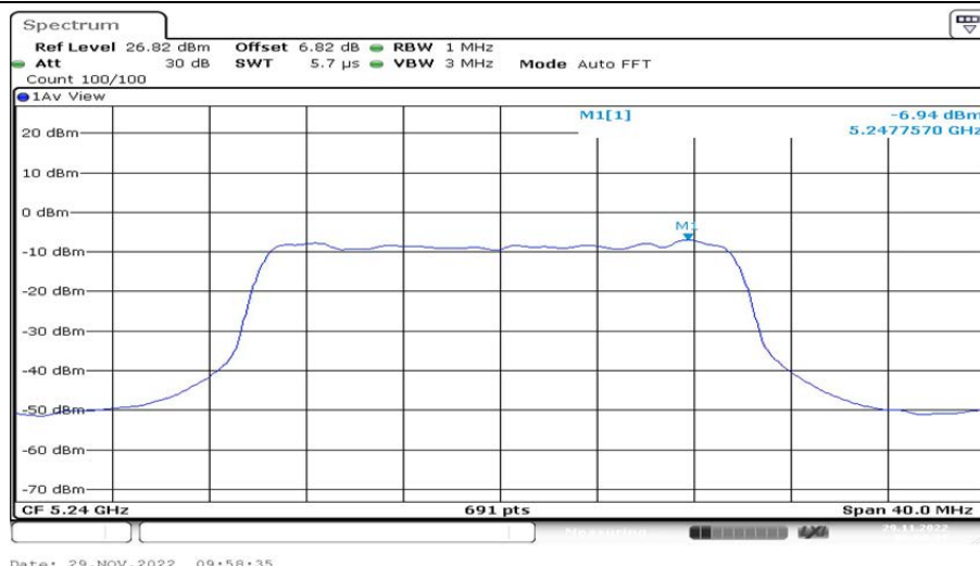
802.11ax(HE20)_Ant2_5240 106/53
