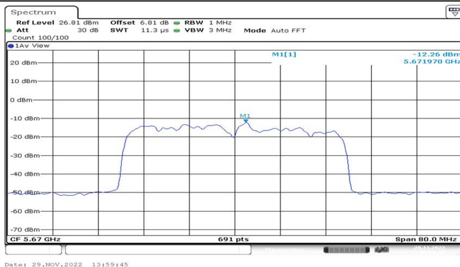
802.11ax(HE40)_Ant2_5670 26/8
