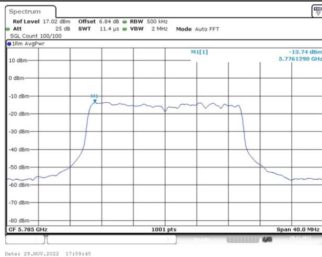
802.11ax(HE20)_Ant2_5785 106/53
