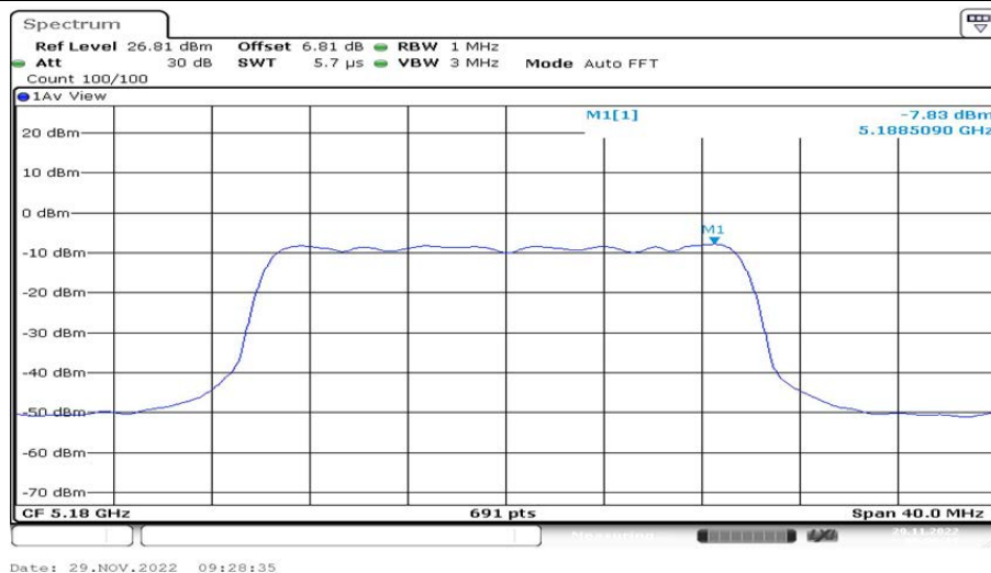
802.11ax(HE20)_Ant2_5180 106/53
