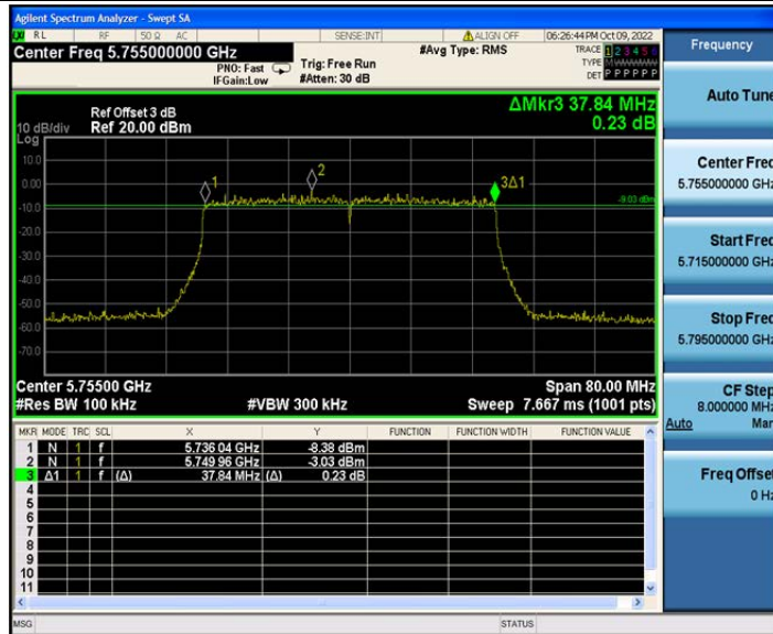
802.11ax(HE40)_Ant2_5755 484/65
