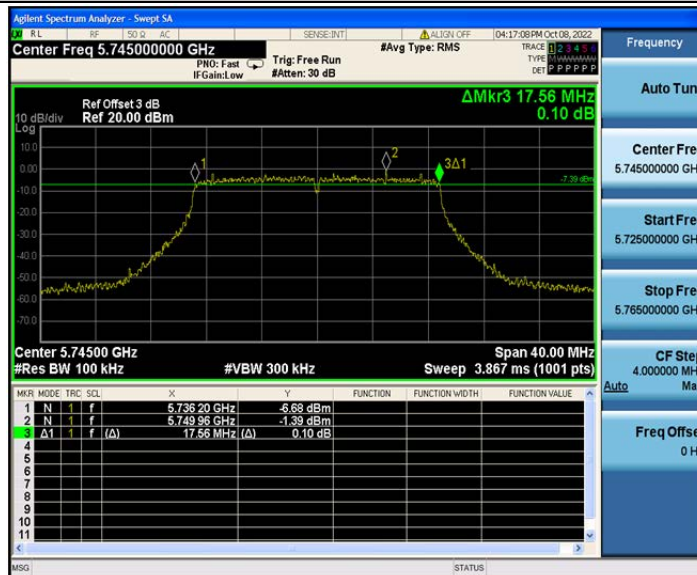
802.11ac(VHT20)_Ant2_5745
