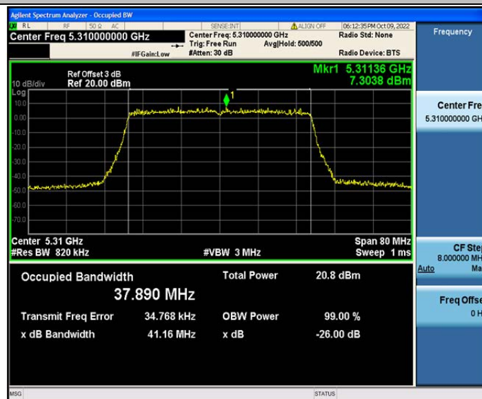
802.11ax(HE40)_Ant2_5310 484/65
