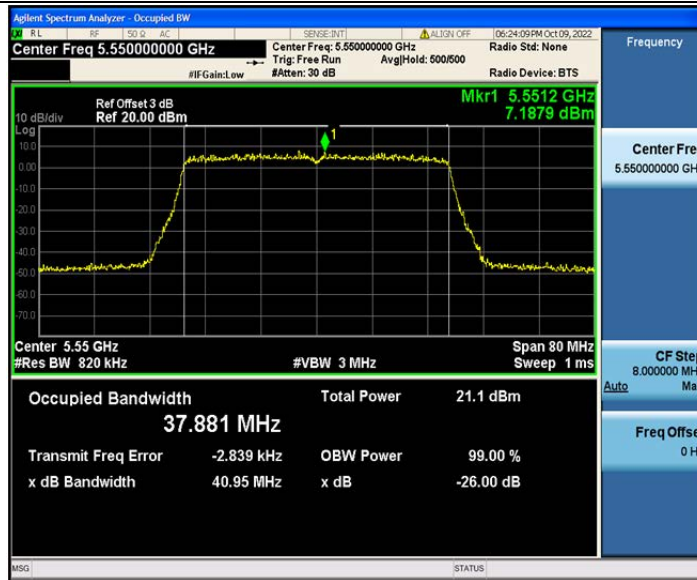
802.11ax(HE40)_Ant2_5550 484/65
