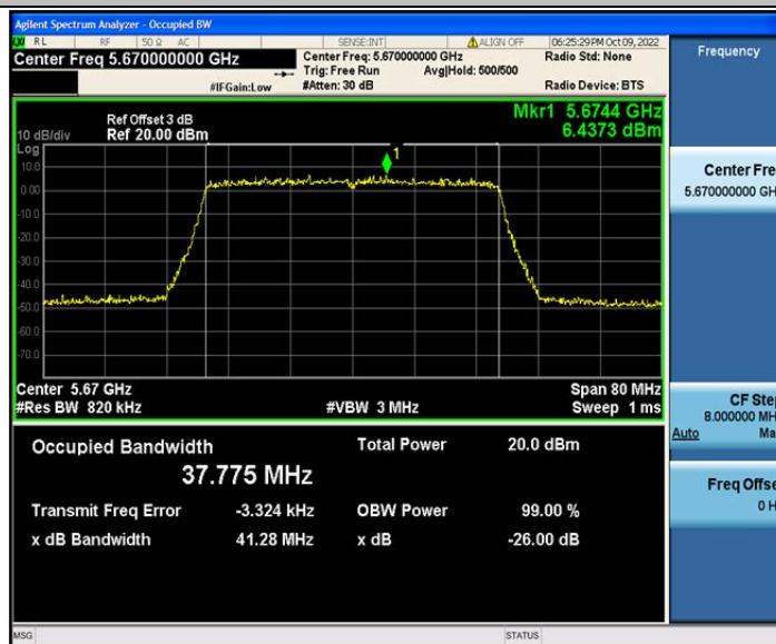
802.11ax(HE40)_Ant2_5670 484/65
