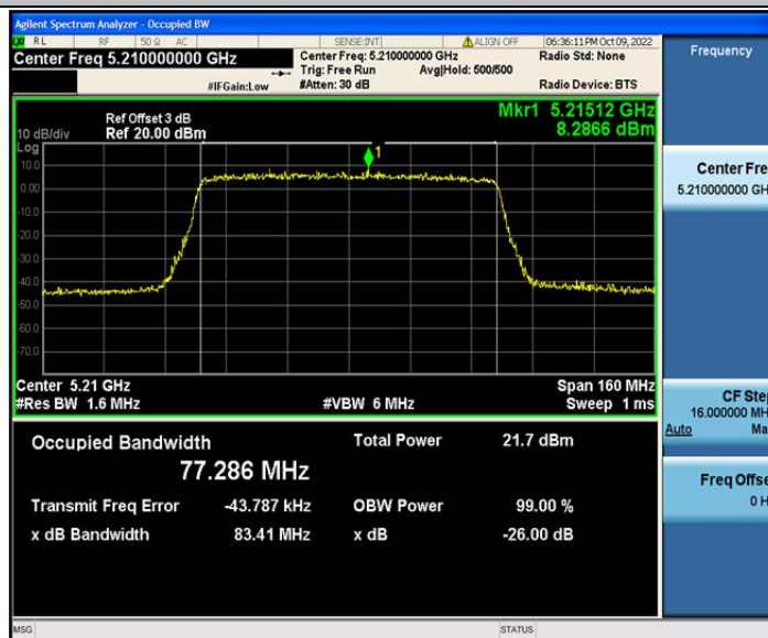
802.11ax(HE80)_Ant2_5210 996/67
