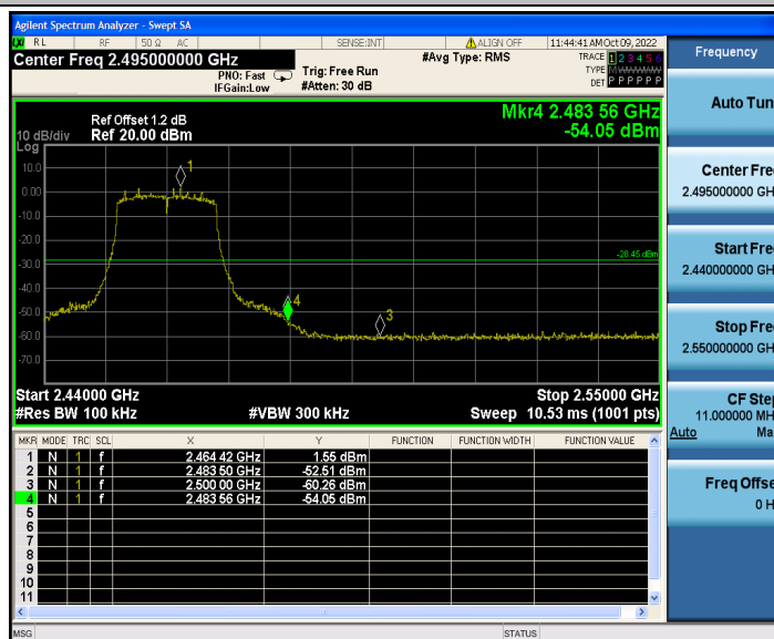
802.11n(HT20)_Ant2_High_2462
