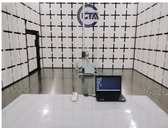
radiation H
