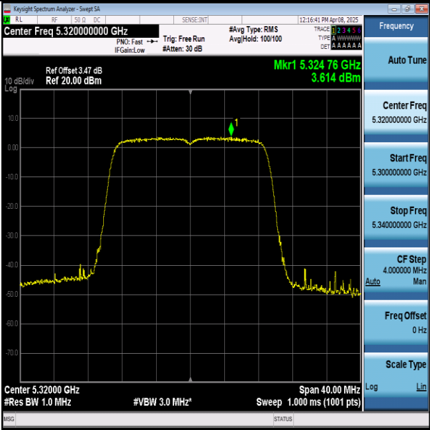
11AC20MIMO-Ant1-5320-PASS
