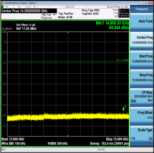
11N40SISO-Ant1-2452-13000~15000-PASS
