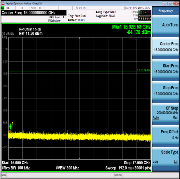
11N40SISO-Ant1-2452-15000~17000-PASS
