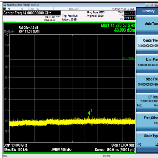
11AX20SISO-Ant1-2437-13000~15000-PASS
