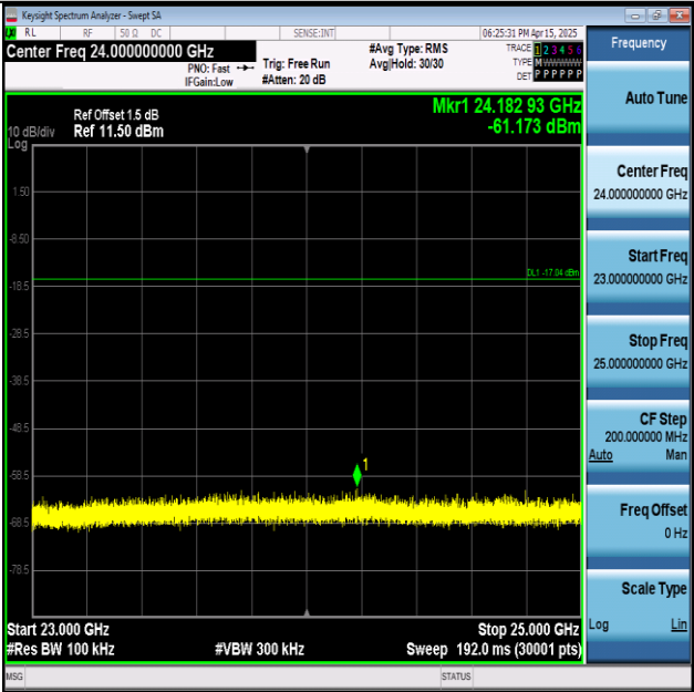
11N40SISO-Ant1-2452-23000~25000-PASS
