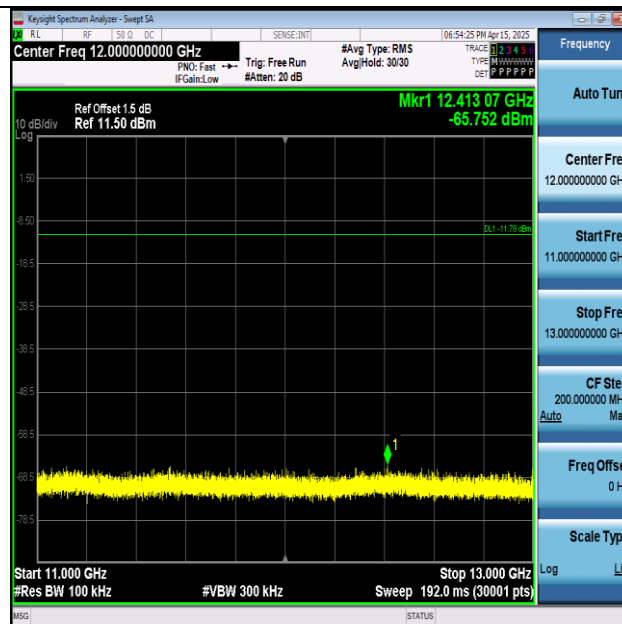
11AX20SISO-Ant1-2412-11000~13000-PASS
