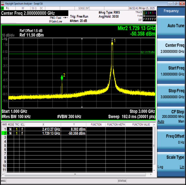
11AX20SISO-Ant1-2412-1000~3000-PASS
