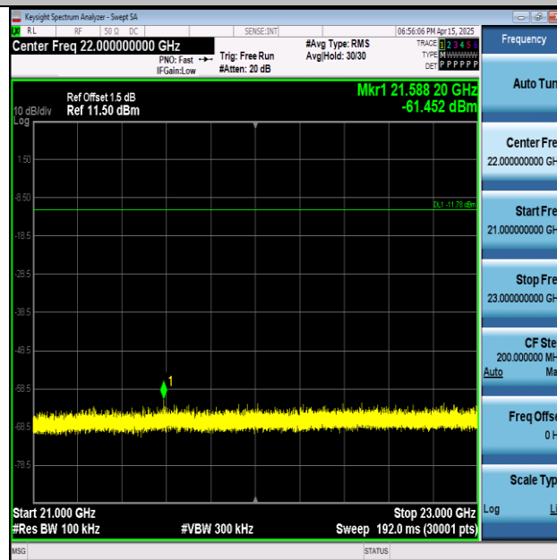
11AX20SISO-Ant1-2412-21000~23000-PASS
