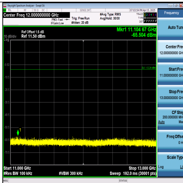
11AX20SISO-Ant1-2462-11000~13000-PASS
