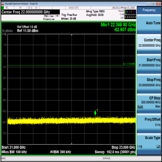
11N40SISO-Ant1-2452-21000~23000-PASS
