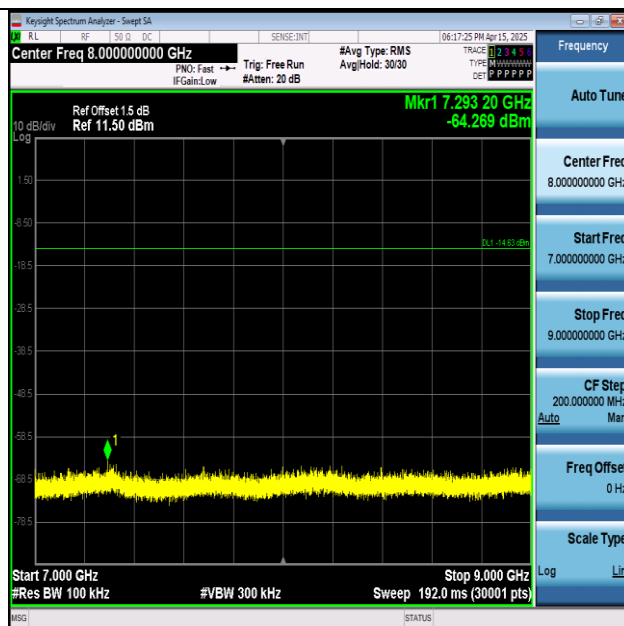
11N40SISO-Ant1-2437-7000~9000-PASS
