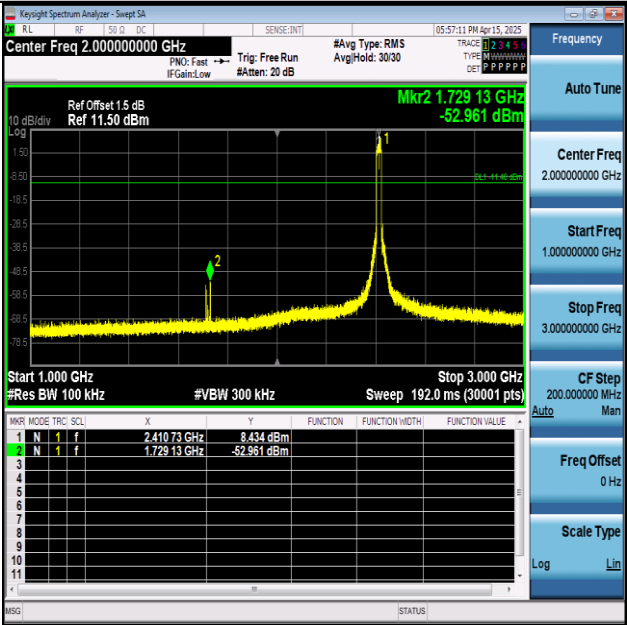
11N20SISO-Ant1-2412-1000~3000-PASS
