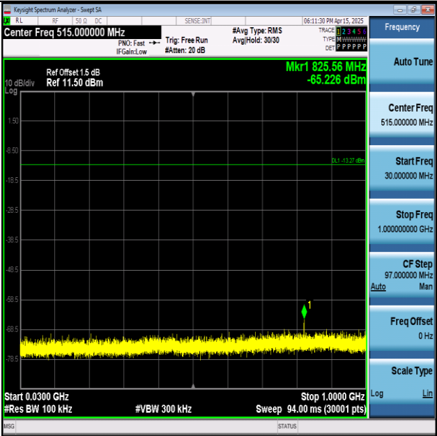
11N40SISO-Ant1-2422-30~1000-PASS
