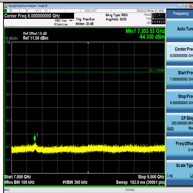
11N20SISO-Ant1-2437-7000~9000-PASS
