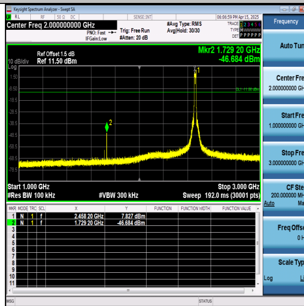
11N20SISO-Ant1-2462-1000~3000-PASS
