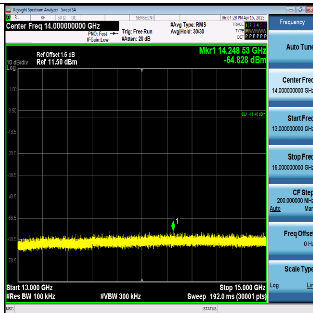
11N20SISO-Ant1-2437-13000~15000-PASS
