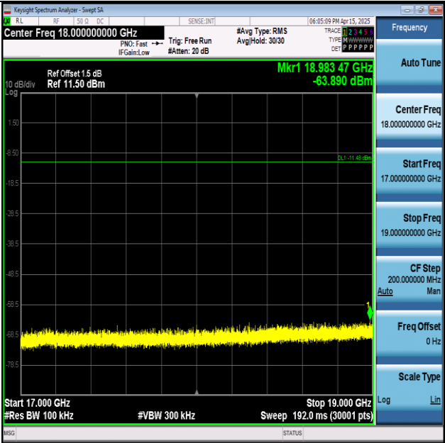
11N20SISO-Ant1-2437-17000~19000-PASS
