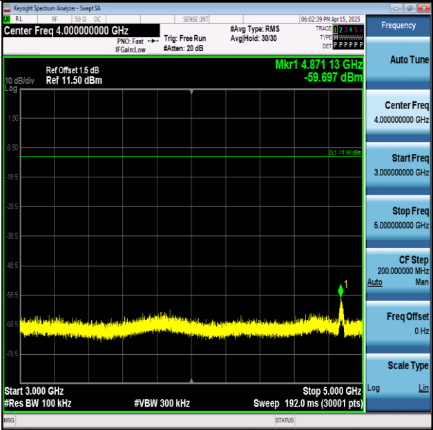
11N20SISO-Ant1-2437-3000~5000-PASS
