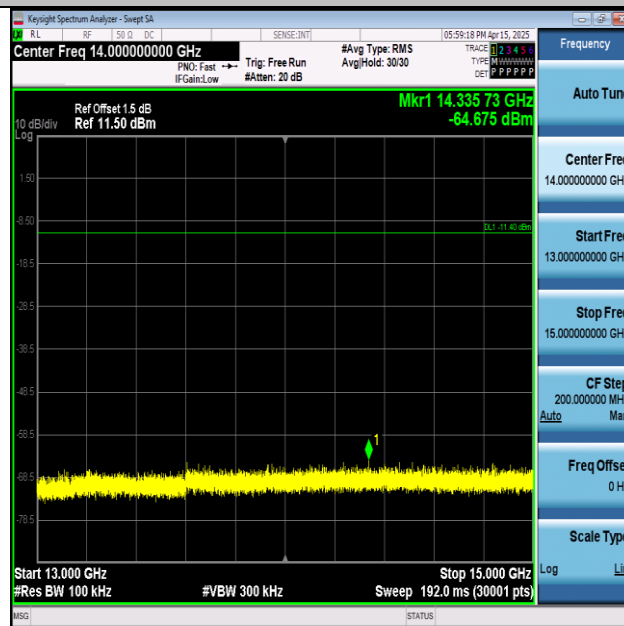
11N20SISO-Ant1-2412-13000~15000-PASS
