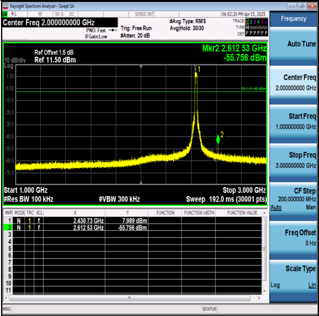
11N20SISO-Ant1-2437-1000~3000-PASS
