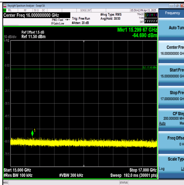
11N20SISO-Ant1-2412-15000~17000-PASS
