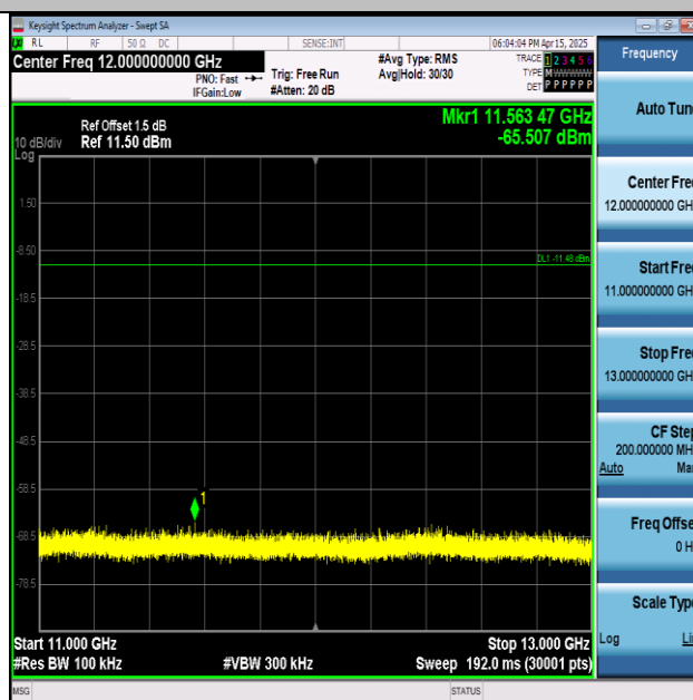
11N20SISO-Ant1-2437-11000~13000-PASS
