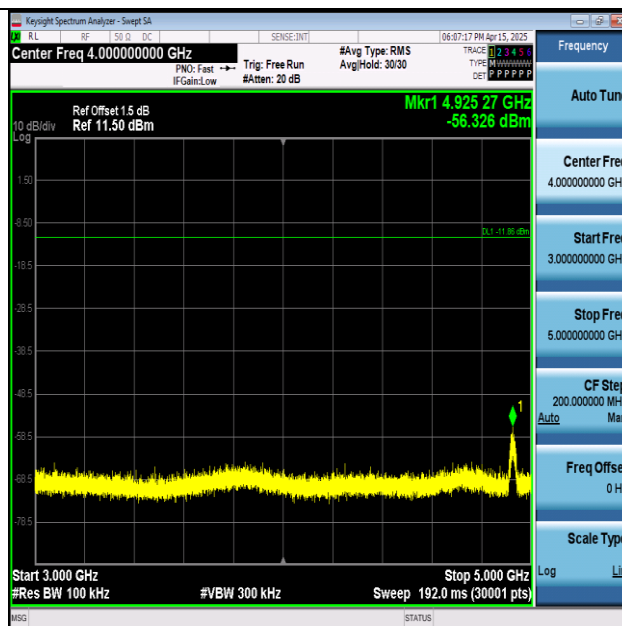
11N20SISO-Ant1-2462-3000~5000-PASS
