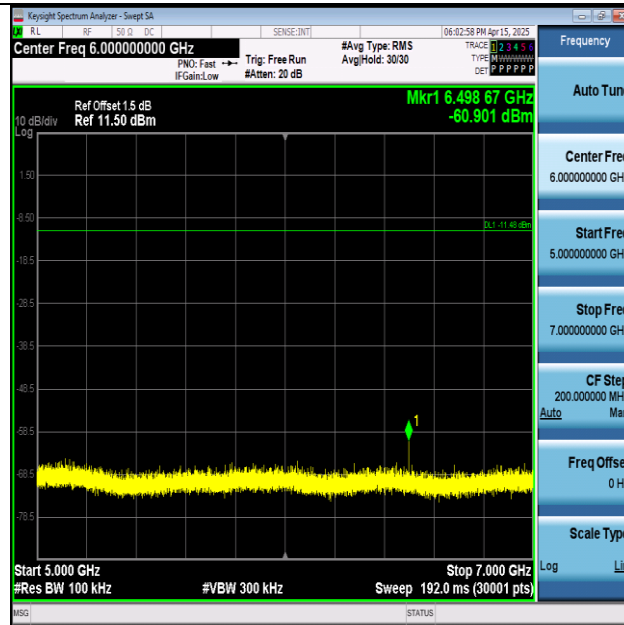
11N20SISO-Ant1-2437-5000~7000-PASS
