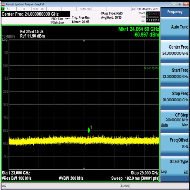
11N20SISO-Ant1-2462-23000~25000-PASS
