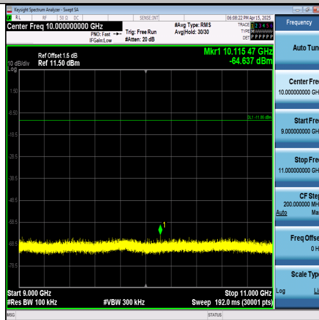
11N20SISO-Ant1-2462-9000~11000-PASS
