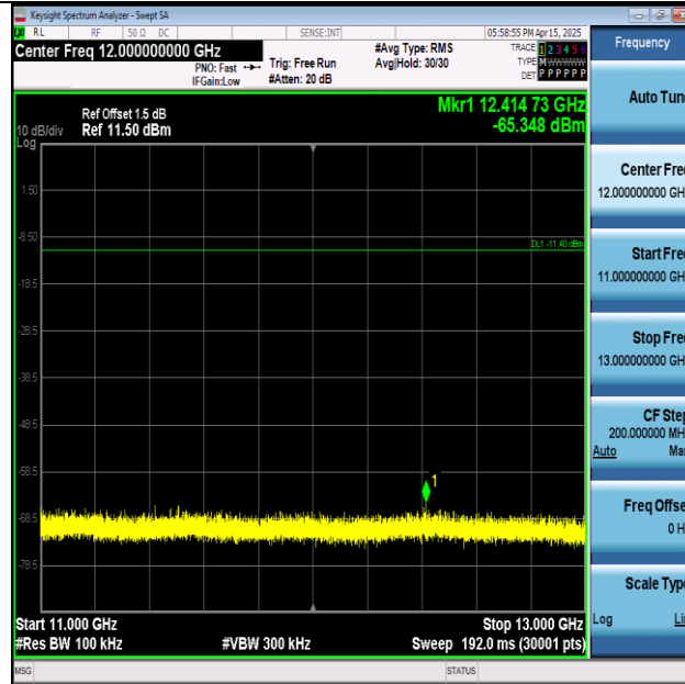
11N20SISO-Ant1-2412-11000~13000-PASS
