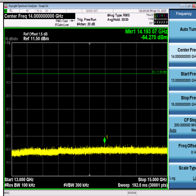
11N20SISO-Ant1-2462-13000~15000-PASS
