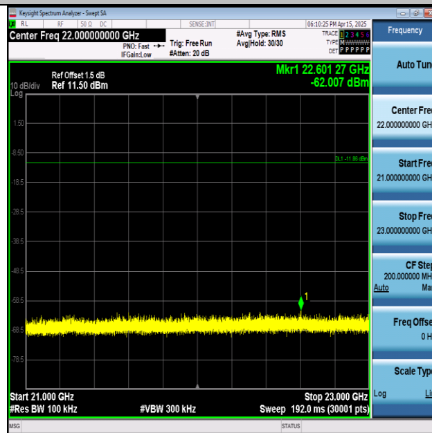
11N20SISO-Ant1-2462-21000~23000-PASS
