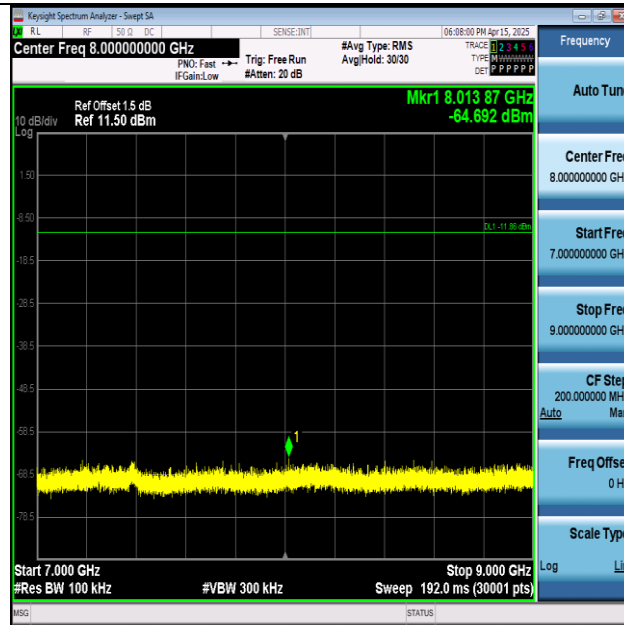
11N20SISO-Ant1-2462-7000~9000-PASS
