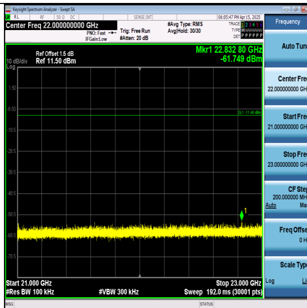
11N20SISO-Ant1-2437-21000~23000-PASS
