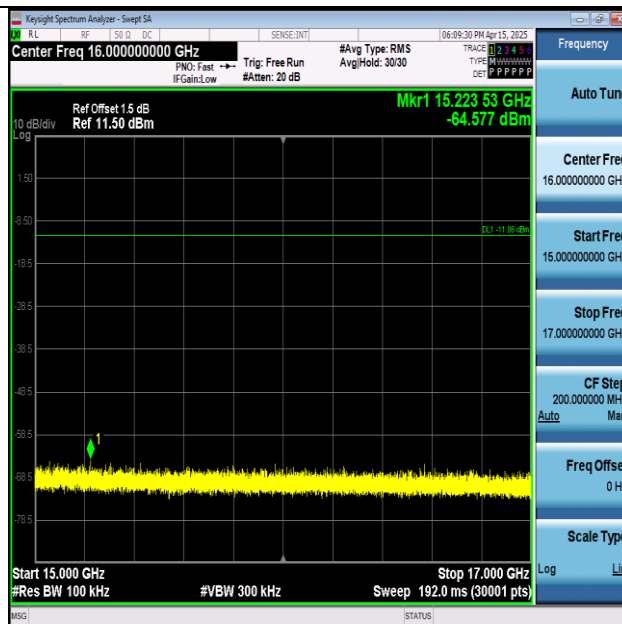
11N20SISO-Ant1-2462-15000~17000-PASS
