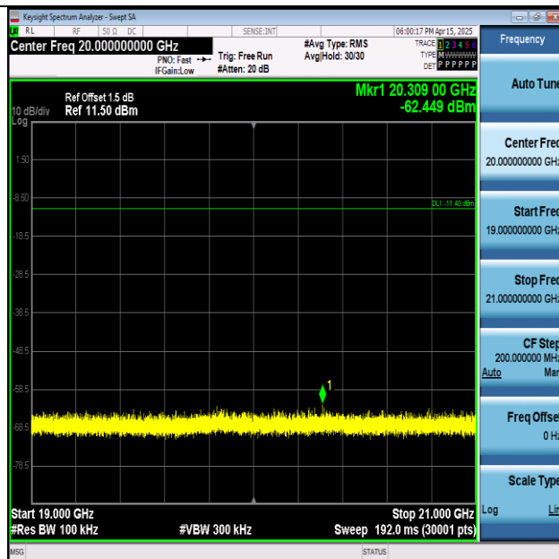
11N20SISO-Ant1-2412-19000~21000-PASS
