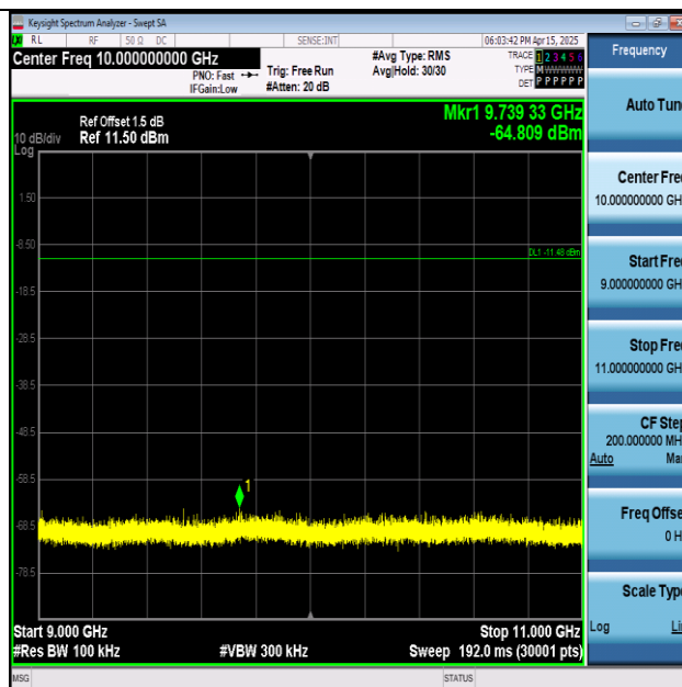
11N20SISO-Ant1-2437-9000~11000-PASS
