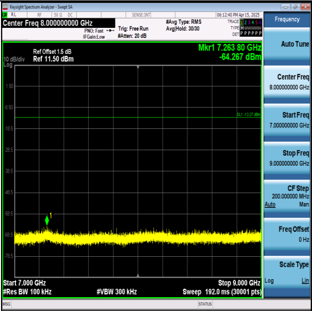
11N40SISO-Ant1-2422-7000~9000-PASS
