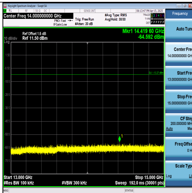
11N40SISO-Ant1-2422-13000~15000-PASS
