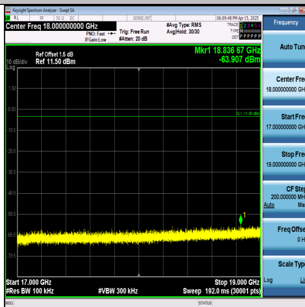
11N20SISO-Ant1-2462-17000~19000-PASS
