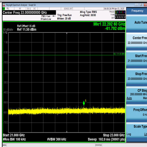
11N20SISO-Ant1-2412-21000~23000-PASS
