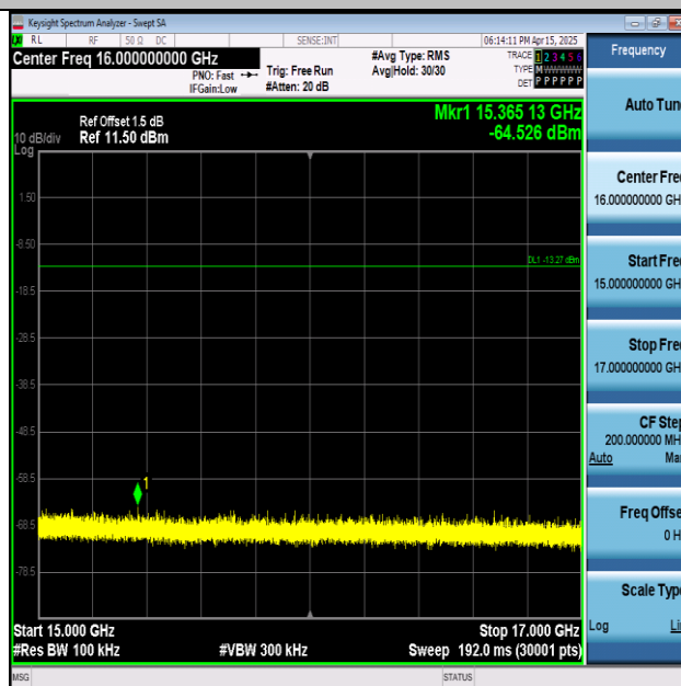
11N40SISO-Ant1-2422-15000~17000-PASS
