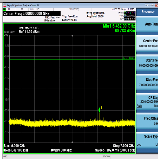
11N20SISO-Ant1-2412-5000~7000-PASS
