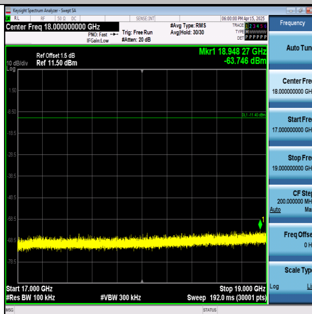
11N20SISO-Ant1-2412-17000~19000-PASS
