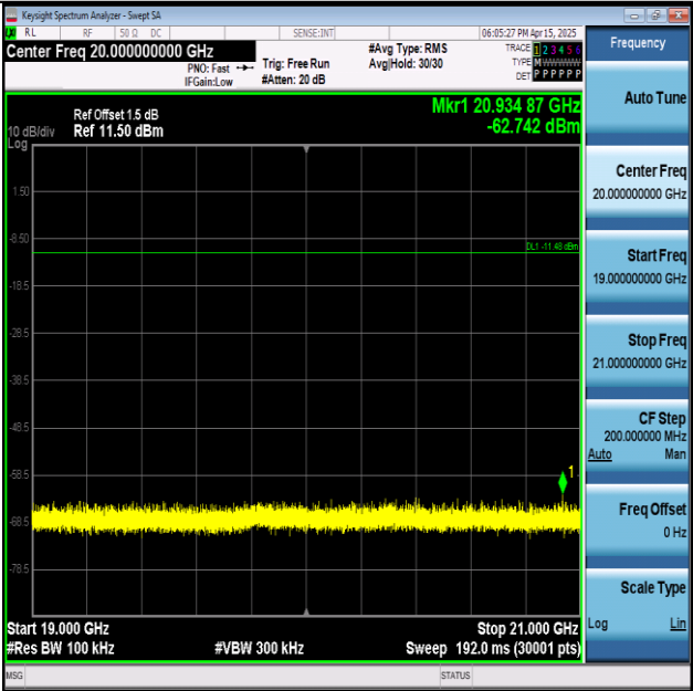
11N20SISO-Ant1-2437-19000~21000-PASS
