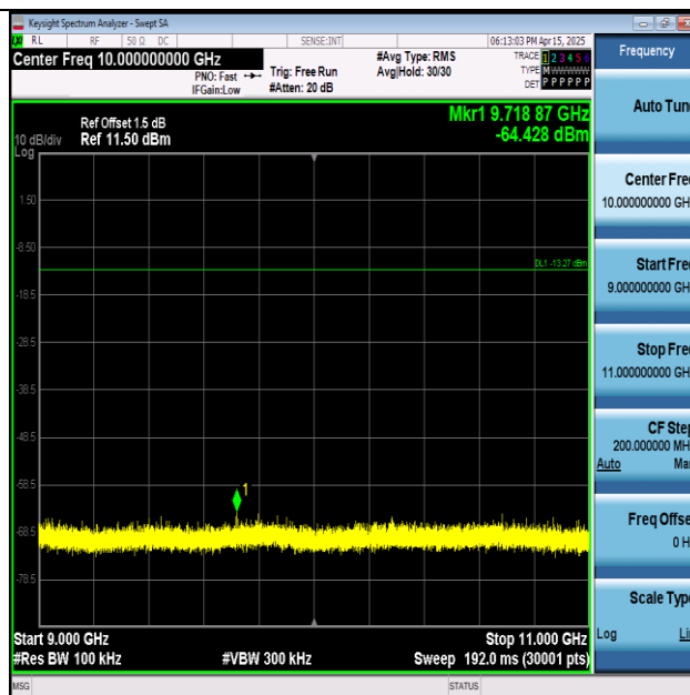
11N40SISO-Ant1-2422-9000~11000-PASS
