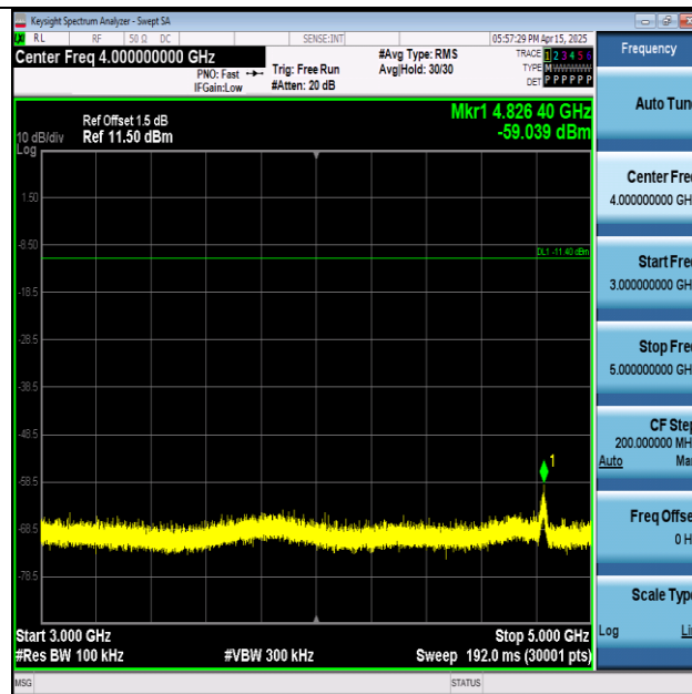
11N20SISO-Ant1-2412-3000~5000-PASS
