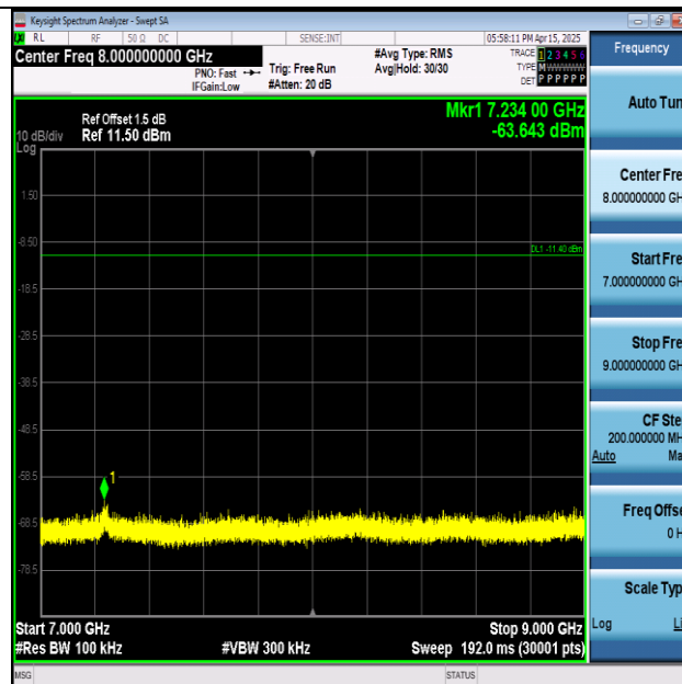
11N20SISO-Ant1-2412-7000~9000-PASS
