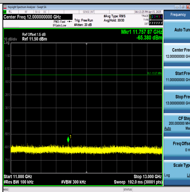
11N40SISO-Ant1-2422-11000~13000-PASS
