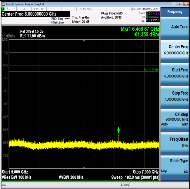
11N40SISO-Ant1-2422-5000~7000-PASS
