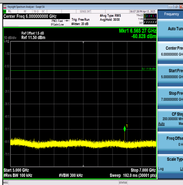
11N20SISO-Ant1-2462-5000~7000-PASS
