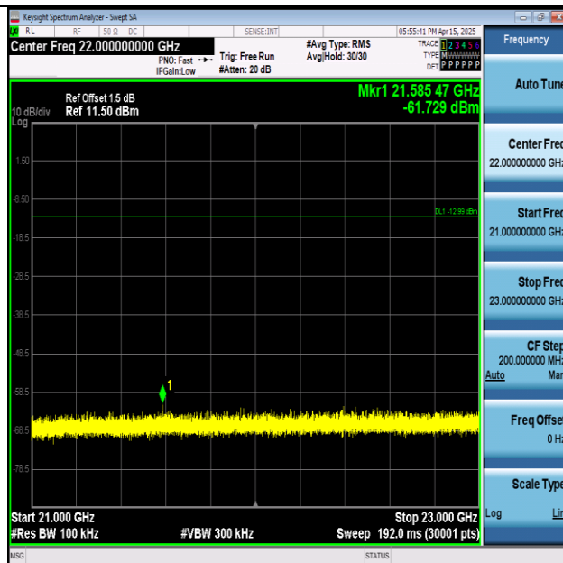
11G-Ant1-2462-21000~23000-PASS
