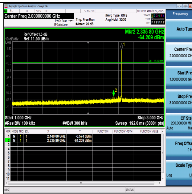
BLE_125K-Ant1-2440-1000~3000-PASS
