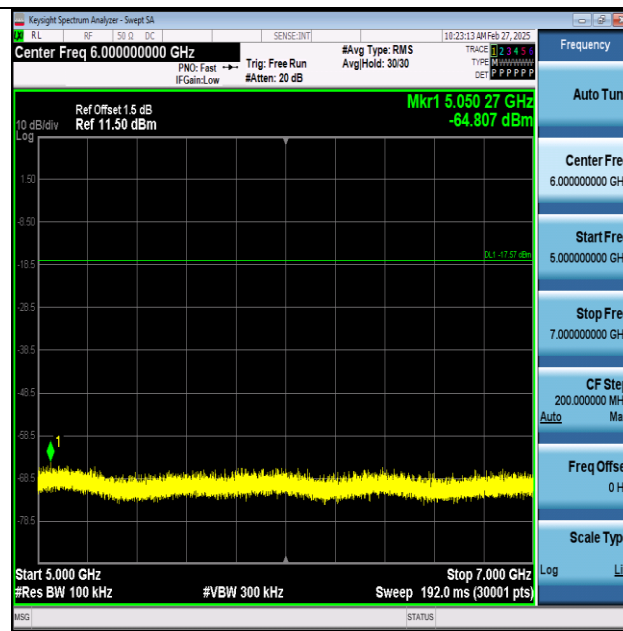
BLE_2M-Ant1-2480-5000~7000-PASS
