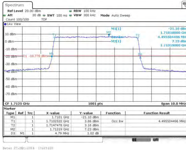
Band66-5MHz-QPSK-132322-25RB#0
