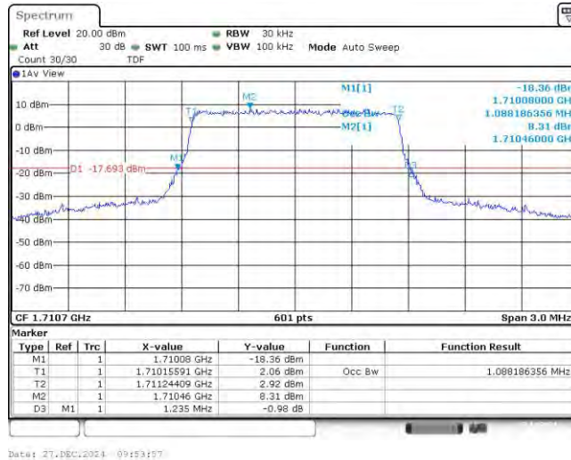
Band66-1.4MHz-16QAM-132322-6RB#0
