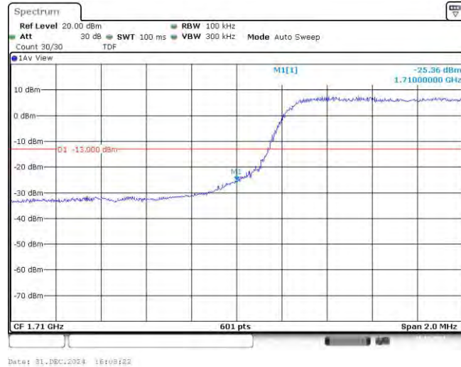
Band66-5MHz-QPSK-132647-25RB#0
