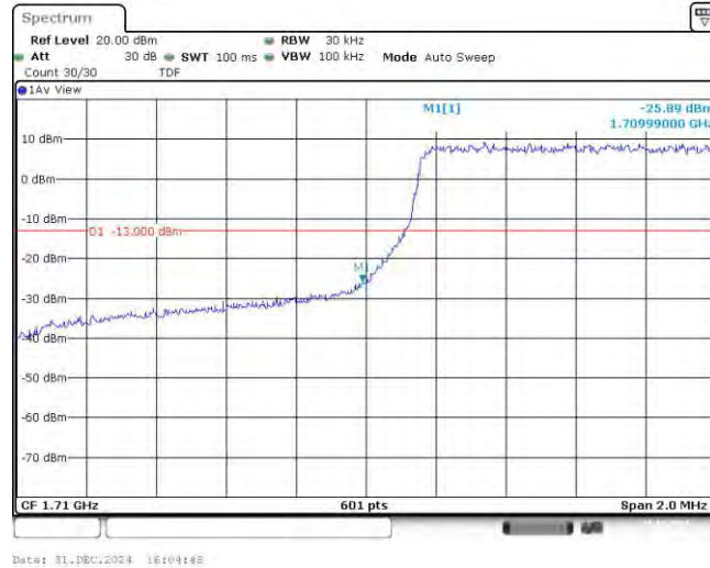
Band66-1.4MHz-16QAM-132665-6RB#0
