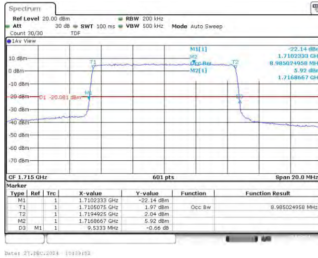
Band66-10MHz-QPSK-132322-50RB#0
