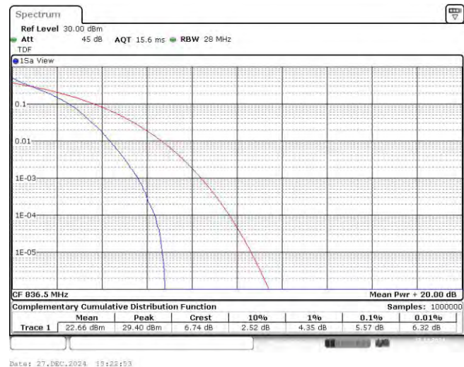
Band26-1.4MHz-QPSK-27033-6RB#0
