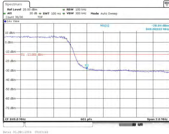
Band26-10MHz-QPSK-26840-50RB#0
