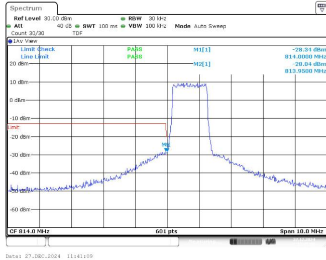
Band26-1.4MHz-16QAM-26783-6RB#0
