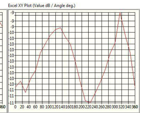
2.45GHz@Theta 0.0 Total
