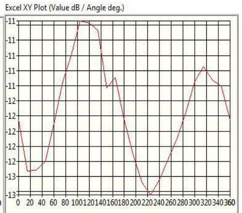
2.485GHz@Theta 0.0 Total
