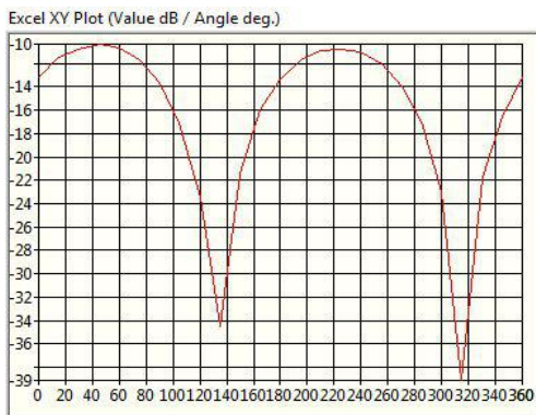
2.45GHz@Theta 0.0 Horizontal
