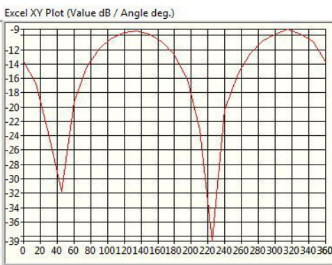
2.45GHz@Theta 0.0 Vertical
