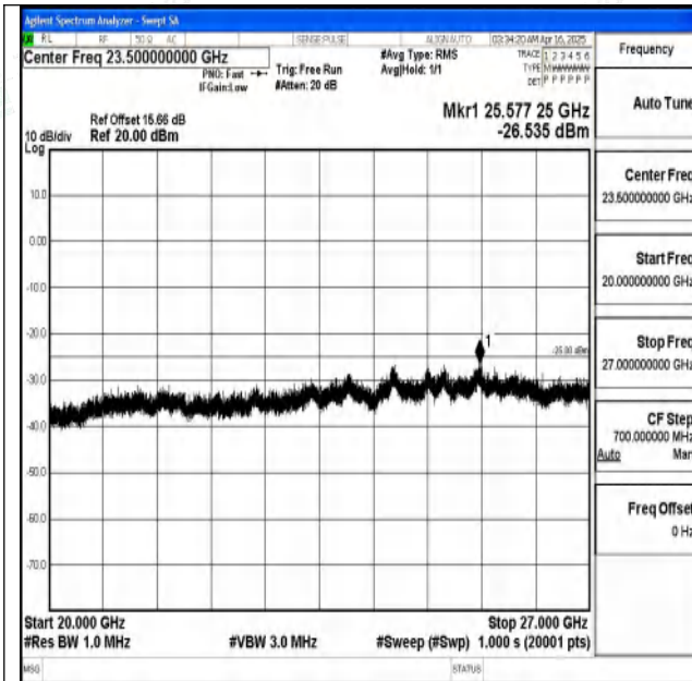
Band7_10MHz_QPSK_21100_1RB#0_20000~27000_2000~27000
