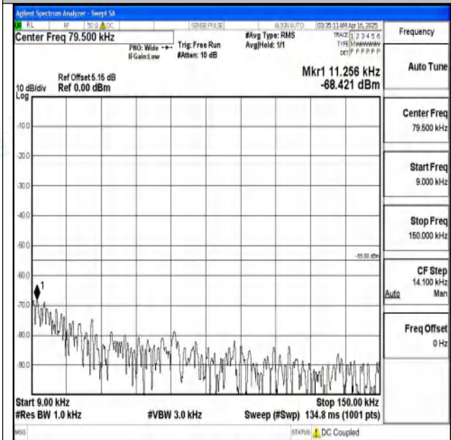
Band7_10MHz_QPSK_21400_1RB#0_0.009~0.15_0.009 ~0.15
