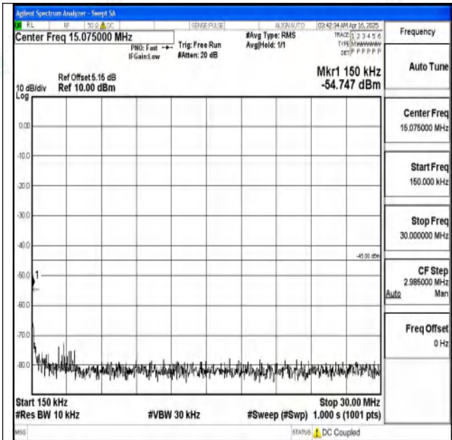
Band7_20MHz_16QAM_20850_1RB#0_0.15~30_0.15~30
