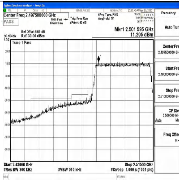
Band7_15MHz_16QAM_20825_75RB#0
