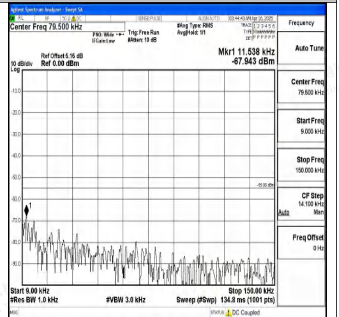
Band7_20MHz_16QAM_21350_1RB#0_0.009~0.15_0.009~0.15
