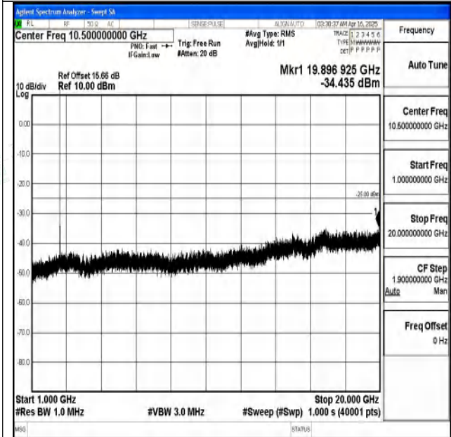
Band7_5MHz_16QAM_21100_1RB#0_1000~20000_1000 ~20000
