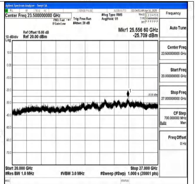
Band7_10MHz_16QAM_21100_1RB#0_20000~27000_200 00~27000
