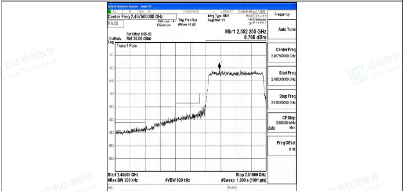
Band7_10MHz_16QAM_20800_50RB#0
