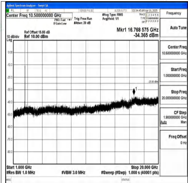
Band7_10MHz_16QAM_21100_1RB#0_1000~20000_100 0~20000
