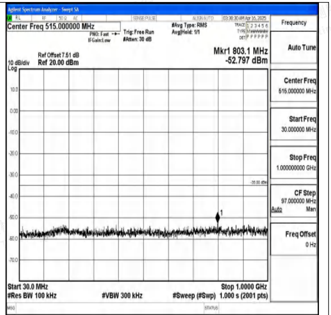
Band7_5MHz_16QAM_21100_1RB#0_30~1000_30~1000
