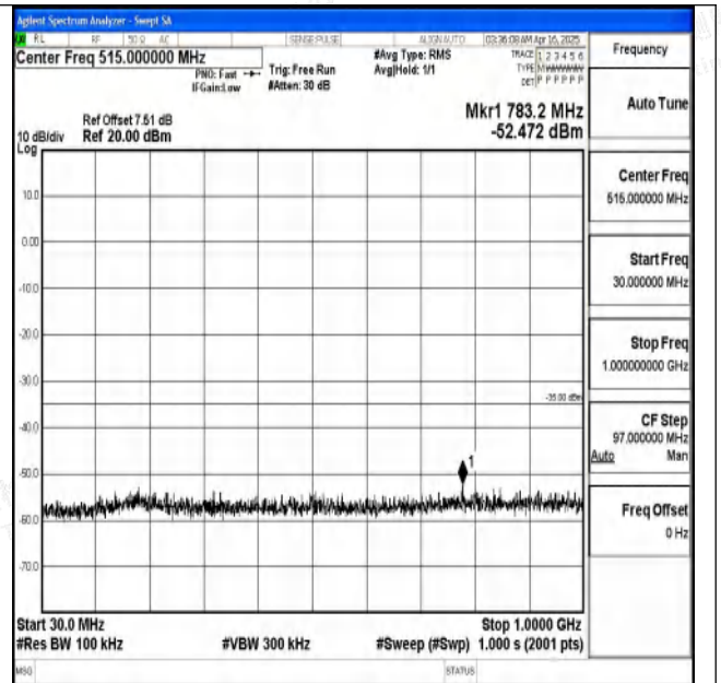
Band7_10MHz_16QAM_21400_1RB#0_30~1000_30~100 0
