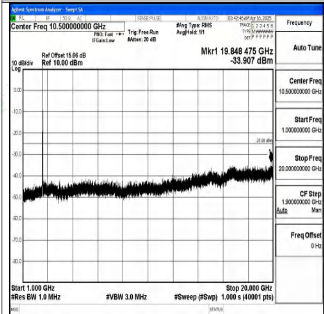
Band7_20MHz_16QAM_20850_1RB#0_1000~20000_100 0~20000
