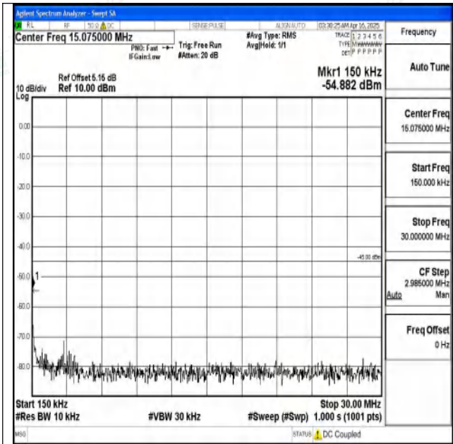
Band7_5MHz_16QAM_21100_1RB#0_0.15~30_0.15~30
