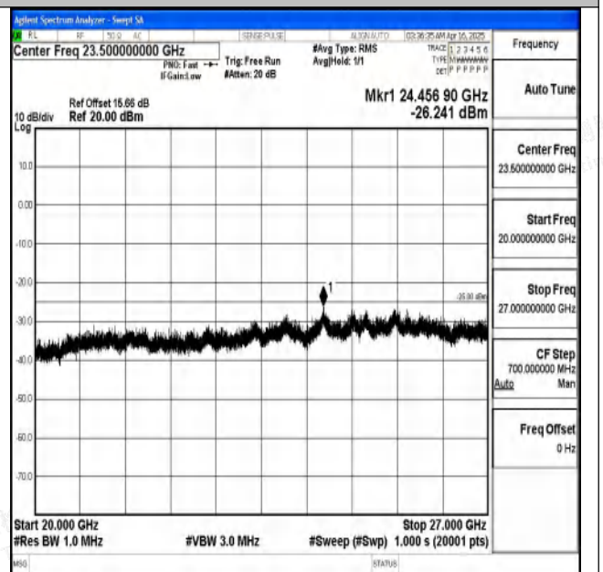
Band7_10MHz_16QAM_21400_1RB#0_20000~27000_200 00~27000
