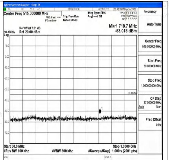
Band7_20MHz_16QAM_20850_1RB#0_30~1000_30~100
