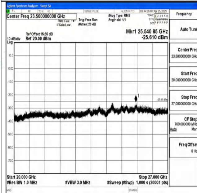
Band7_20MHz_QPSK_21350_1RB#0_20000~27000_20000~27000
