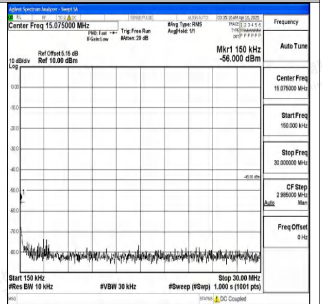
Band7_10MHz_QPSK_21400_1RB#0_0.15~30_0.15~30
