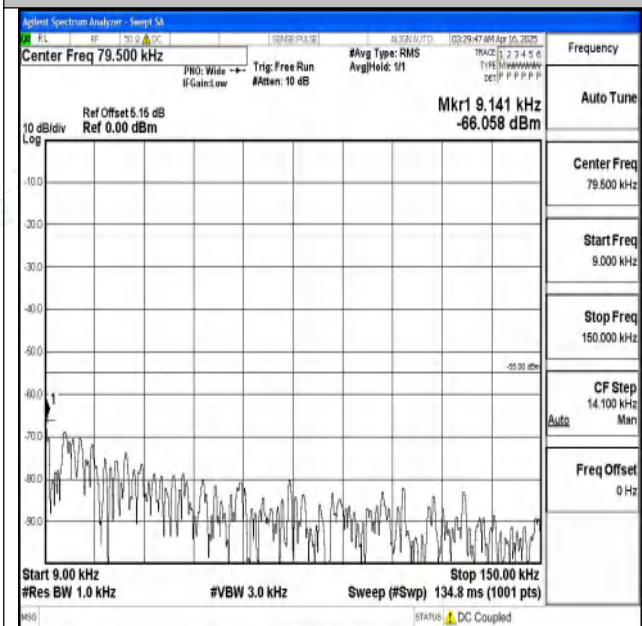
Band7_5MHz_QPSK_21100_1RB#0_0.009~0.15_0.009~ 0.15
