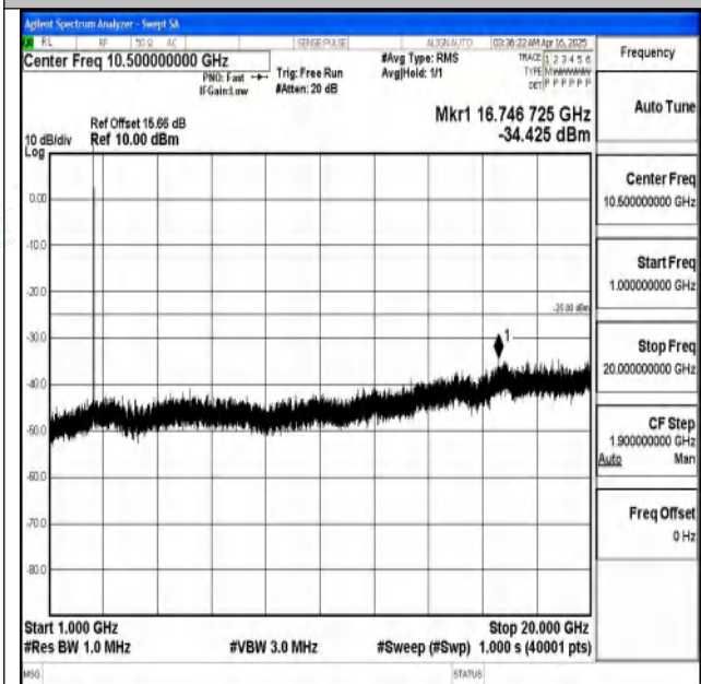
Band7_10MHz_16QAM_21400_1RB#0_1000~20000_100 0~20000
