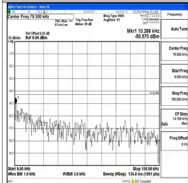
Band2-10MHz-QPSK-19150-1RB#0-0.009~0.15-PASS
