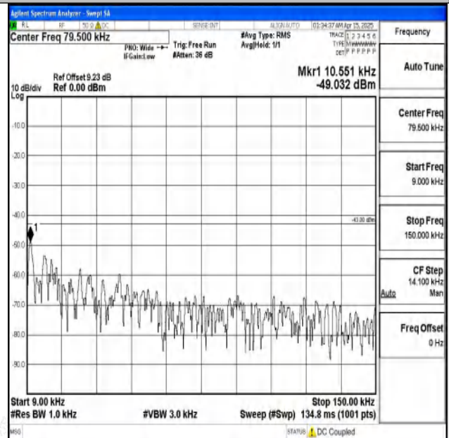
Band2-15MHz-16QAM-18900-1RB#0-0.009~0.15-PASS
