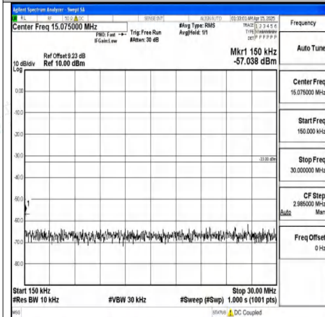
Band2-15MHz-16QAM-18675-1RB#0-0.15~30-PASS
