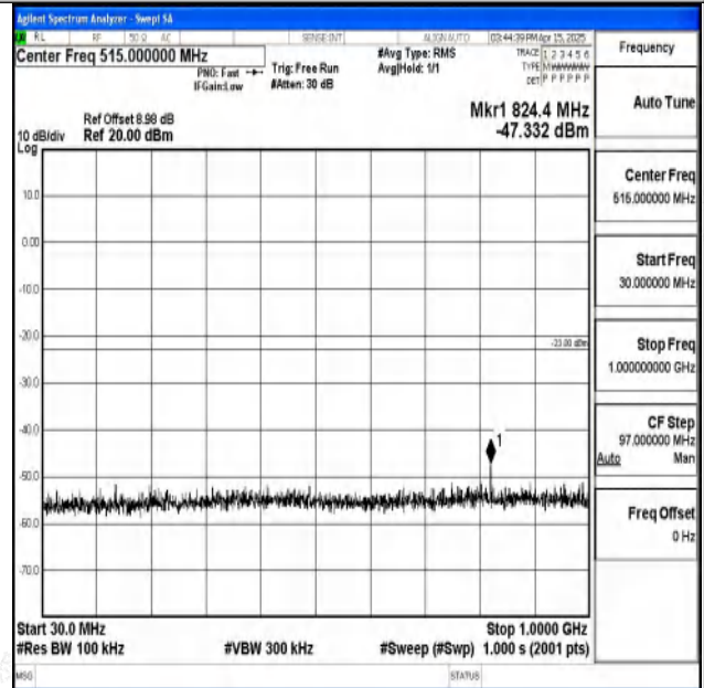
Band2-1.4MHz-16QAM-18607-1RB#0-30~1000-PASS
