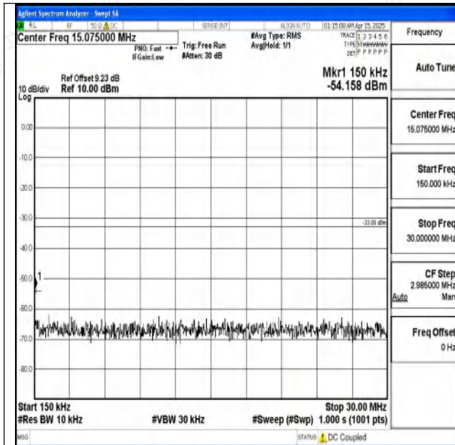
Band2-3MHz-16QAM-18615-1RB#0-0.15~30-PASS
