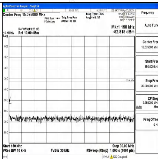
Band2-20MHz-QPSK-18900-1RB#0-0.15~30-PASS
