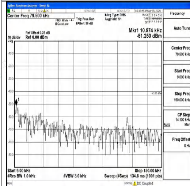
Band2-15MHz-QPSK-18900-1RB#0-0.009~0.15-PASS
