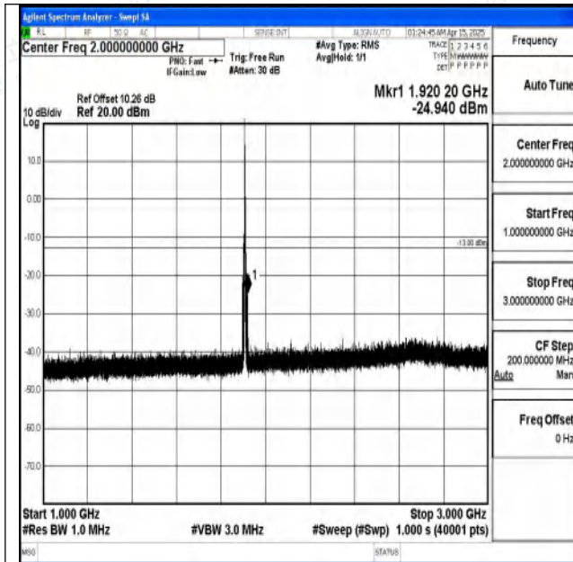
Band2-5MHz-16QAM-19175-1RB#0-1000~3000-PASS
