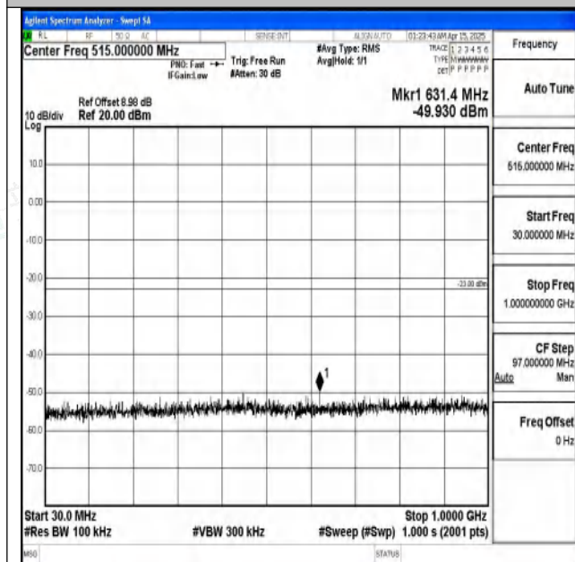
Band2-5MHz-QPSK-19175-1RB#0-30~1000-PASS
