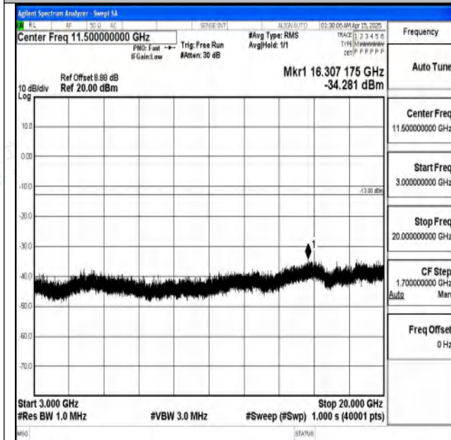
Band2-10MHz-QPSK-19150-1RB#0-3000~20000-PASS
