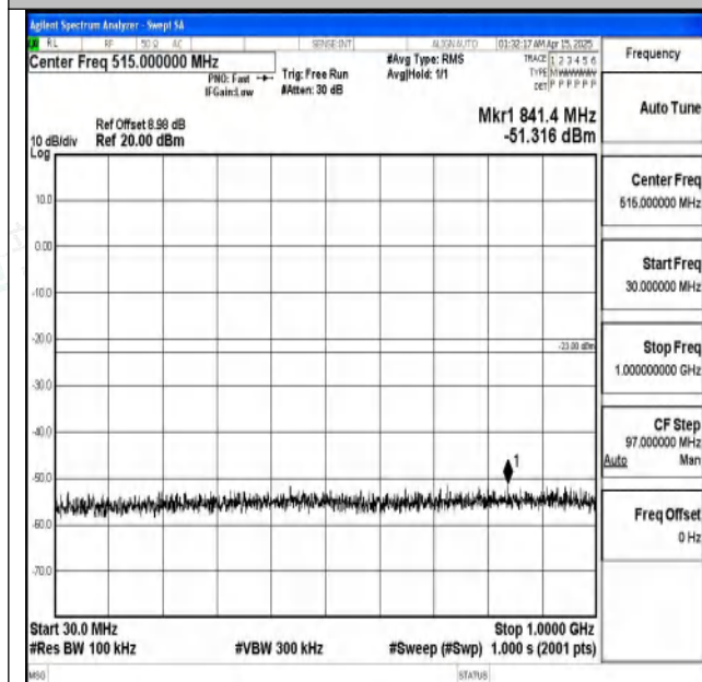
Band2-15MHz-QPSK-18675-1RB#0-30~1000-PASS
