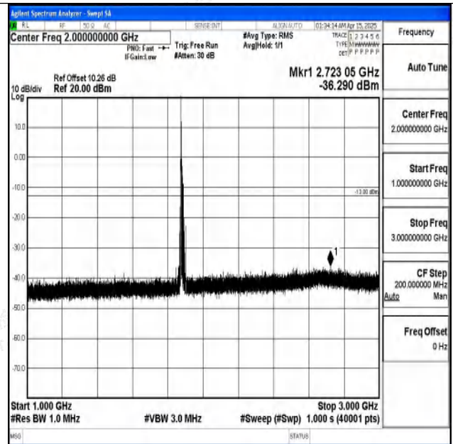
Band2-15MHz-QPSK-18900-1RB#0-1000~3000-PASS
