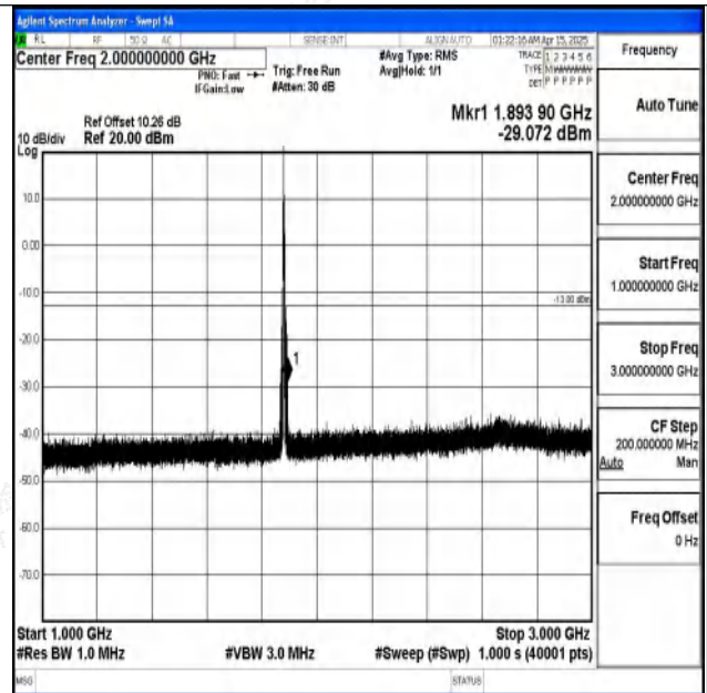
Band2-5MHz-QPSK-18900-1RB#0-1000~3000-PASS
