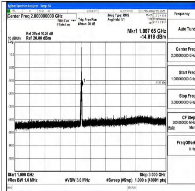
Band2-3MHz-16QAM-18900-1RB#0-1000~3000-PASS
