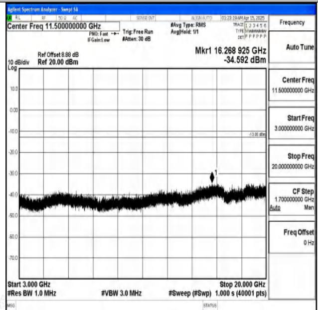
Band2-5MHz-16QAM-18900-1RB#0-3000~20000-PASS
