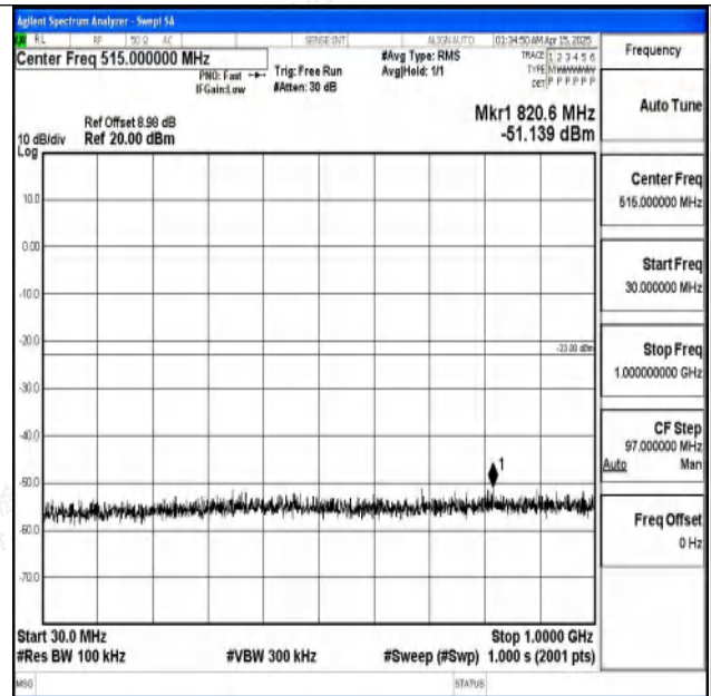
Band2-15MHz-16QAM-18900-1RB#0-30~1000-PASS
