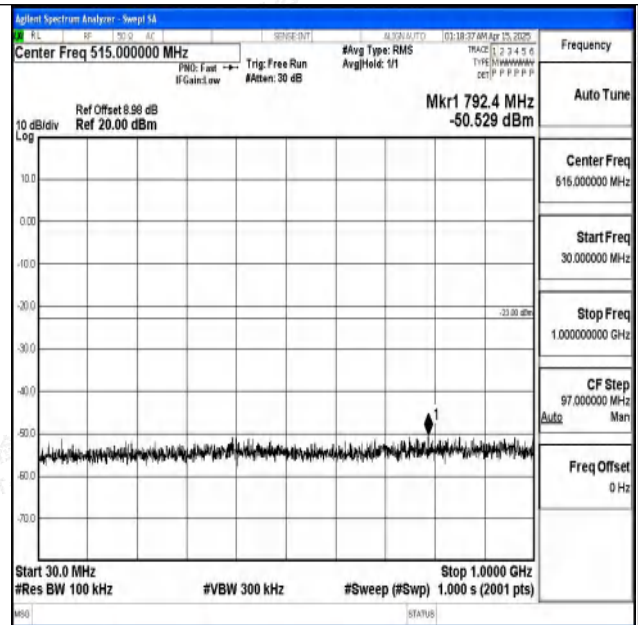
Band2-3MHz-16QAM-19185-1RB#0-30~1000-PASS
