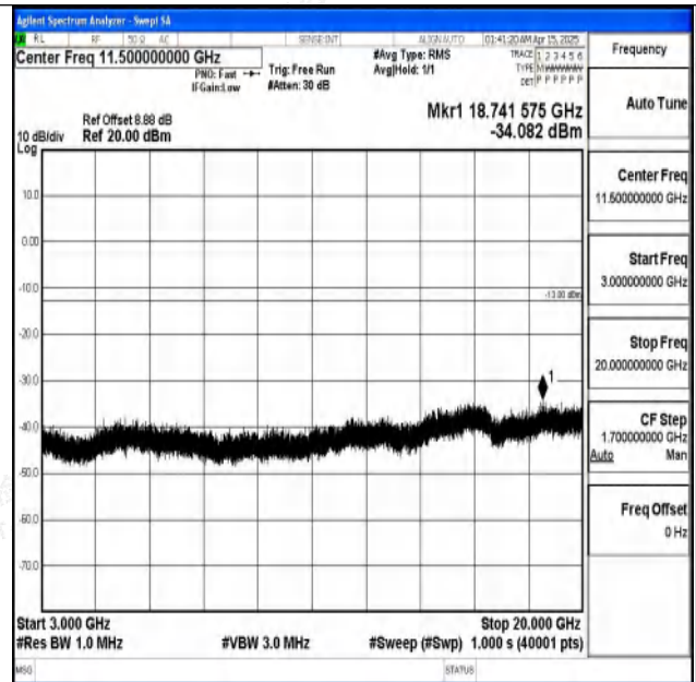
Band2-20MHz-16QAM-18900-1RB#0-3000~20000-PASS
