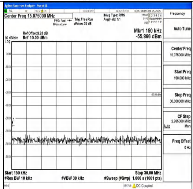
Band2-1.4MHz-QPSK-19193-1RB#0-0.15~30-PASS
