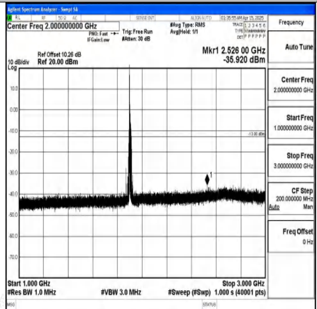
Band2-15MHz-QPSK-19125-1RB#0-1000~3000-PASS
