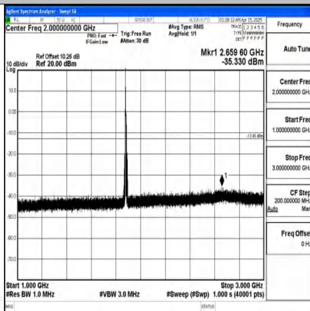
Band2-10MHz-QPSK-18900-1RB#0-1000~3000-PASS
