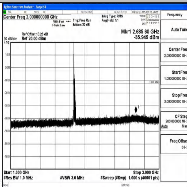
Band2-15MHz-QPSK-18675-1RB#0-1000~3000-PASS
