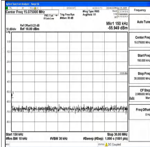
Band2-1.4MHz-16QAM-18607-1RB#0-0.15~30-PASS
