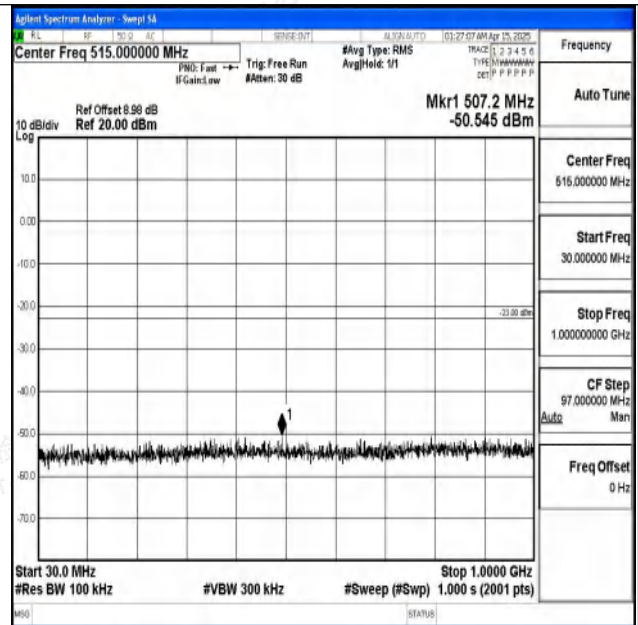
Band2-10MHz-16QAM-18650-1RB#0-30~1000-PASS
