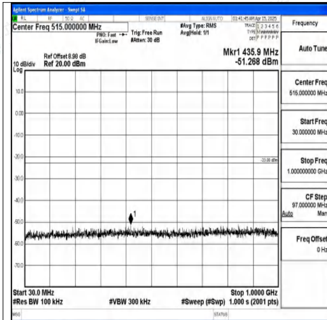
Band2-20MHz-QPSK-19100-1RB#0-30~1000-PASS
