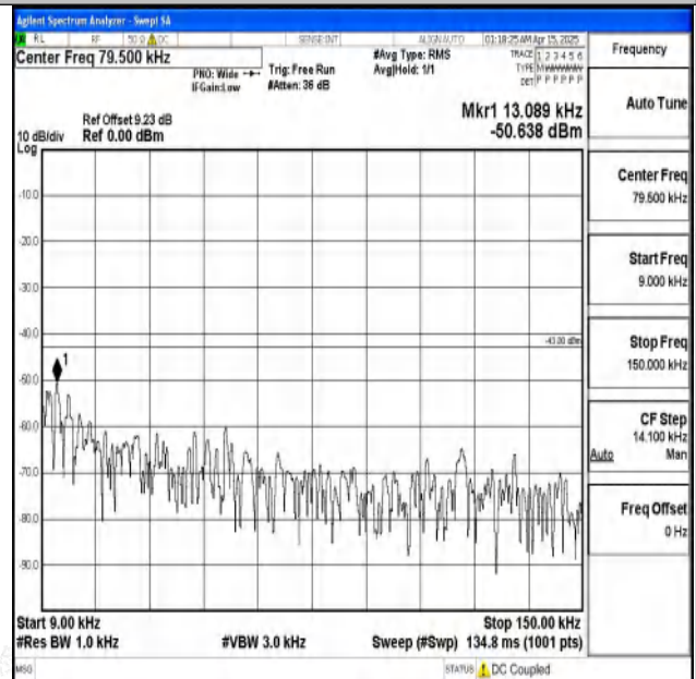
Band2-3MHz-16QAM-19185-1RB#0-0.009~0.15-PASS
