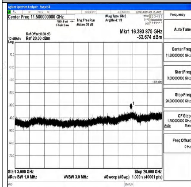
Band2-1.4MHz-16QAM-19193-1RB#0-3000~20000-PASS
