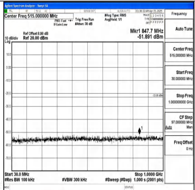
Band2-15MHz-16QAM-19125-1RB#0-30~1000-PASS
