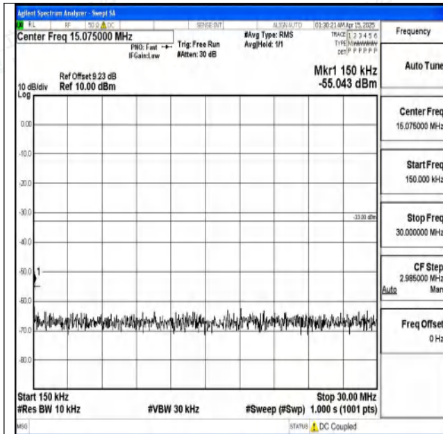
Band2-10MHz-16QAM-19150-1RB#0-0.15~30-PASS
