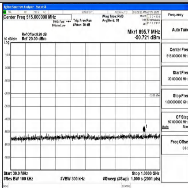
Band2-5MHz-16QAM-18625-1RB#0-30~1000-PASS
