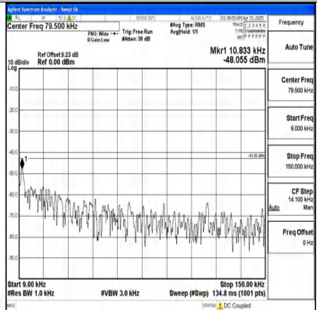
Band2-20MHz-16QAM-18700-1RB#0-0.009~0.15-PASS
