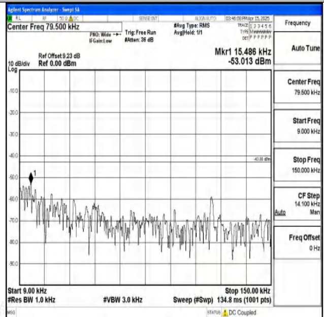
Band2-1.4MHz-16QAM-18900-1RB#0-0.009~0.15-PASS
