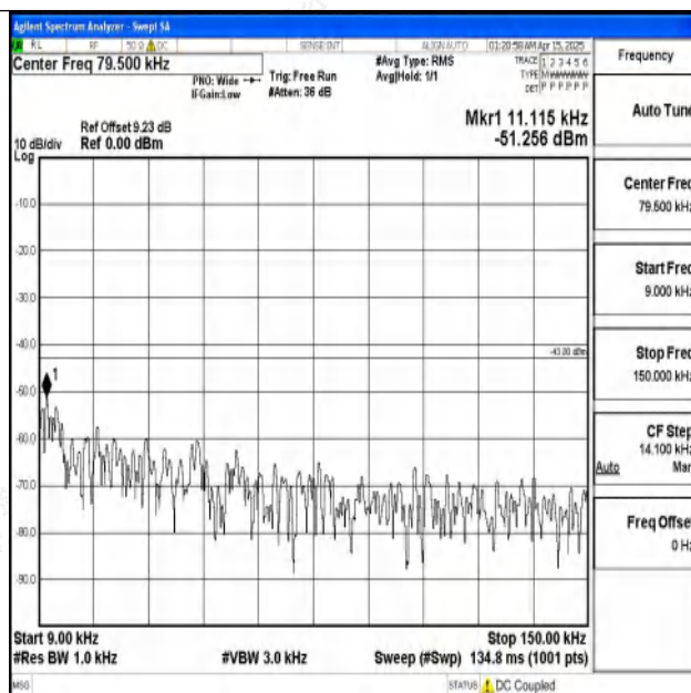
Band2-5MHz-16QAM-18625-1RB#0-0.009~0.15-PASS
