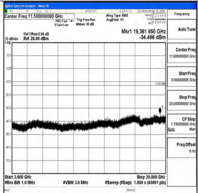
Band2-20MHz-16QAM-19100-1RB#0-3000~20000-PASS
