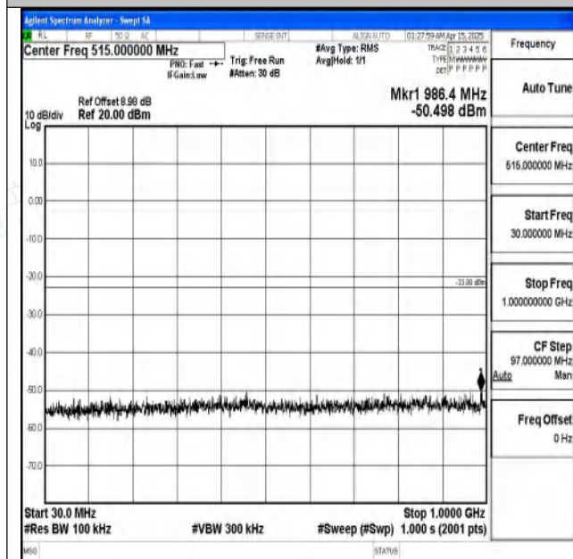
Band2-10MHz-QPSK-18900-1RB#0-30~1000-PASS
