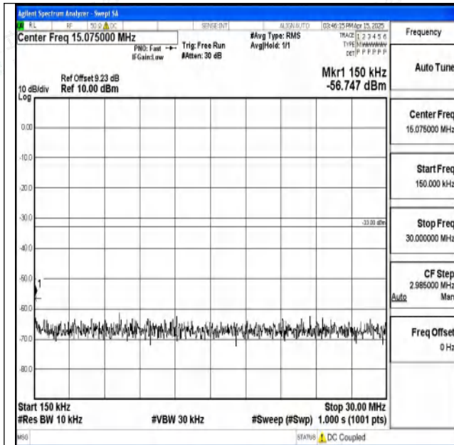
Band2-1.4MHz-16QAM-18900-1RB#0-0.15~30-PASS
