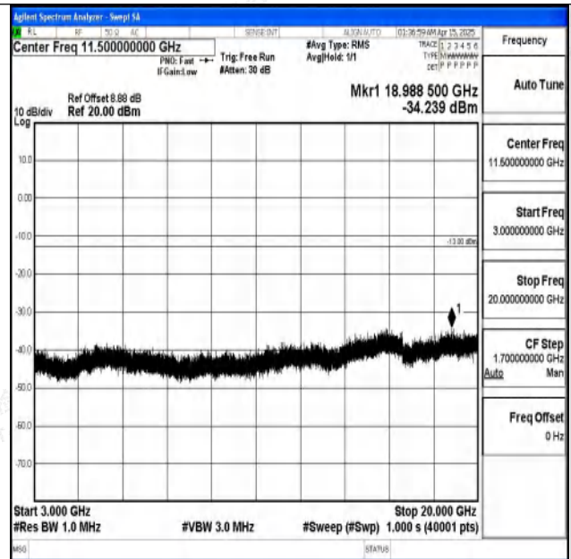
Band2-15MHz-16QAM-19125-1RB#0-3000~20000-PASS
