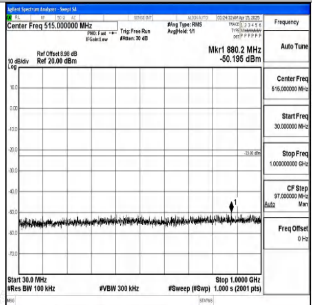
Band2-5MHz-16QAM-19175-1RB#0-30~1000-PASS
