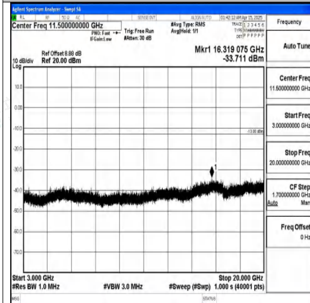
Band2-20MHz-QPSK-19100-1RB#0-3000~20000-PASS
