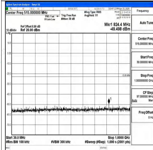
Band2-1.4MHz-QPSK-19193-1RB#0-30~1000-PASS
