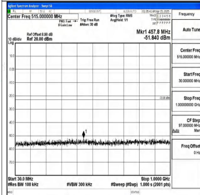
Band2-15MHz-QPSK-19125-1RB#0-30~1000-PASS
