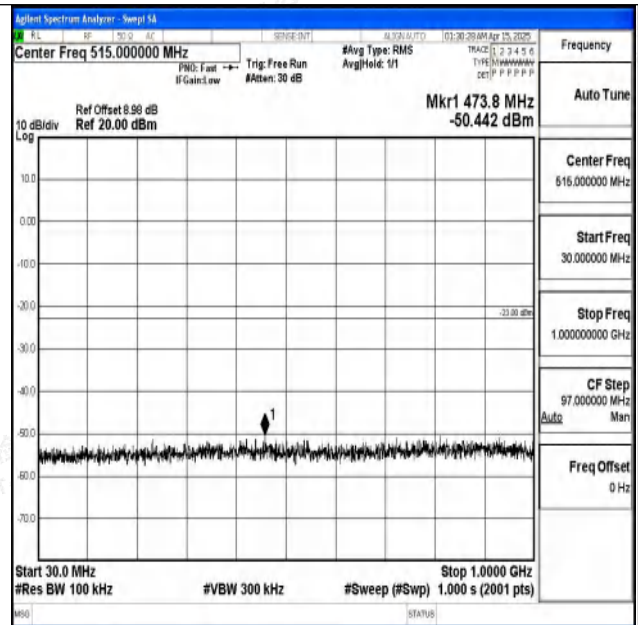
Band2-10MHz-16QAM-19150-1RB#0-30~1000-PASS
