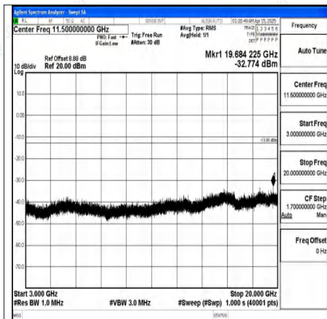
Band2-5MHz-QPSK-18625-1RB#0-3000~20000-PASS
