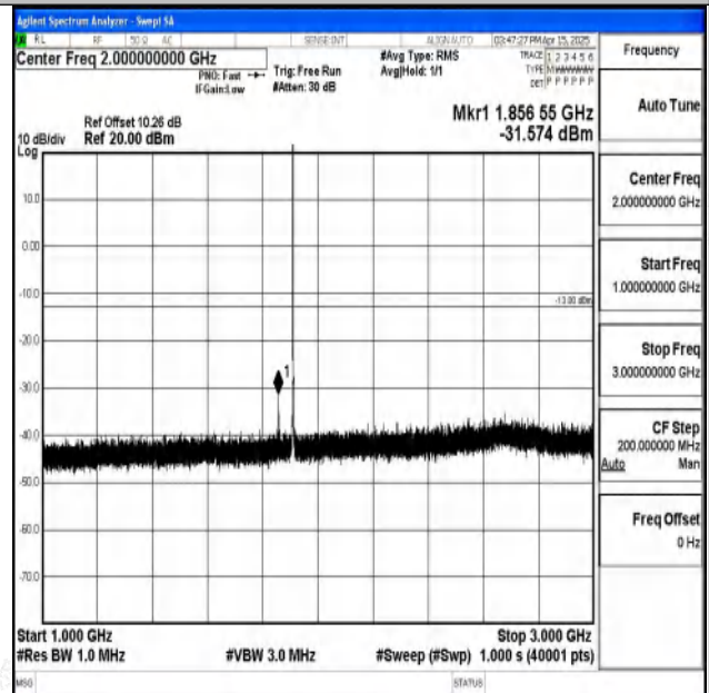
Band2-1.4MHz-QPSK-19193-1RB#0-1000~3000-PASS
