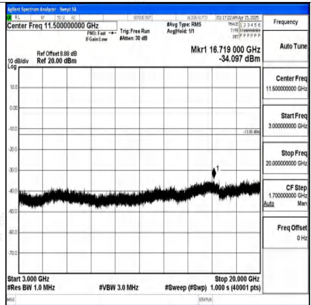
Band2-3MHz-16QAM-18900-1RB#0-3000~20000-PASS
