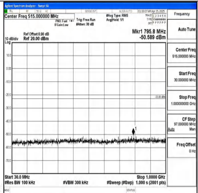
Band2-15MHz-16QAM-18675-1RB#0-30~1000-PASS
