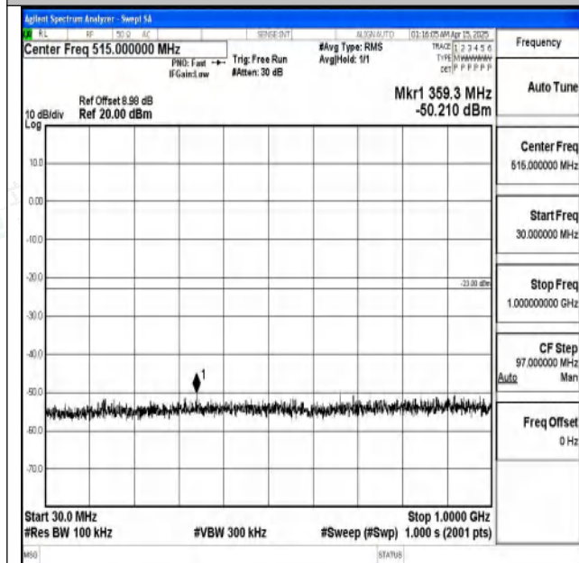
Band2-3MHz-QPSK-18900-1RB#0-30~1000-PASS
