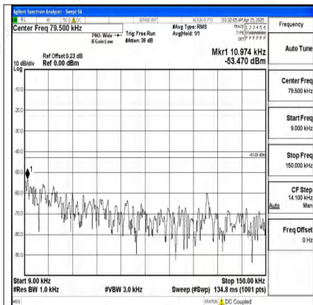
Band2-15MHz-QPSK-18675-1RB#0-0.009~0.15-PASS
