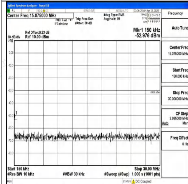
Band2-15MHz-16QAM-19125-1RB#0-0.15~30-PASS
