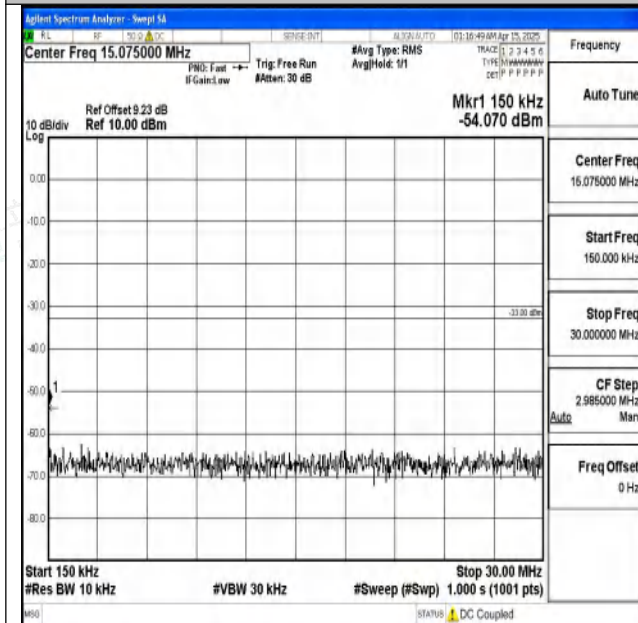
Band2-3MHz-16QAM-18900-1RB#0-0.15~30-PASS
