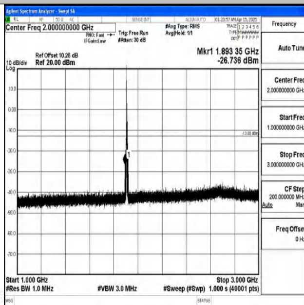
Band2-5MHz-QPSK-19175-1RB#0-1000~3000-PASS
