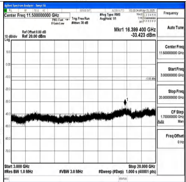
Band2-15MHz-16QAM-18675-1RB#0-3000~20000-PASS
