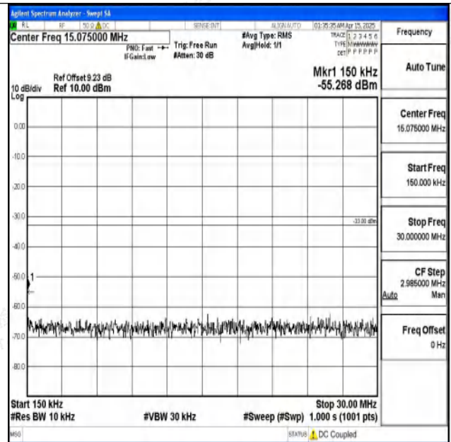
Band2-15MHz-QPSK-19125-1RB#0-0.15~30-PASS
