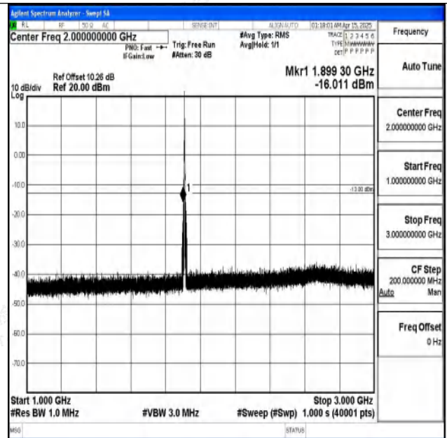
Band2-3MHz-QPSK-19185-1RB#0-1000~3000-PASS
