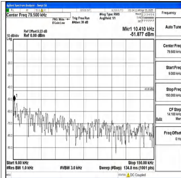
Band2-3MHz-QPSK-18615-1RB#0-0.009~0.15-PASS
