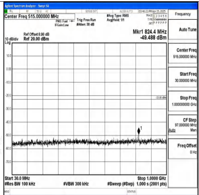
Band2-1.4MHz-16QAM-18900-1RB#0-30~1000-PASS
