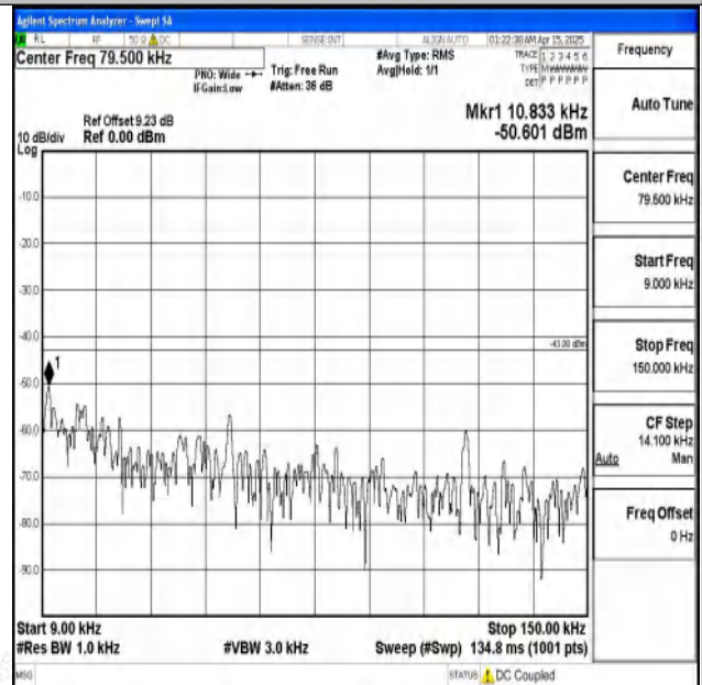
Band2-5MHz-16QAM-18900-1RB#0-0.009~0.15-PASS
