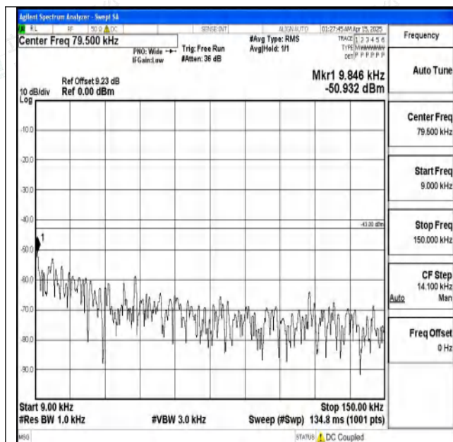
Band2-10MHz-QPSK-18900-1RB#0-0.009~0.15-PASS
