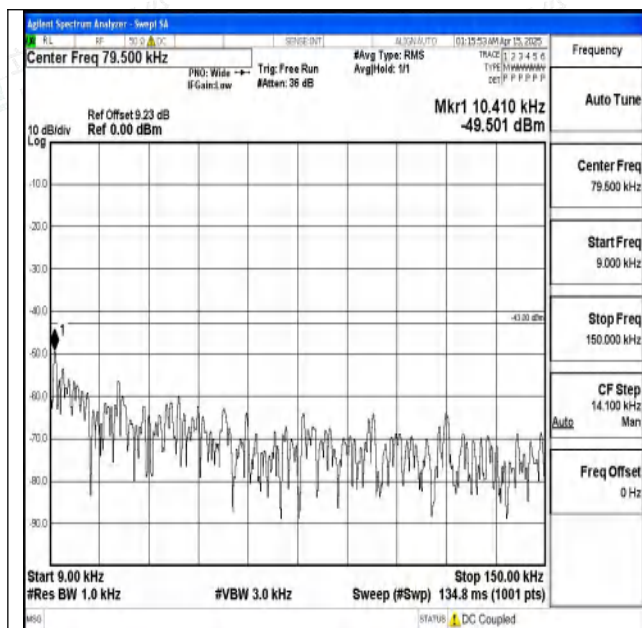
Band2-3MHz-QPSK-18900-1RB#0-0.009~0.15-PASS
