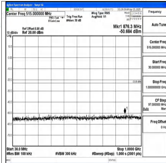
Band2-10MHz-QPSK-19150-1RB#0-30~1000-PASS
