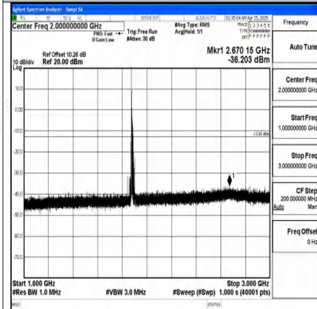
Band2-15MHz-16QAM-18900-1RB#0-1000~3000-PASS
