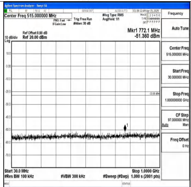
Band2-20MHz-16QAM-18700-1RB#0-30~1000-PASS
