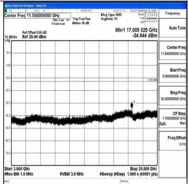
Band2-10MHz-16QAM-18650-1RB#0-3000~20000-PASS
