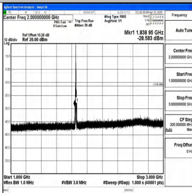
Band2-5MHz-QPSK-18625-1RB#0-1000~3000-PASS
