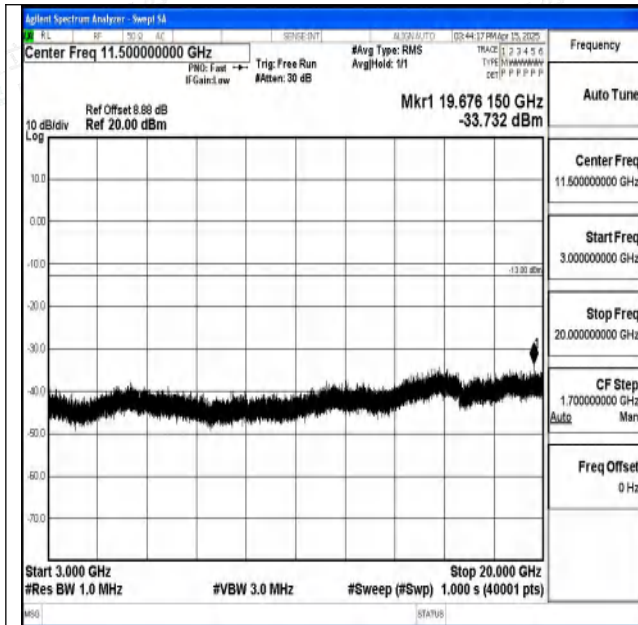
Band2-1.4MHz-QPSK-18607-1RB#0-3000~20000-PASS
