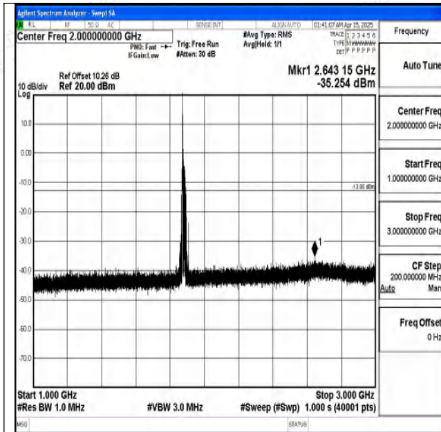
Band2-20MHz-16QAM-18900-1RB#0-1000~3000-PASS
