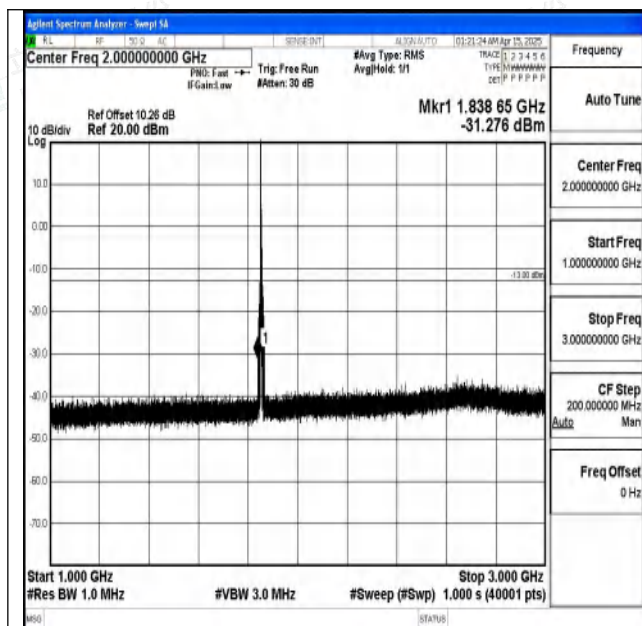
Band2-5MHz-16QAM-18625-1RB#0-1000~3000-PASS
