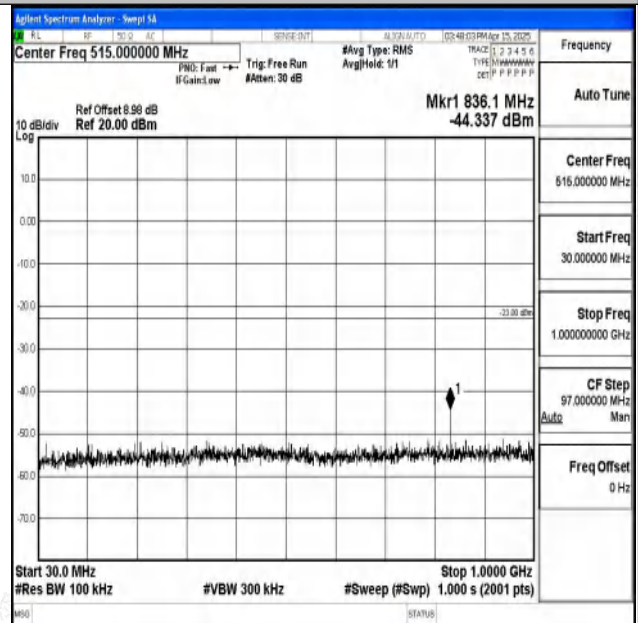
Band2-1.4MHz-16QAM-19193-1RB#0-30~1000-PASS
