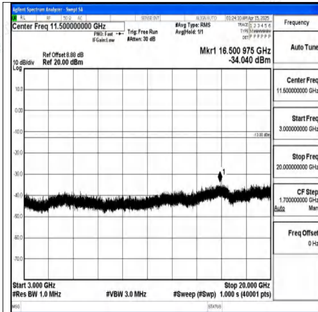
Band2-5MHz-QPSK-19175-1RB#0-3000~20000-PASS
