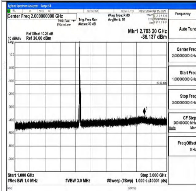
Band2-10MHz-16QAM-18650-1RB#0-1000~3000-PASS
