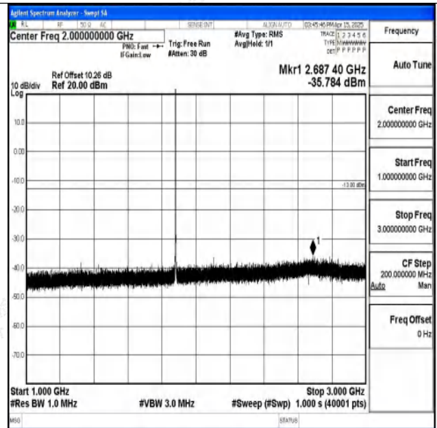
Band2-1.4MHz-QPSK-18900-1RB#0-1000~3000-PASS
