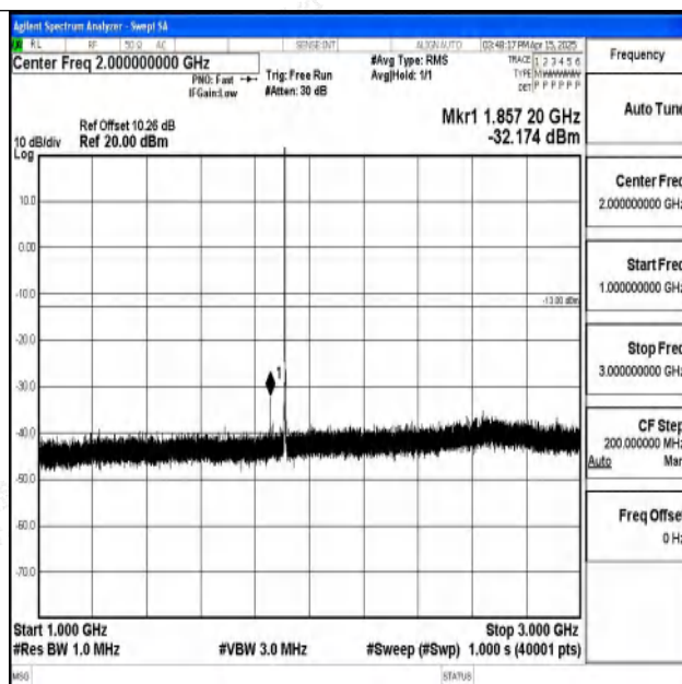
Band2-1.4MHz-16QAM-19193-1RB#0-1000~3000-PASS
