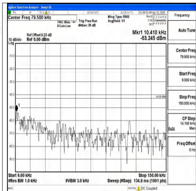
Band2-20MHz-QPSK-18900-1RB#0-0.009~0.15-PASS
