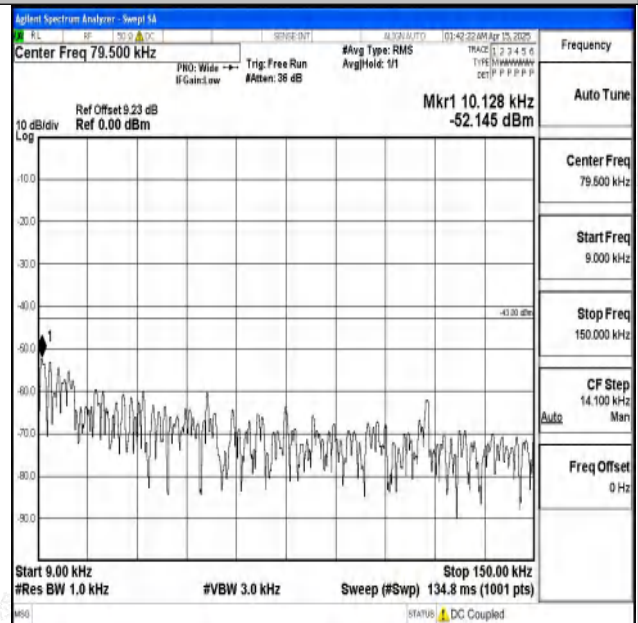
Band2-20MHz-16QAM-19100-1RB#0-0.009~0.15-PASS
