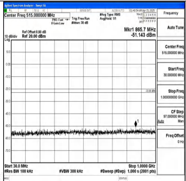
Band2-20MHz-16QAM-18900-1RB#0-30~1000-PASS
