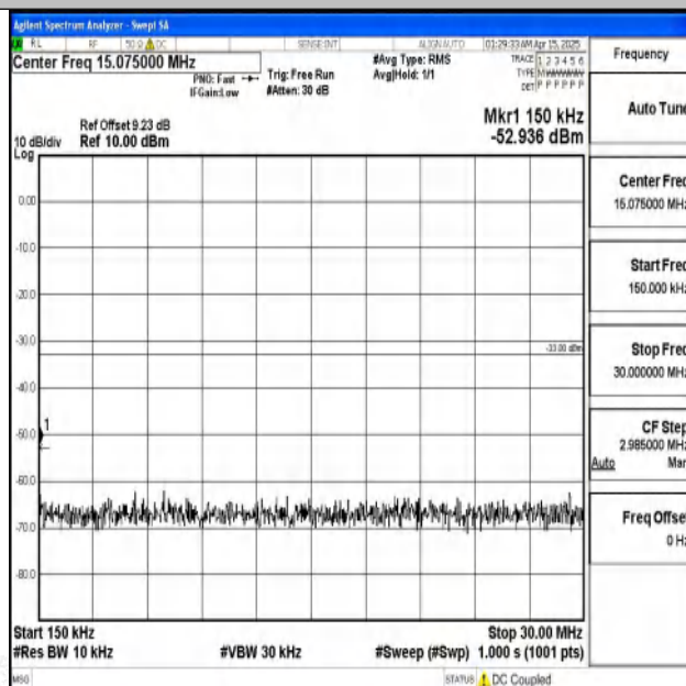
Band2-10MHz-QPSK-19150-1RB#0-0.15~30-PASS
