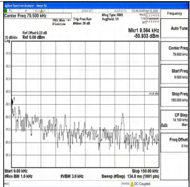
Band2-15MHz-16QAM-19125-1RB#0-0.009~0.15-PASS
