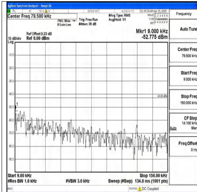
Band2-15MHz-QPSK-19125-1RB#0-0.009~0.15-PASS
