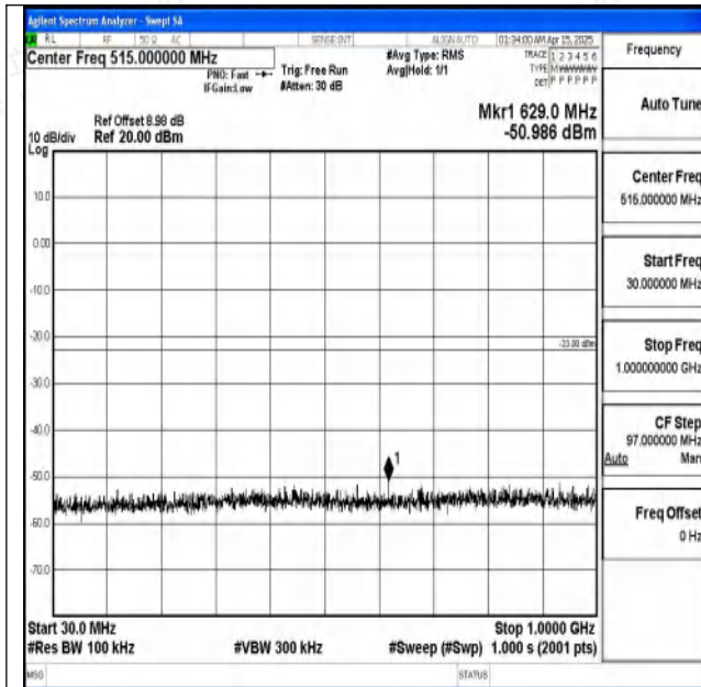
Band2-15MHz-QPSK-18900-1RB#0-30~1000-PASS
