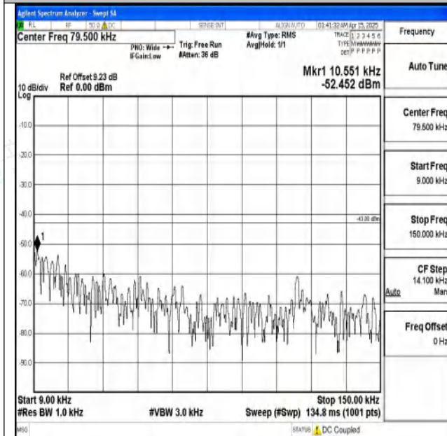
Band2-20MHz-QPSK-19100-1RB#0-0.009~0.15-PASS
