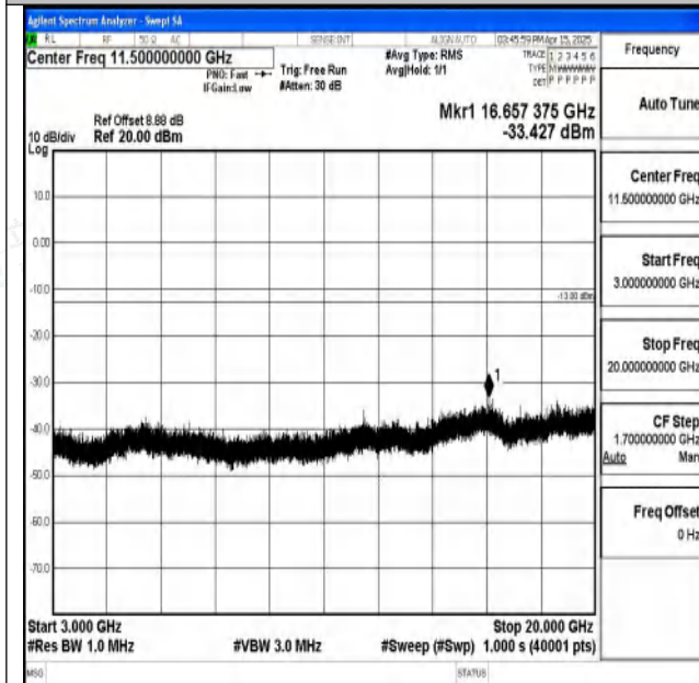
Band2-1.4MHz-QPSK-18900-1RB#0-3000~20000-PASS
