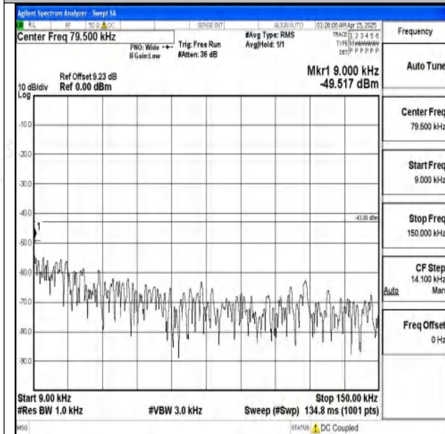
Band2-10MHz-QPSK-18650-1RB#0-0.009~0.15-PASS
