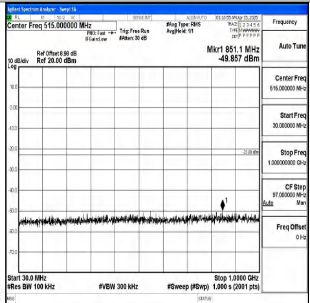
Band2-3MHz-16QAM-18900-1RB#0-30~1000-PASS
