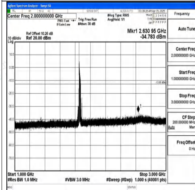
Band2-20MHz-16QAM-18700-1RB#0-1000~3000-PASS
