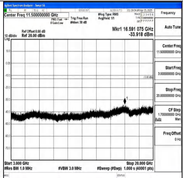
Band2-3MHz-16QAM-19185-1RB#0-3000~20000-PASS
