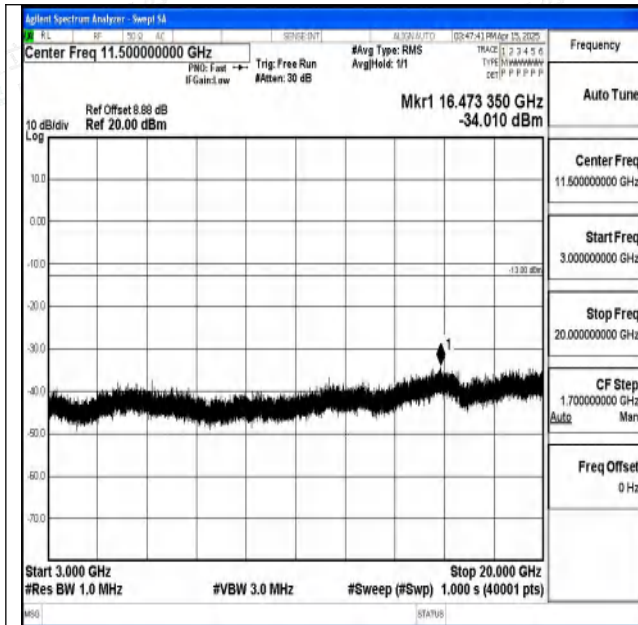
Band2-1.4MHz-QPSK-19193-1RB#0-3000~20000-PASS
