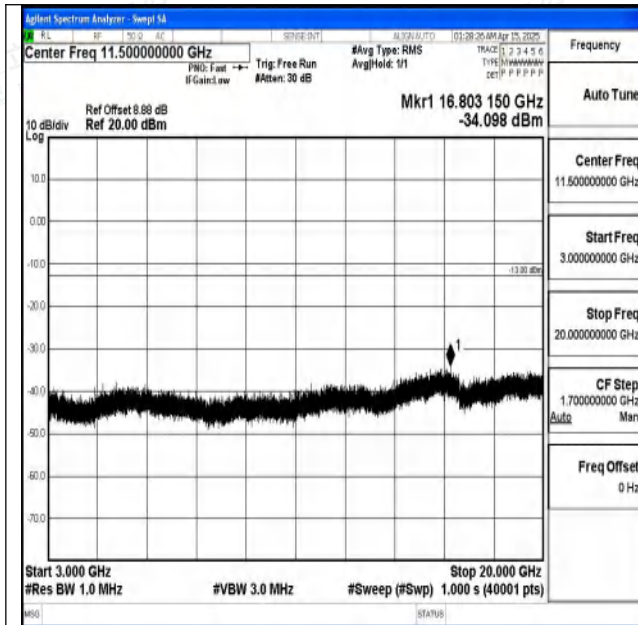
Band2-10MHz-QPSK-18900-1RB#0-3000~20000-PASS
