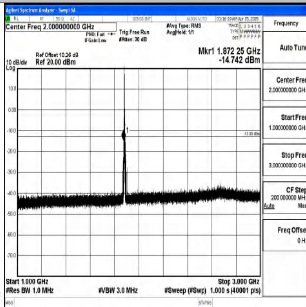
Band2-3MHz-QPSK-18900-1RB#0-1000~3000-PASS
