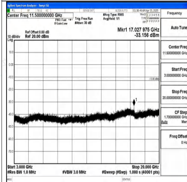
Band2-20MHz-QPSK-18700-1RB#0-3000~20000-PASS
