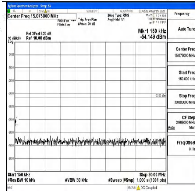
Band2-20MHz-16QAM-19100-1RB#0-0.15~30-PASS
