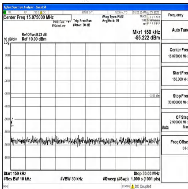
Band2-5MHz-QPSK-18625-1RB#0-0.15~30-PASS
