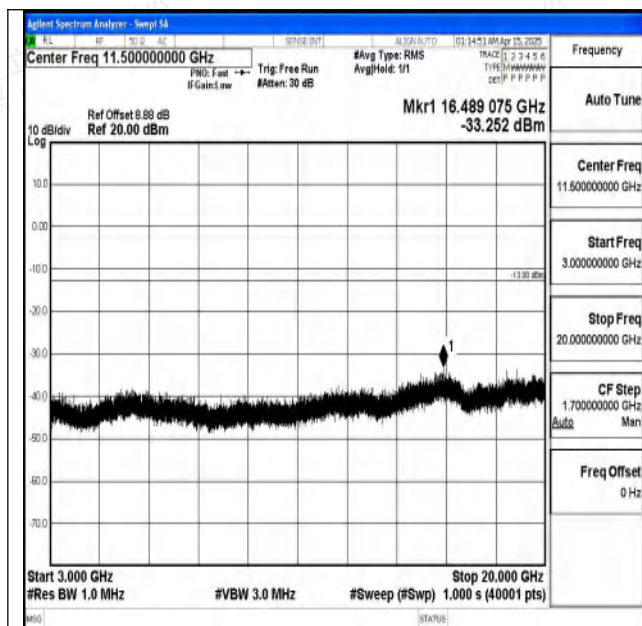
Band2-3MHz-QPSK-18615-1RB#0-3000~20000-PASS
