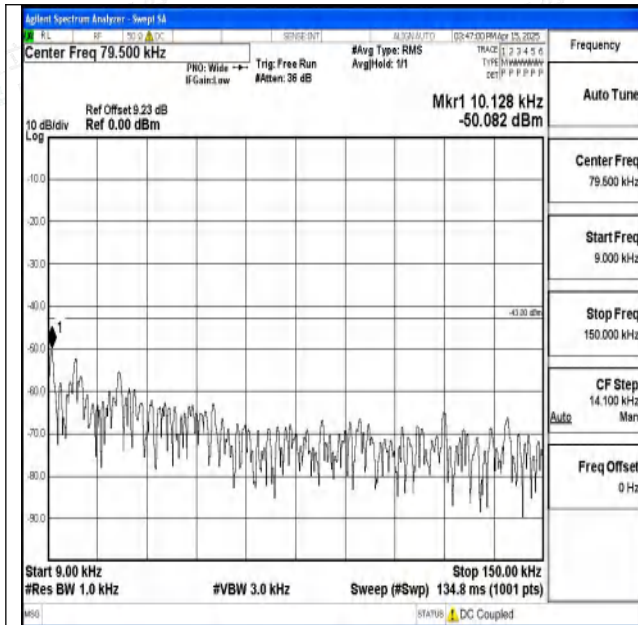
Band2-1.4MHz-QPSK-19193-1RB#0-0.009~0.15-PASS
