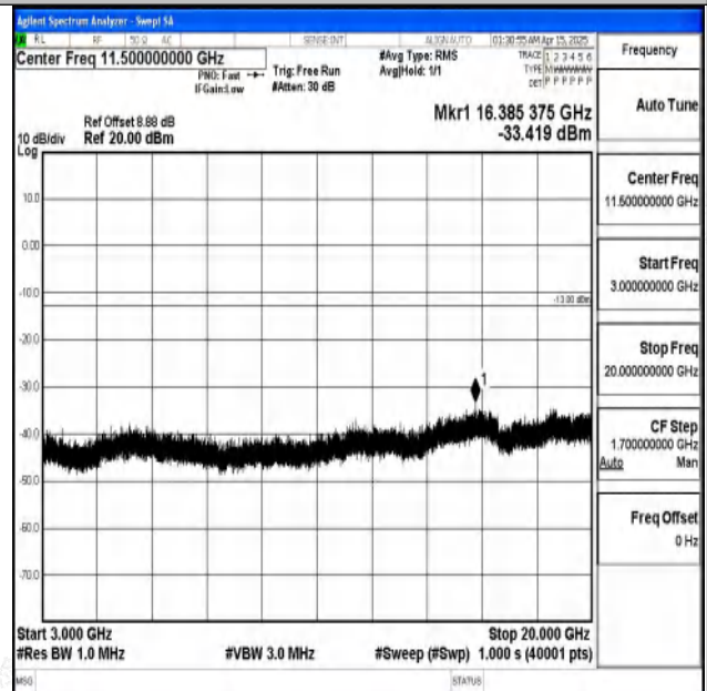
Band2-10MHz-16QAM-19150-1RB#0-3000~20000-PASS
