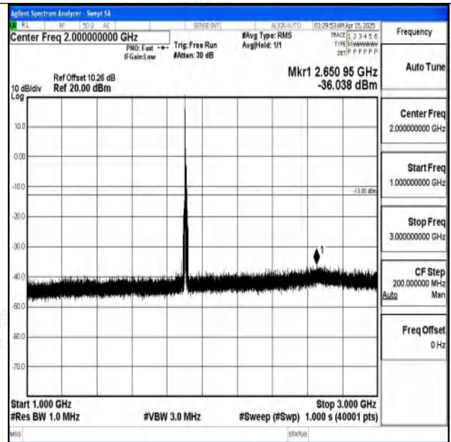
Band2-10MHz-QPSK-19150-1RB#0-1000~3000-PASS
