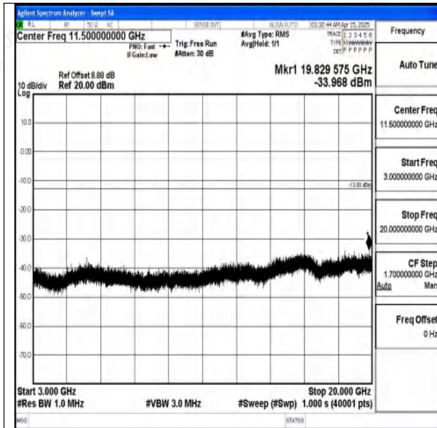
Band2-15MHz-QPSK-18675-1RB#0-3000~20000-PASS
