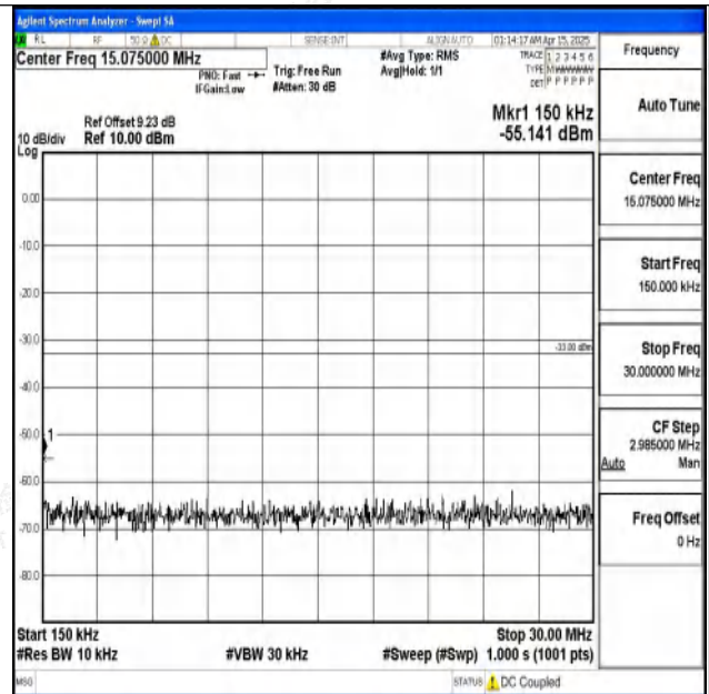
Band2-3MHz-QPSK-18615-1RB#0-0.15~30-PASS
