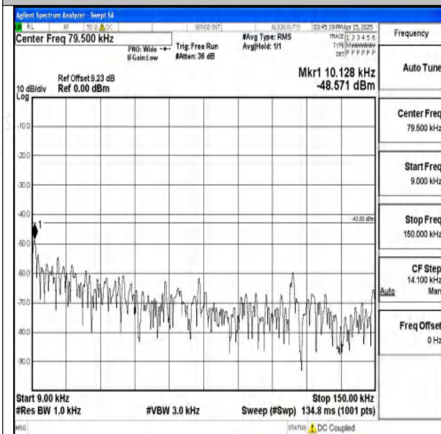
Band2-1.4MHz-QPSK-18900-1RB#0-0.009~0.15-PASS
