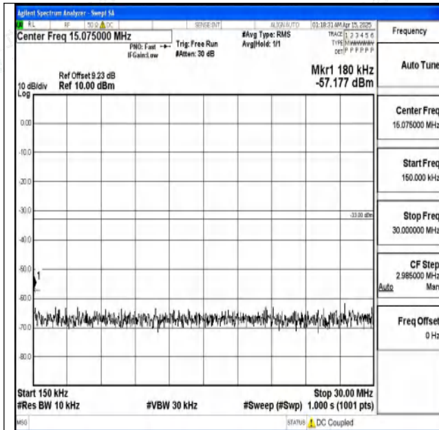
Band2-3MHz-16QAM-19185-1RB#0-0.15~30-PASS
