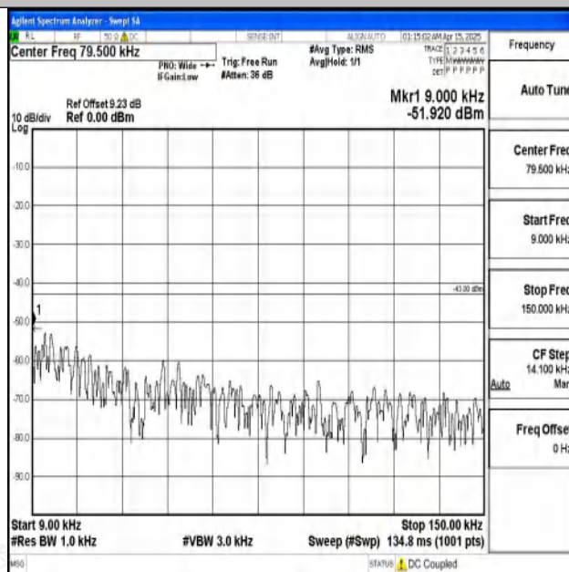
Band2-3MHz-16QAM-18615-1RB#0-0.009~0.15-PASS
