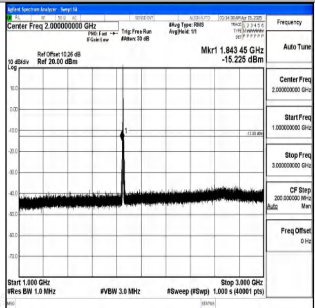
Band2-3MHz-QPSK-18615-1RB#0-1000~3000-PASS
