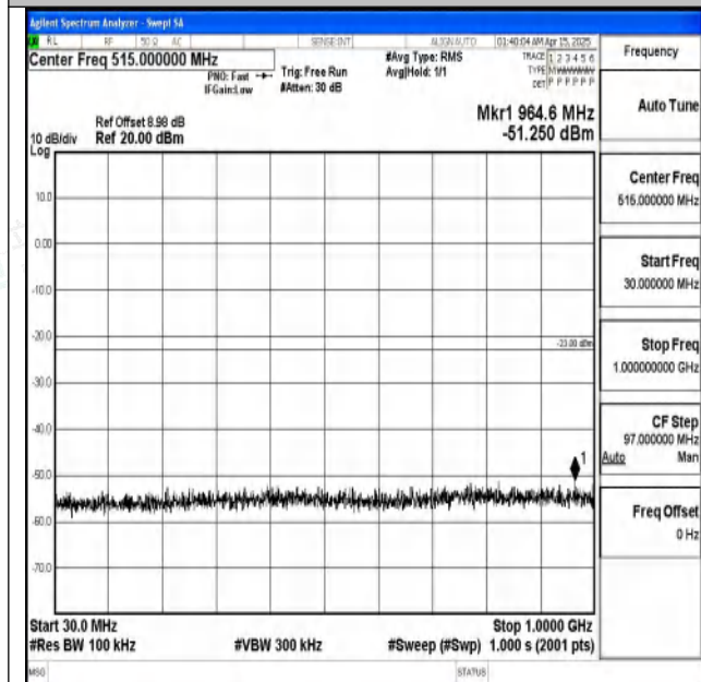
Band2-20MHz-QPSK-18900-1RB#0-30~1000-PASS
