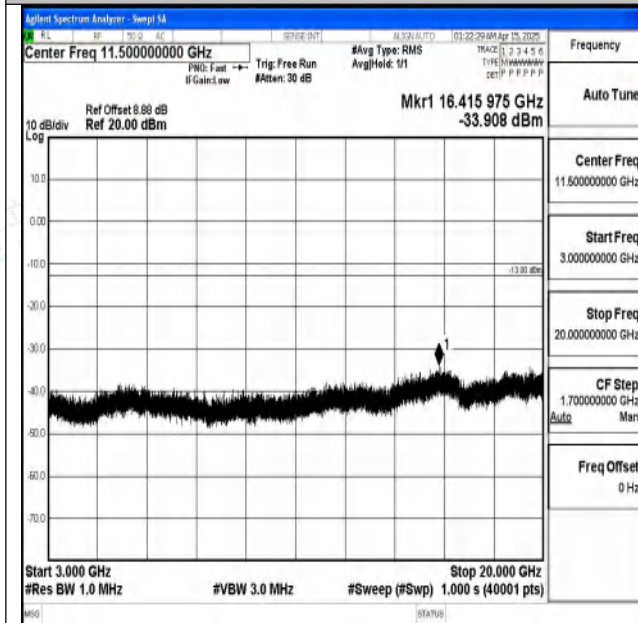
Band2-5MHz-QPSK-18900-1RB#0-3000~20000-PASS
