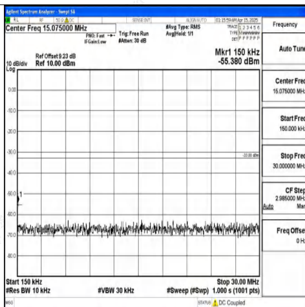
Band2-3MHz-QPSK-18900-1RB#0-0.15~30-PASS
