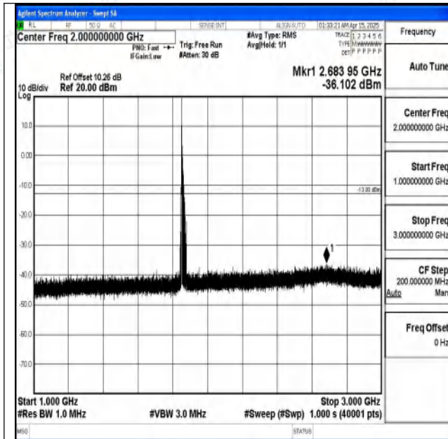
Band2-15MHz-16QAM-18675-1RB#0-1000~3000-PASS
