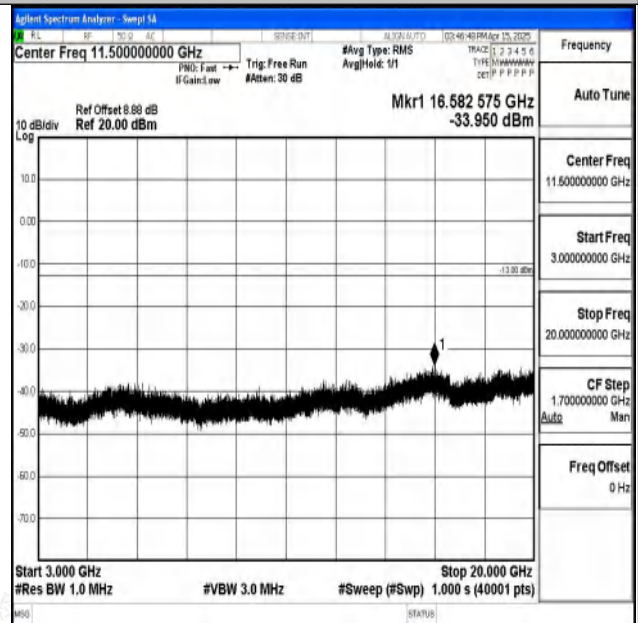
Band2-1.4MHz-16QAM-18900-1RB#0-3000~20000-PAS
