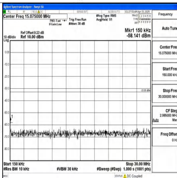
Band2-10MHz-QPSK-18900-1RB#0-0.15~30-PASS
