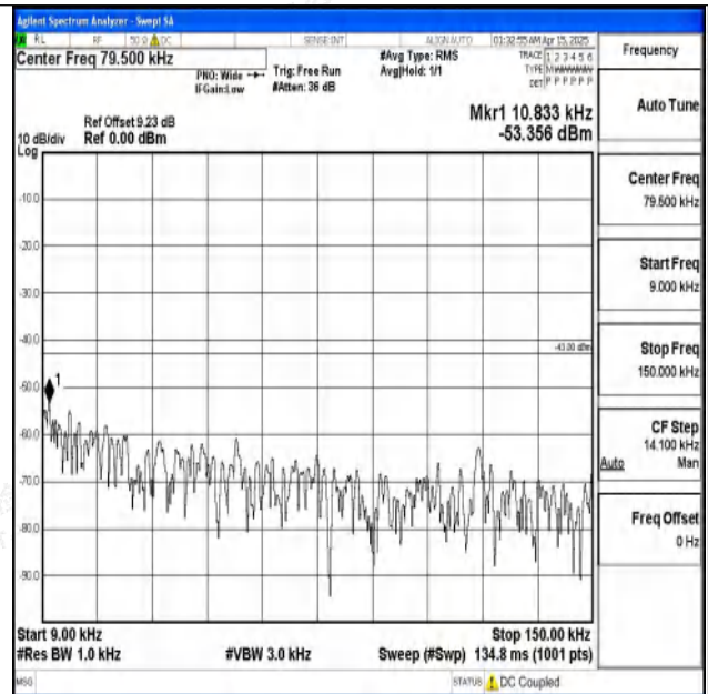
Band2-15MHz-16QAM-18675-1RB#0-0.009~0.15-PASS
