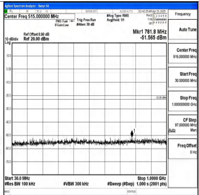
Band2-20MHz-16QAM-19100-1RB#0-30~1000-PASS
