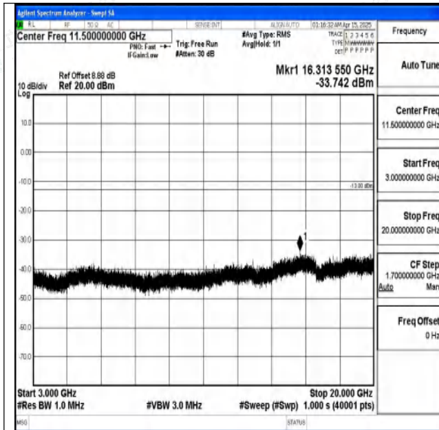
Band2-3MHz-QPSK-18900-1RB#0-3000~20000-PASS
