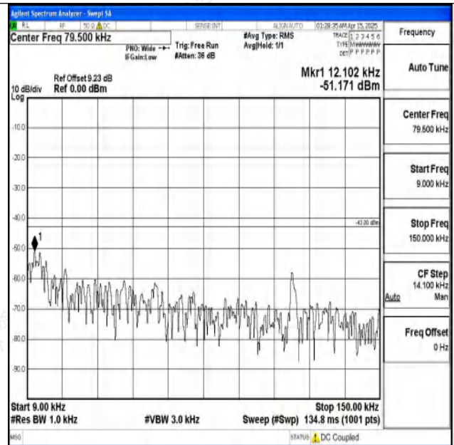
Band2-10MHz-16QAM-18900-1RB#0-0.009~0.15-PASS
