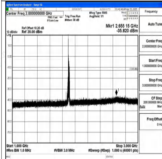
Band2-20MHz-16QAM-19100-1RB#0-1000~3000-PASS
