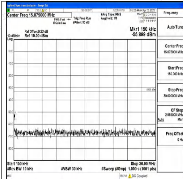
Band2-5MHz-16QAM-18900-1RB#0-0.15~30-PASS
