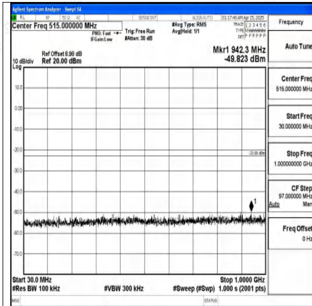
Band2-3MHz-QPSK-19185-1RB#0-30~1000-PASS
