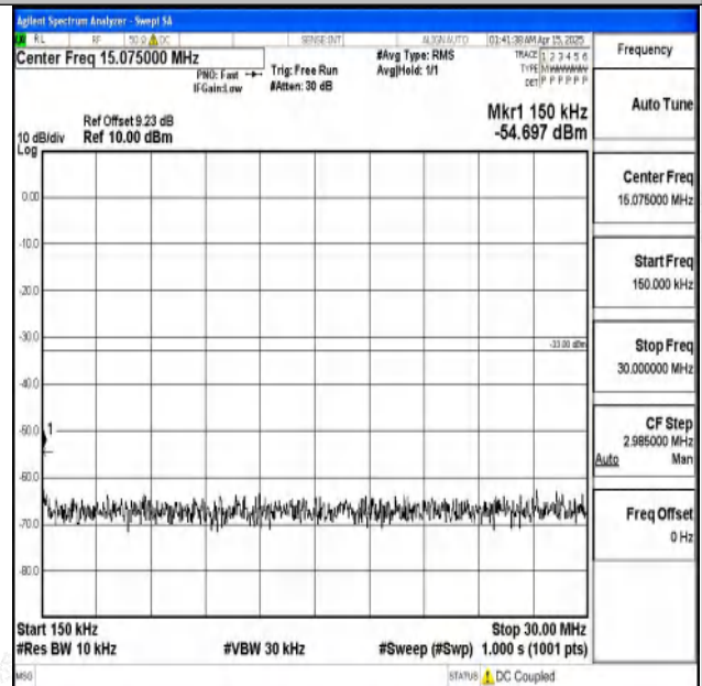
Band2-20MHz-QPSK-19100-1RB#0-0.15~30-PASS
