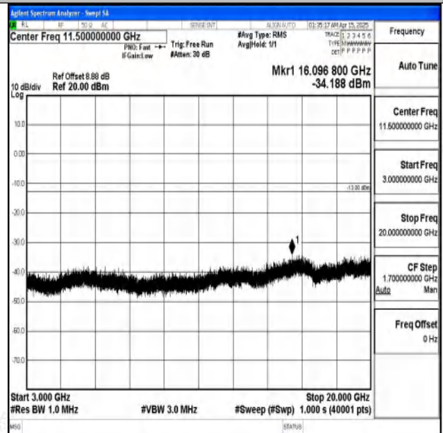
Band2-15MHz-16QAM-18900-1RB#0-3000~20000-PASS
