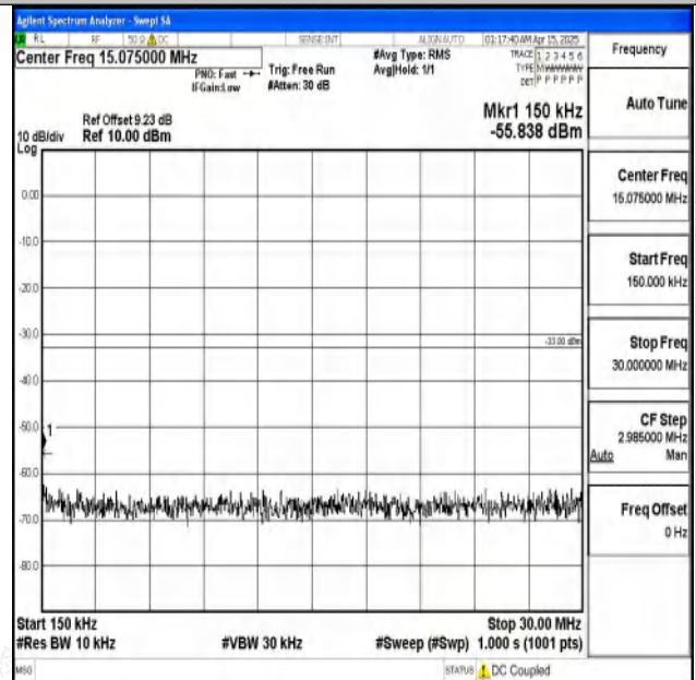
Band2-3MHz-QPSK-19185-1RB#0-0.15~30-PASS
