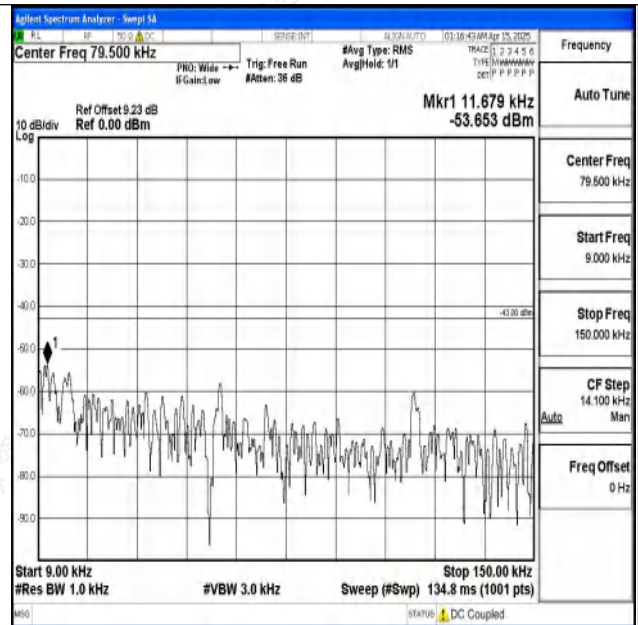
Band2-3MHz-16QAM-18900-1RB#0-0.009~0.15-PASS
