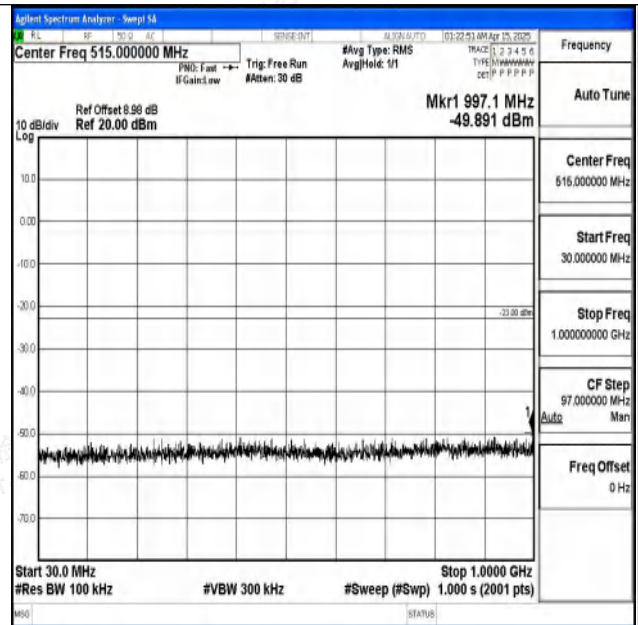
Band2-5MHz-16QAM-18900-1RB#0-30~1000-PASS
