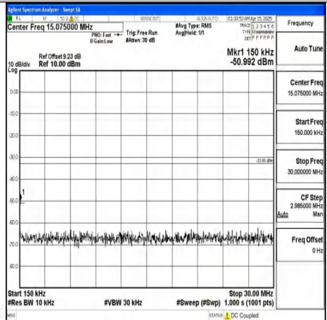
Band2-15MHz-QPSK-18900-1RB#0-0.15~30-PASS
