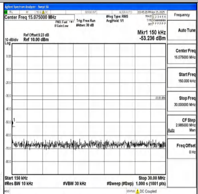
Band2-1.4MHz-QPSK-18900-1RB#0-0.15~30-PASS
