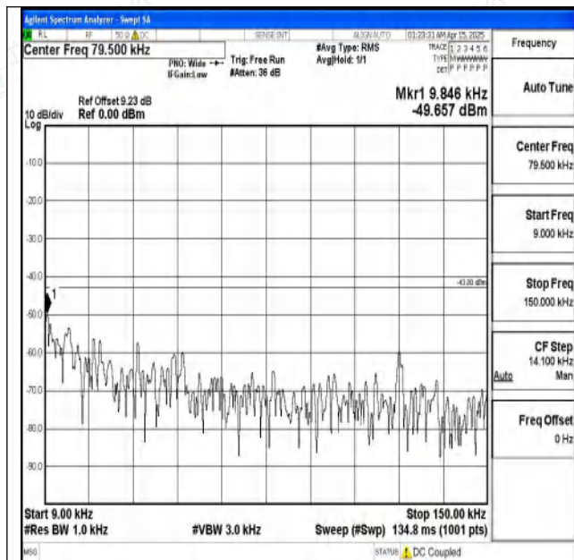
Band2-5MHz-QPSK-19175-1RB#0-0.009~0.15-PASS
