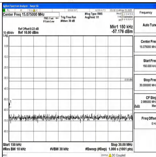
Band2-15MHz-QPSK-18675-1RB#0-0.15~30-PASS
