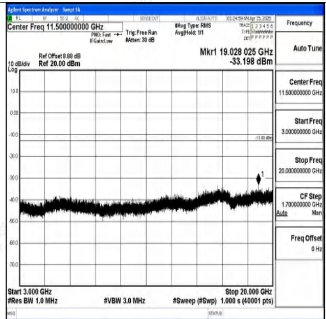
Band2-5MHz-16QAM-19175-1RB#0-3000~20000-PASS
