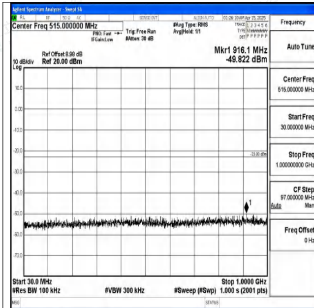
Band2-10MHz-QPSK-18650-1RB#0-30~1000-PASS
