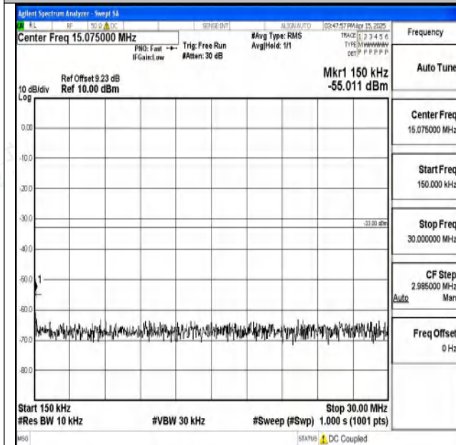
Band2-1.4MHz-16QAM-19193-1RB#0-0.15~30-PASS
