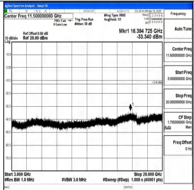
Band2-3MHz-16QAM-18615-1RB#0-3000~20000-PASS
