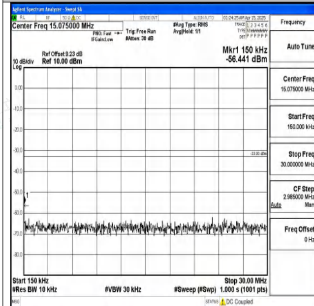
Band2-5MHz-16QAM-19175-1RB#0-0.15~30-PASS
