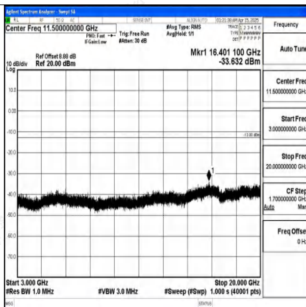
Band2-5MHz-16QAM-18625-1RB#0-3000~20000-PASS
