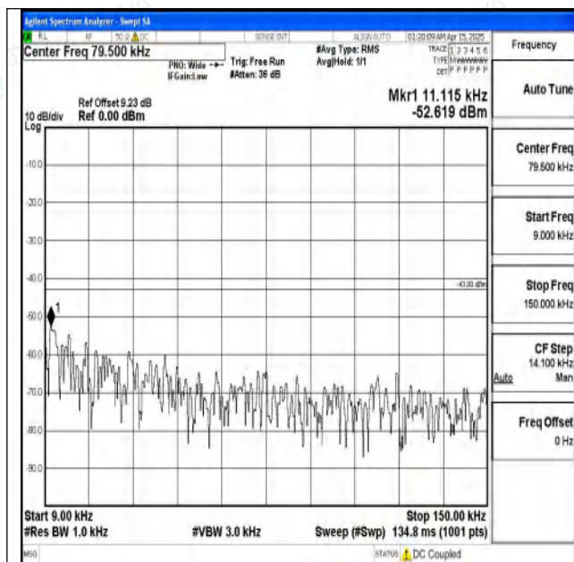
Band2-5MHz-QPSK-18625-1RB#0-0.009~0.15-PASS
