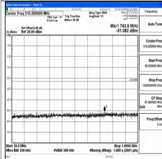
Band2-3MHz-QPSK-18615-1RB#0-30~1000-PASS
