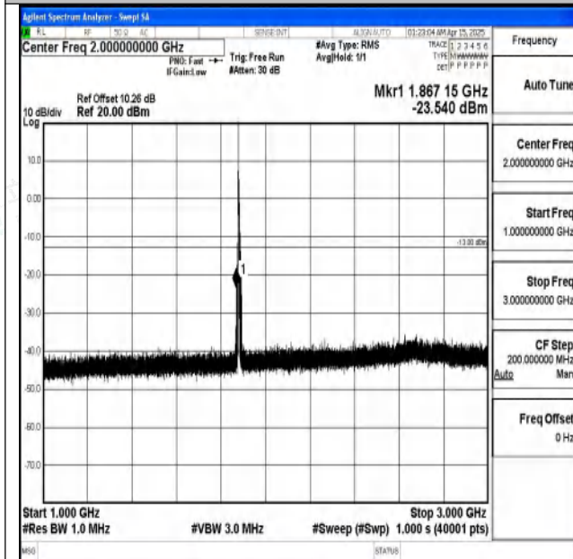
Band2-5MHz-16QAM-18900-1RB#0-1000~3000-PASS
