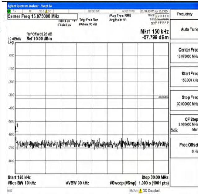
Band2-15MHz-16QAM-18900-1RB#0-0.15~30-PASS
