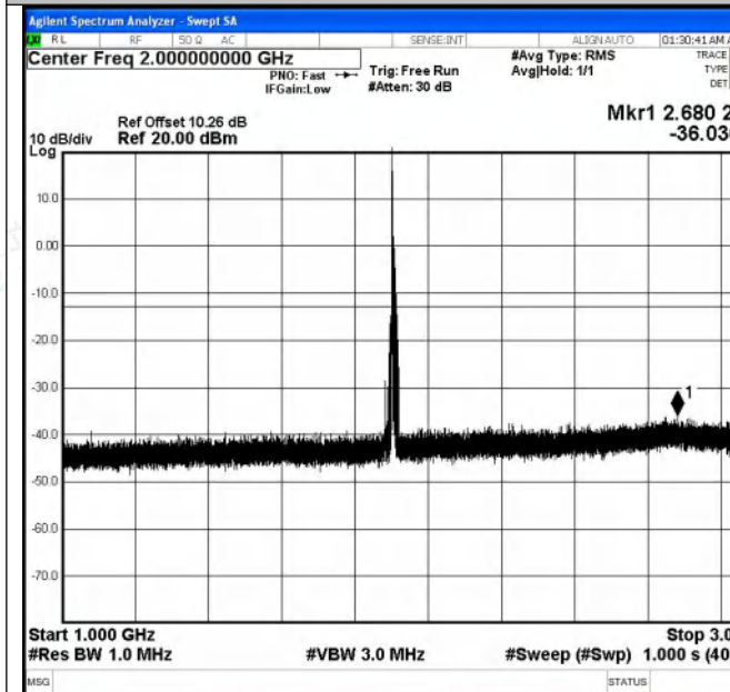
Band2-10MHz-16QAM-19150-1RB#0-1000~3000-PASS
