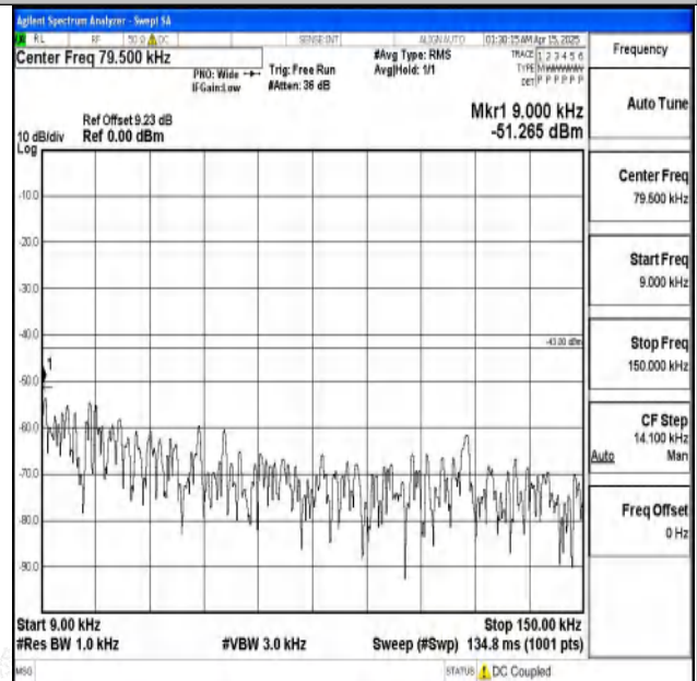
Band2-10MHz-16QAM-19150-1RB#0-0.009~0.15-PASS
