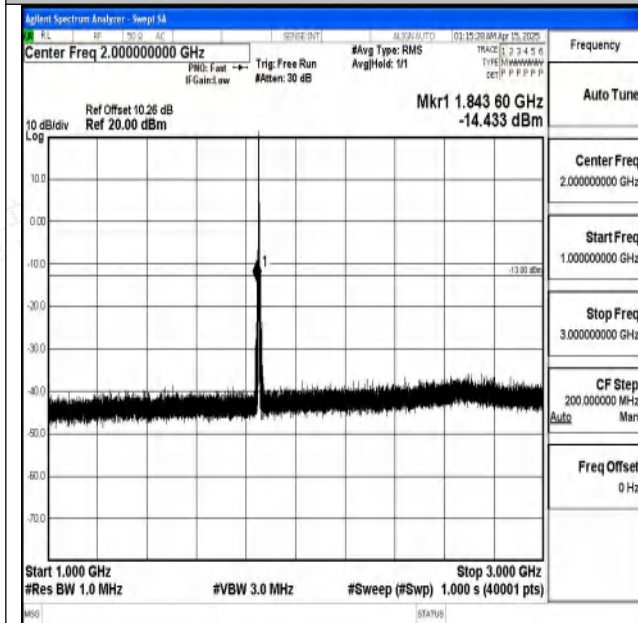
Band2-3MHz-16QAM-18615-1RB#0-1000~3000-PASS
