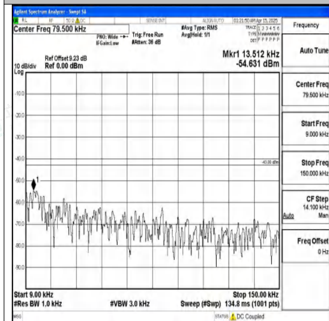
Band2-5MHz-QPSK-18900-1RB#0-0.009~0.15-PASS
