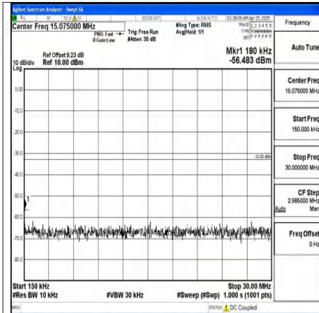
Band2-20MHz-16QAM-18700-1RB#0-0.15~30-PASS
