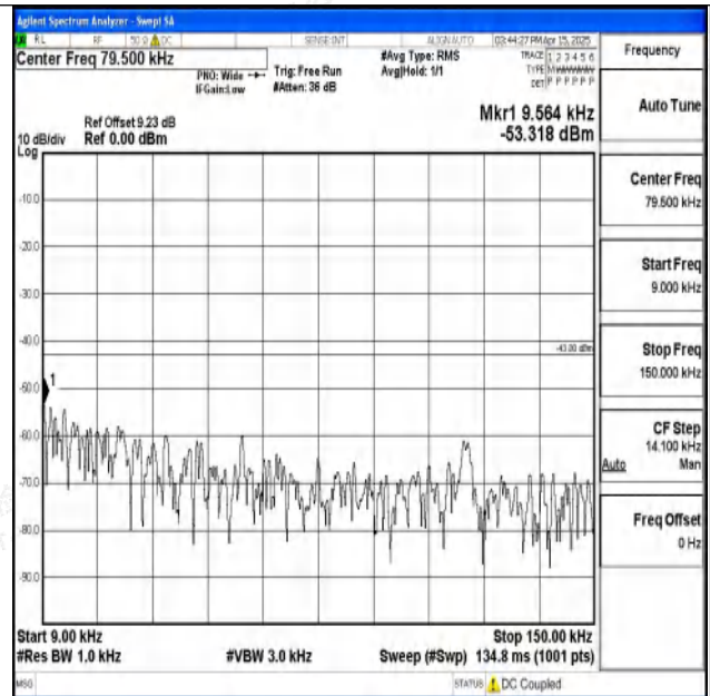
Band2-1.4MHz-16QAM-18607-1RB#0-0.009~0.15-PASS
