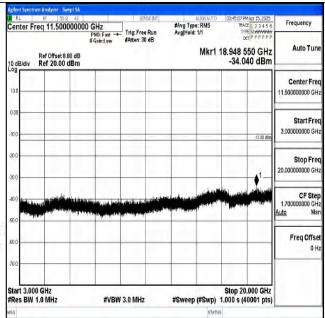
Band2-1.4MHz-16QAM-18607-1RB#0-3000~20000-PASS S
