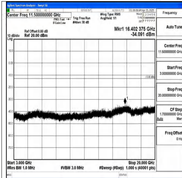
Band2-15MHz-QPSK-19125-1RB#0-3000~20000-PASS
