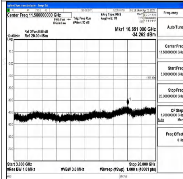
Band2-3MHz-QPSK-19185-1RB#0-3000~20000-PASS
