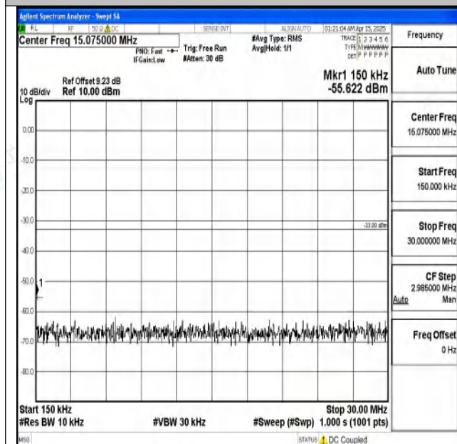
Band2-5MHz-16QAM-18625-1RB#0-0.15~30-PASS
