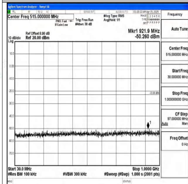
Band2-5MHz-QPSK-18625-1RB#0-30~1000-PASS
