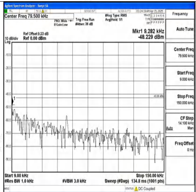
Band2-5MHz-16QAM-19175-1RB#0-0.009~0.15-PASS
