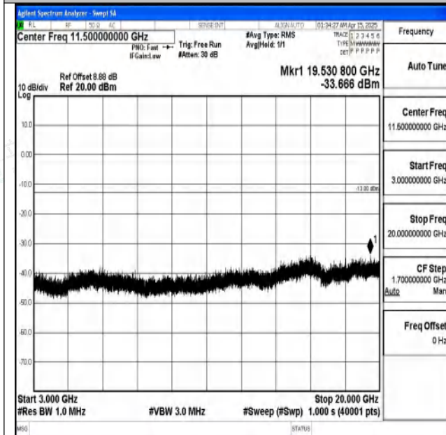
Band2-15MHz-QPSK-18900-1RB#0-3000~20000-PASS
