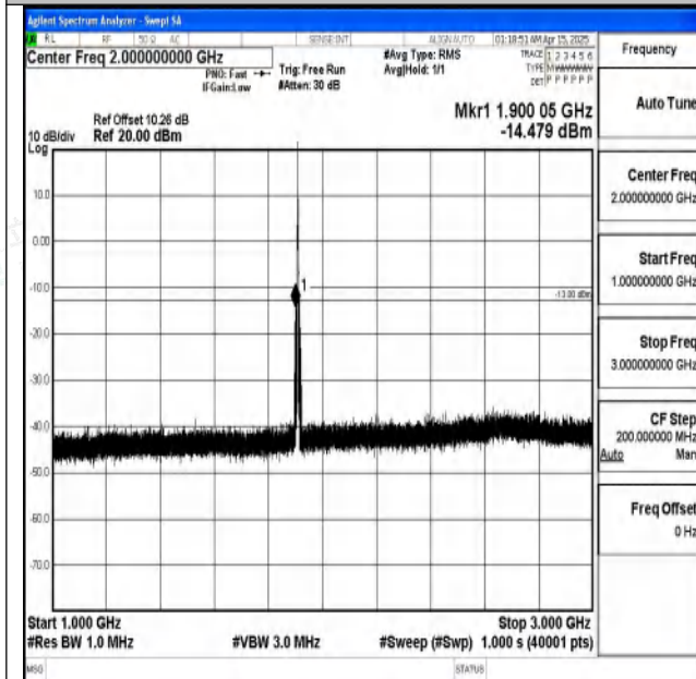
Band2-3MHz-16QAM-19185-1RB#0-1000~3000-PASS
