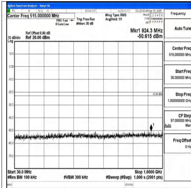
Band2-5MHz-QPSK-18900-1RB#0-30~1000-PASS
