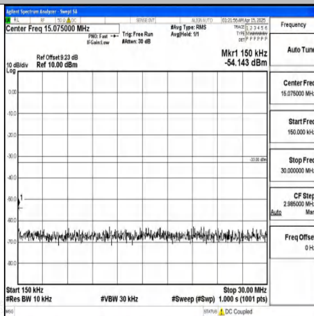
Band2-5MHz-QPSK-18900-1RB#0-0.15~30-PASS
