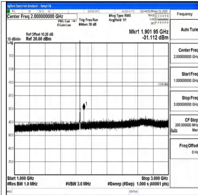
Band2-1.4MHz-16QAM-18607-1RB#0-1000~3000-PASS
