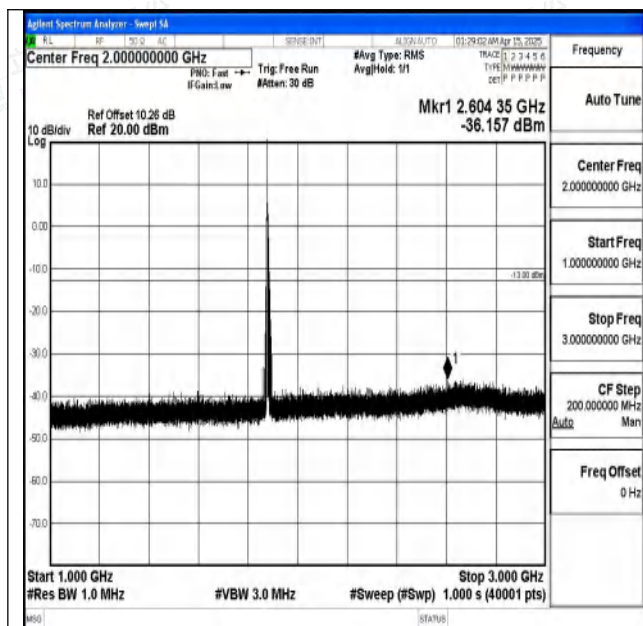
Band2-10MHz-16QAM-18900-1RB#0-1000~3000-PASS
