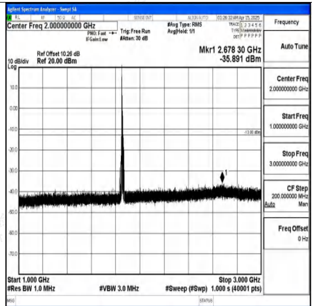
Band2-10MHz-QPSK-18650-1RB#0-1000~3000-PASS
