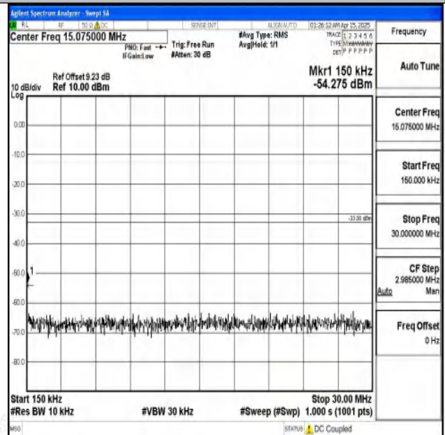
Band2-10MHz-QPSK-18650-1RB#0-0.15~30-PASS
