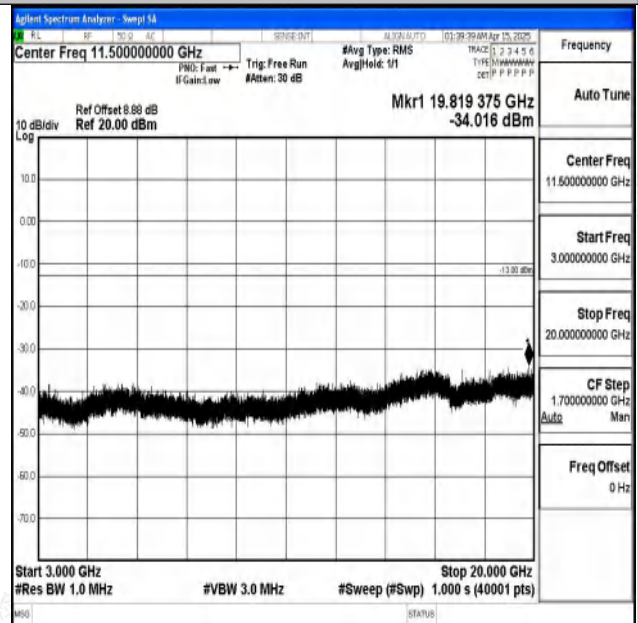
Band2-20MHz-16QAM-18700-1RB#0-3000~20000-PASS
