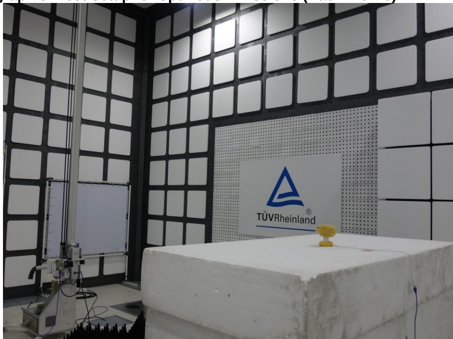
Photograph 8: Test Setup for Spurious Emissions (Back View 5)
