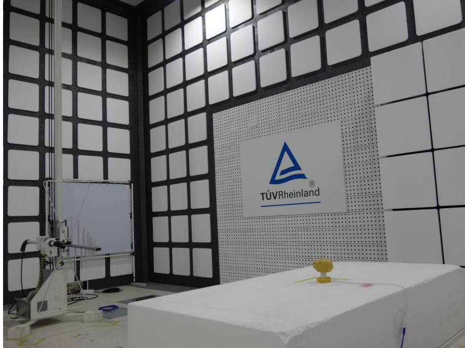
Photograph 5: Test Setup for Spurious Emissions (Back View 2)
