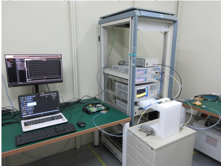
Photograph 13: Test Setup for DFS Mode (WiFi 5GHz)
