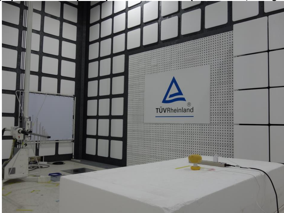
Photograph 6: Test Setup for Spurious Emissions (Back View 3, Charge Mode)
